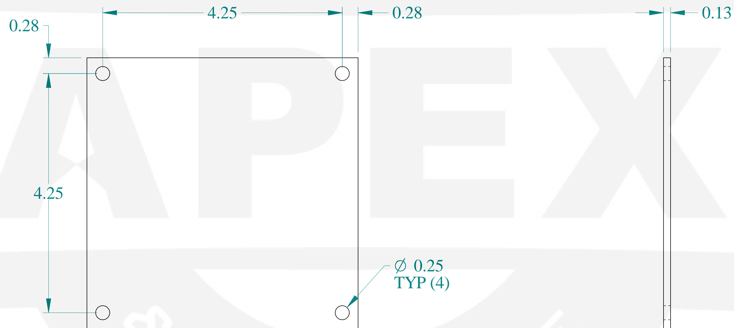
FRONT VIEW
