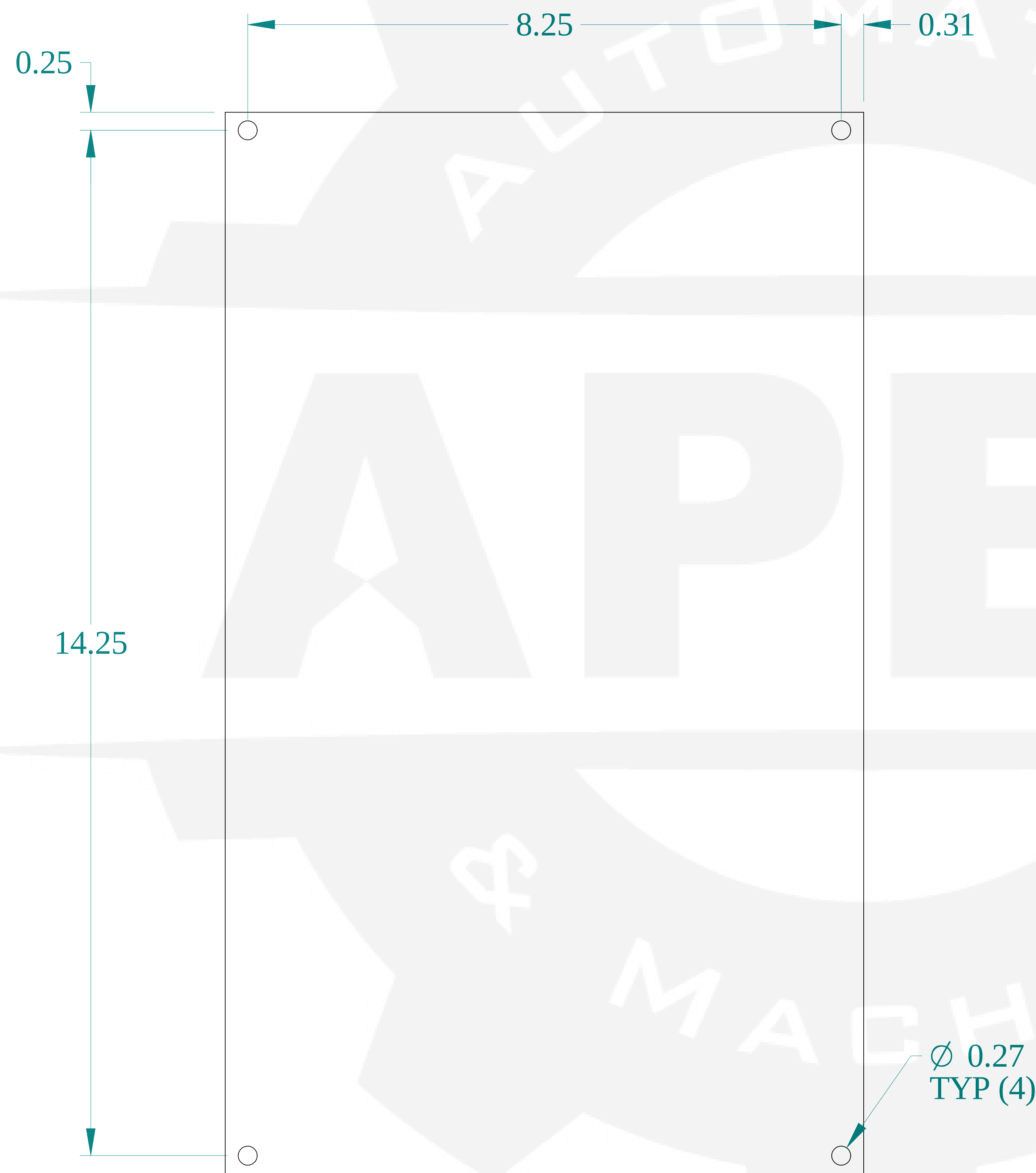
FRONT VIEW
