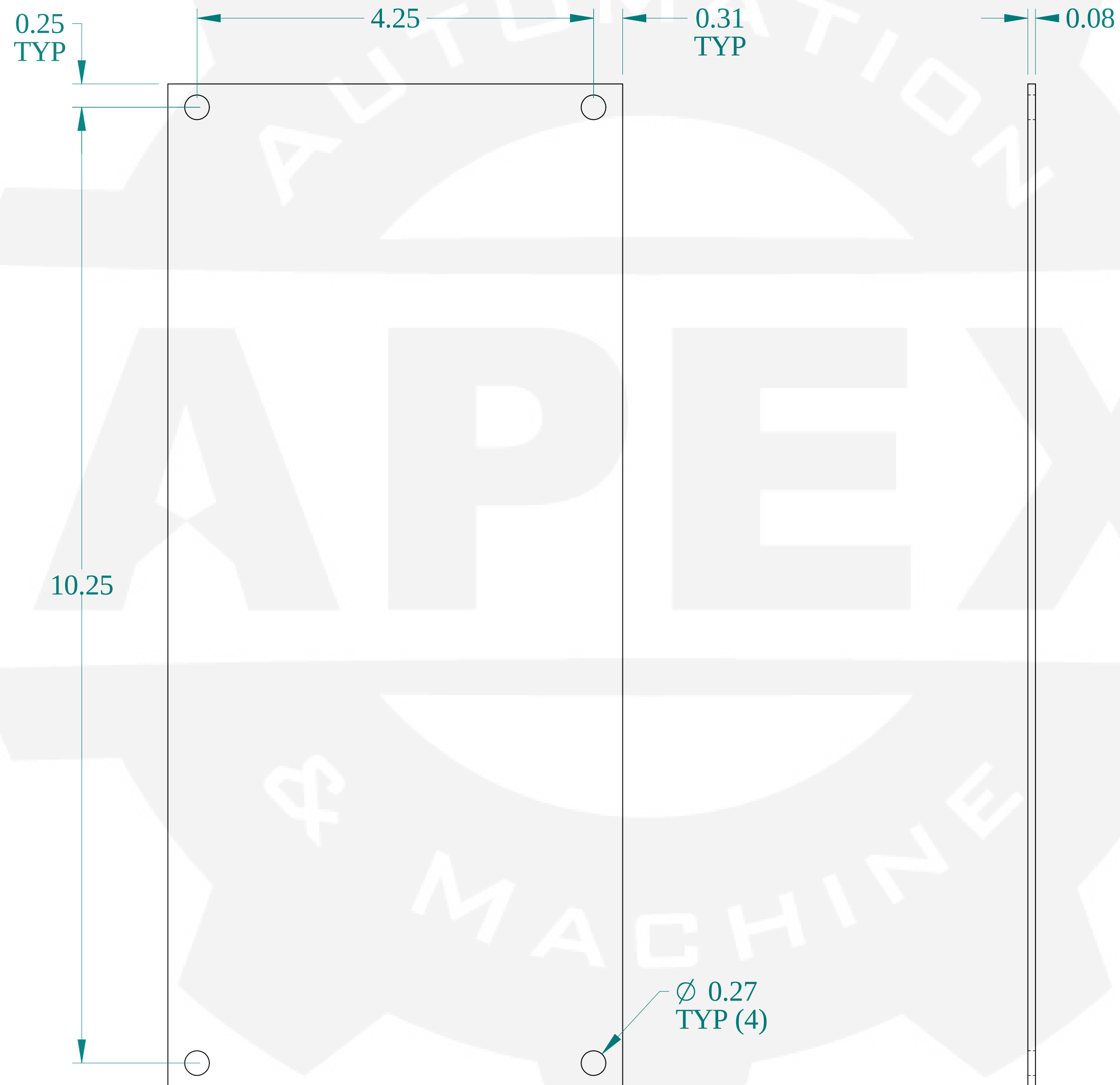
FRONT VIEW
