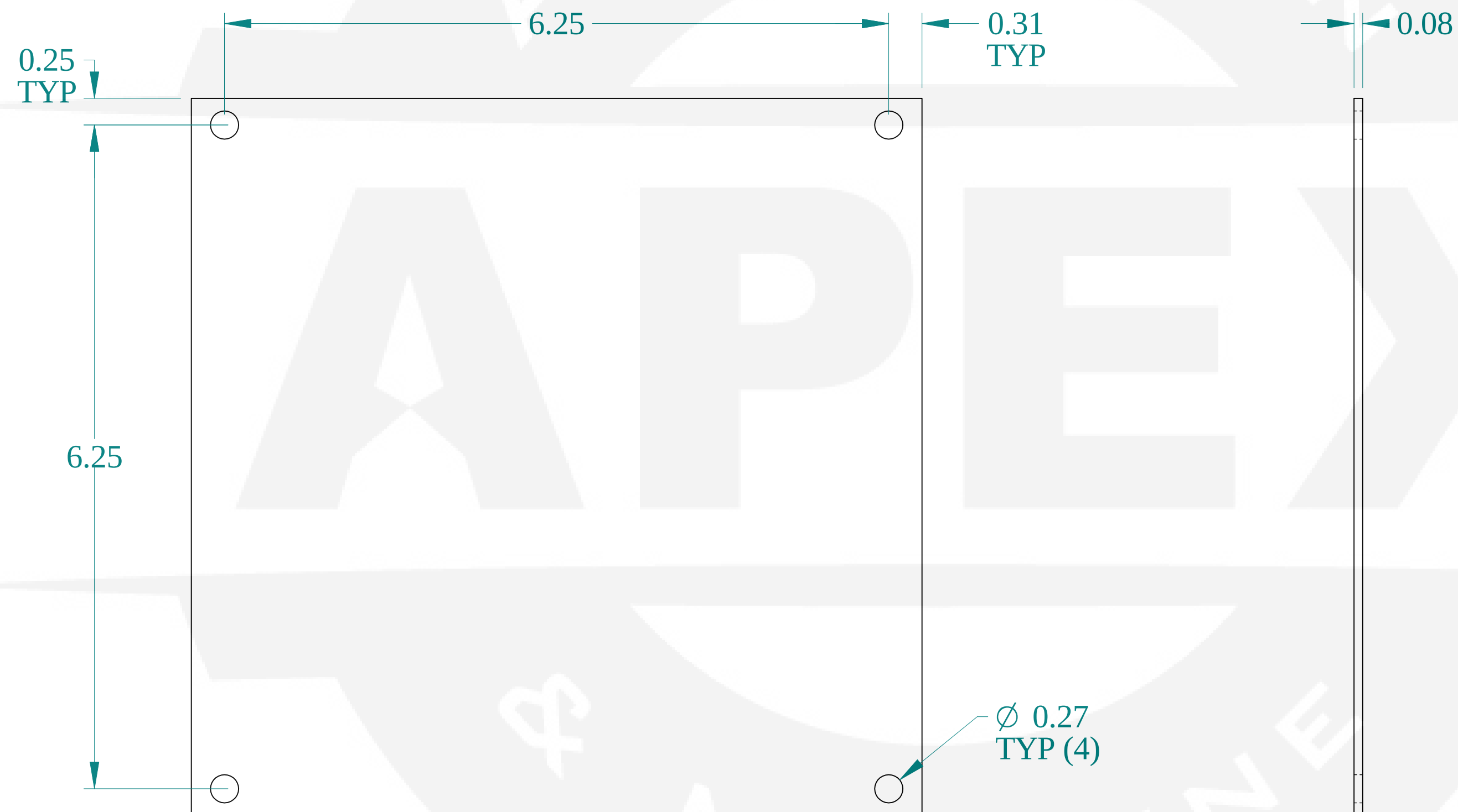
FRONT VIEW
