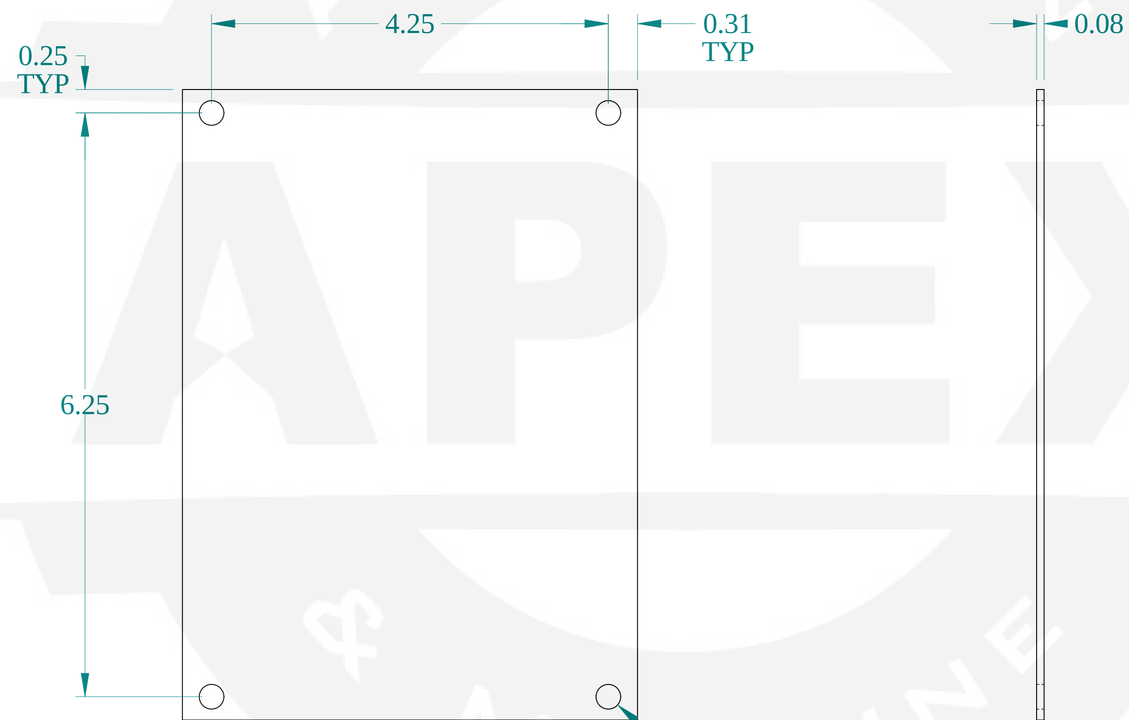
FRONT VIEW
