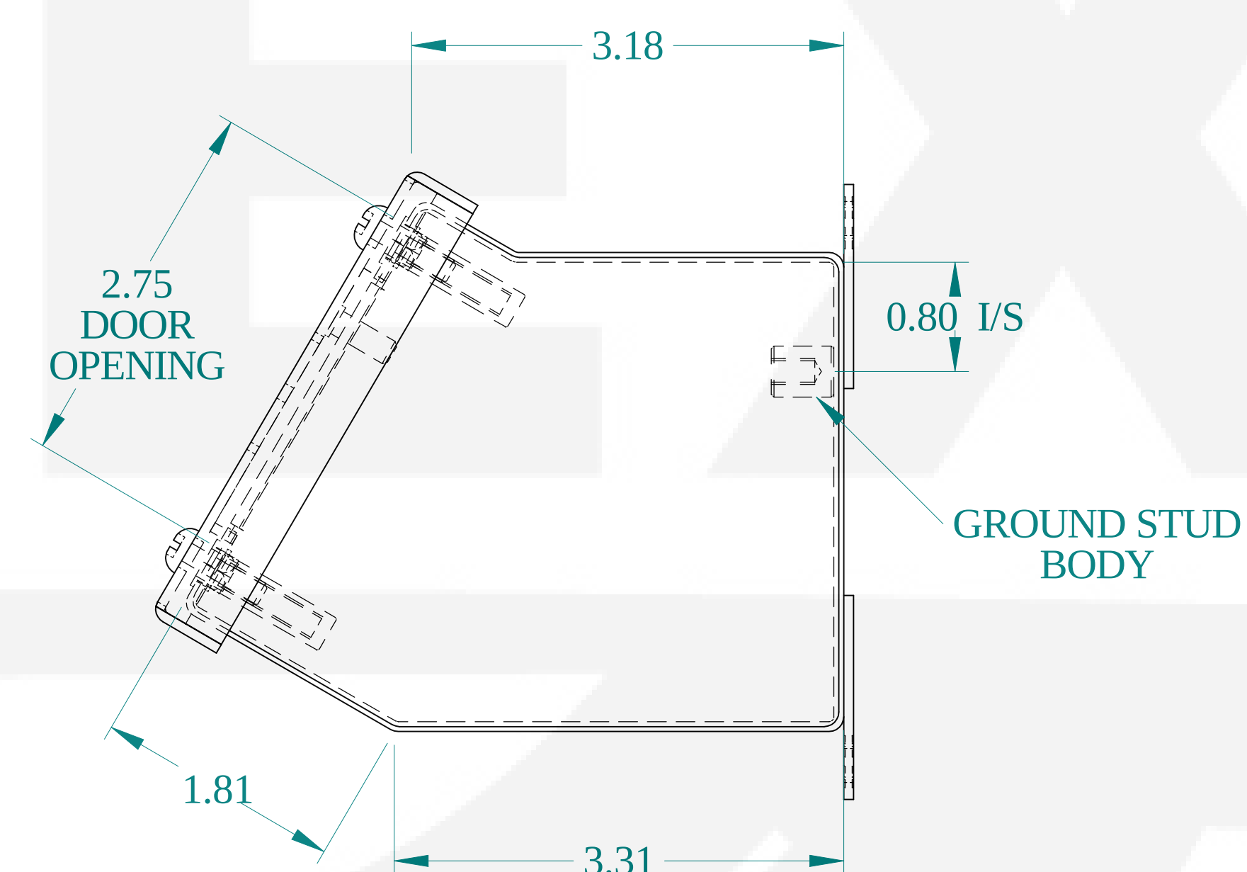
SIDE VIEW
