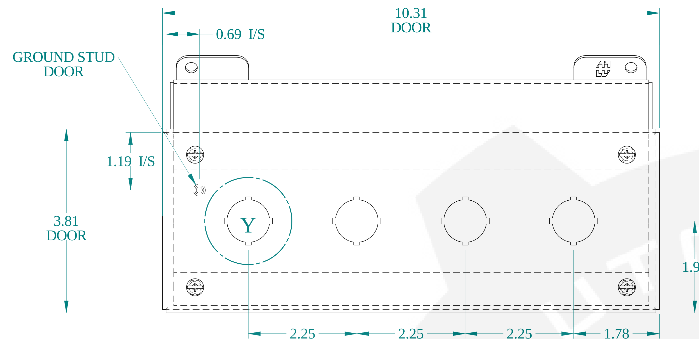
VIEW Z-Z
