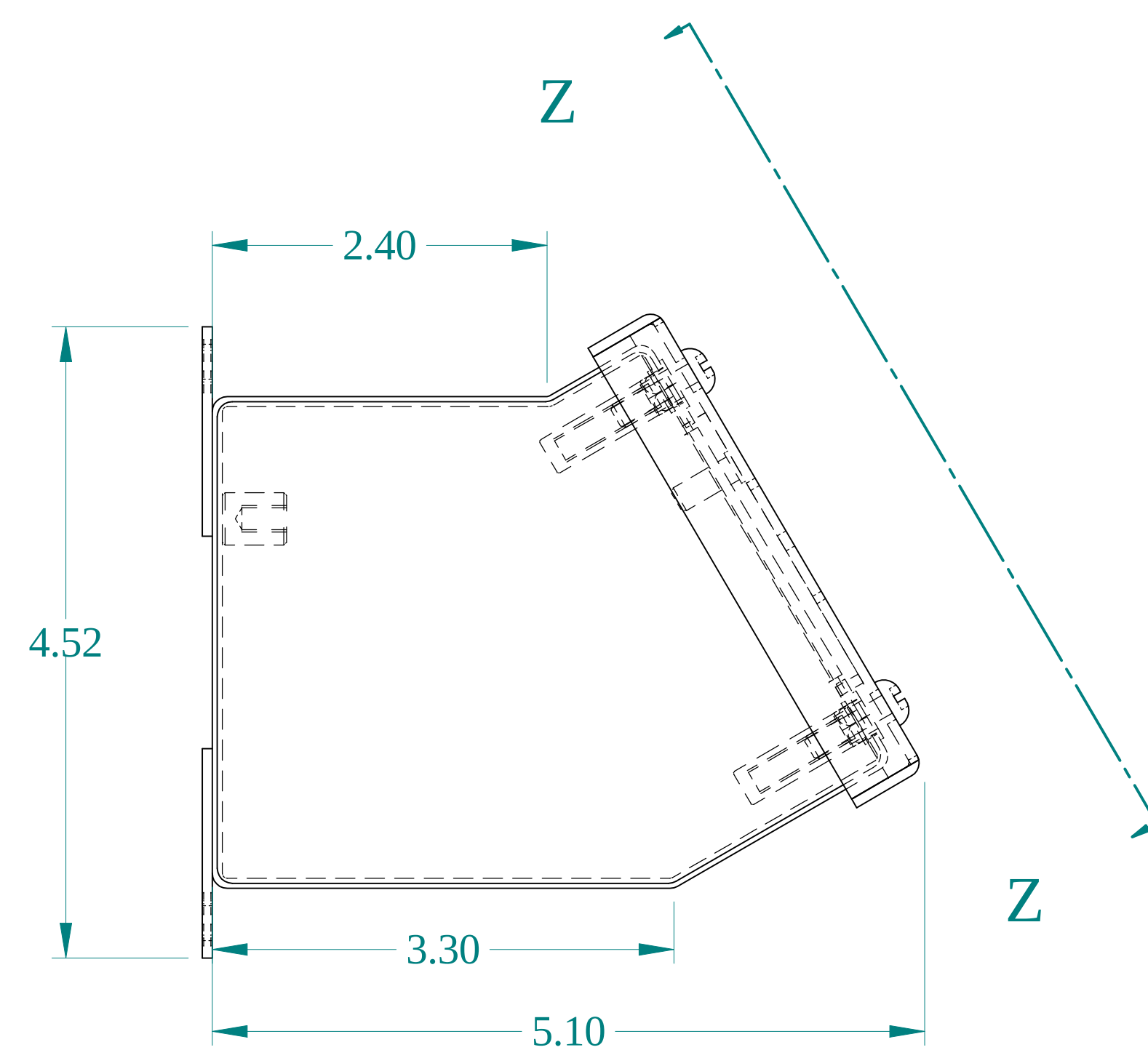
SIDE VIEW
