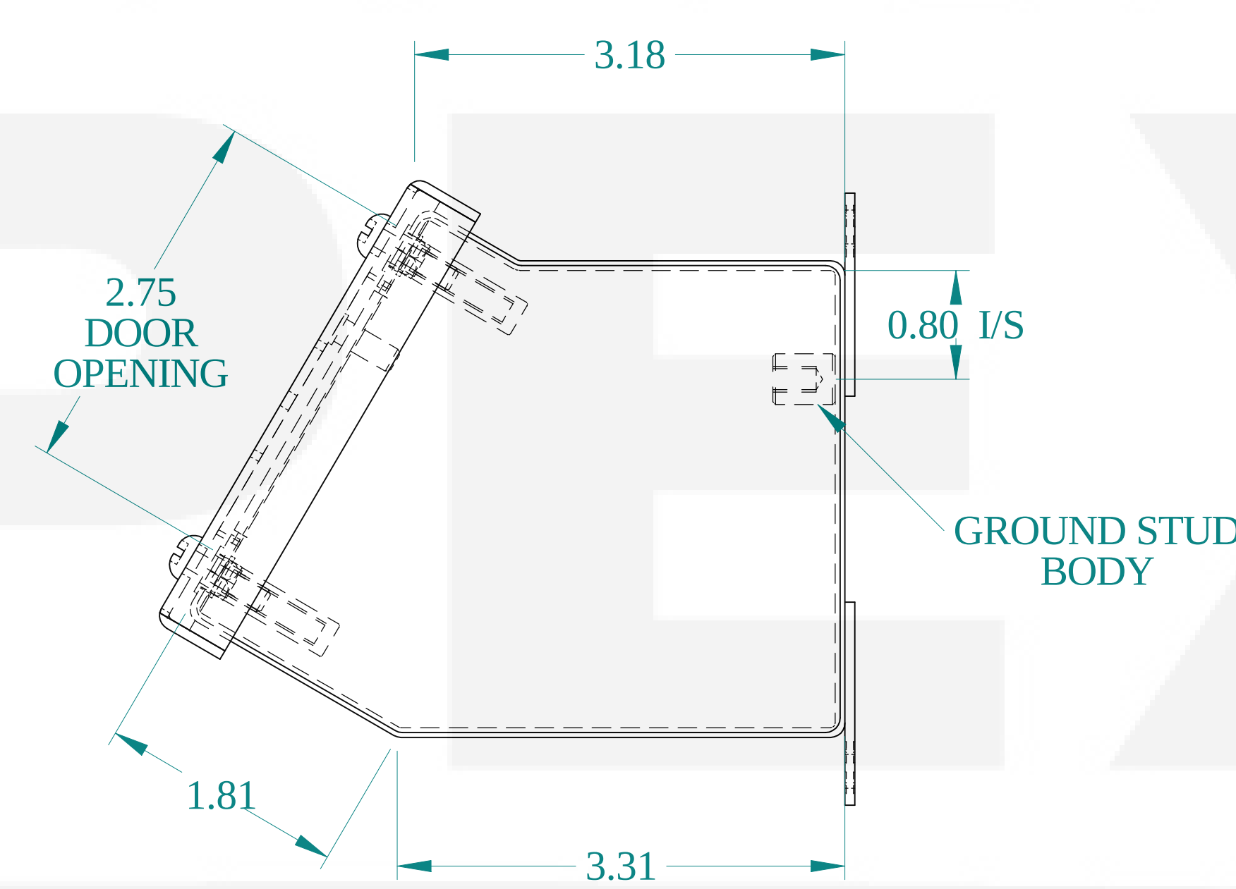
SIDE VIEW
