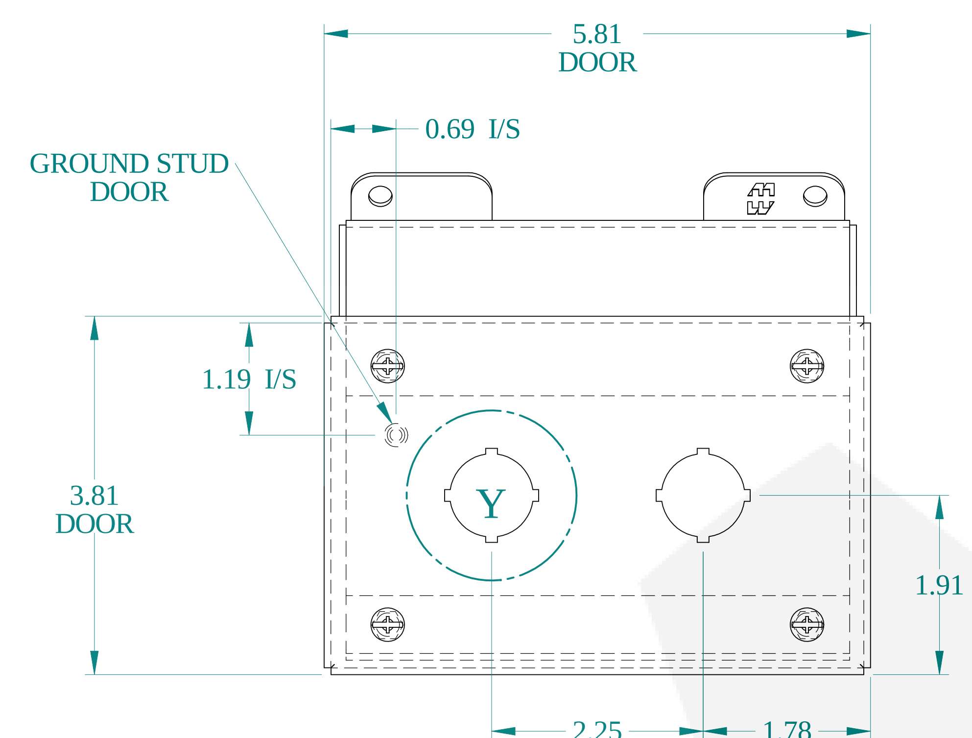
VIEW Z-Z
