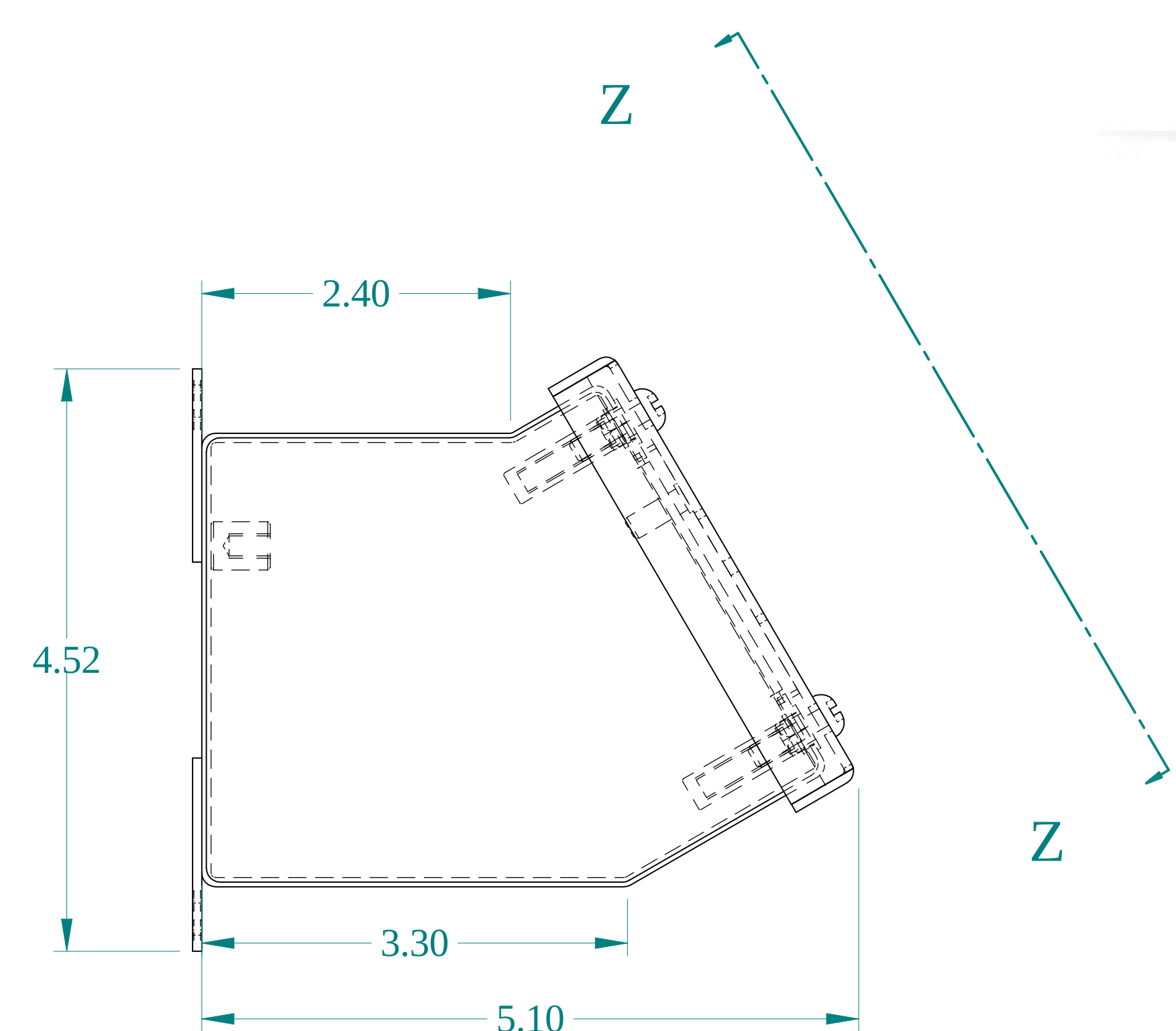
SIDE VIEW
