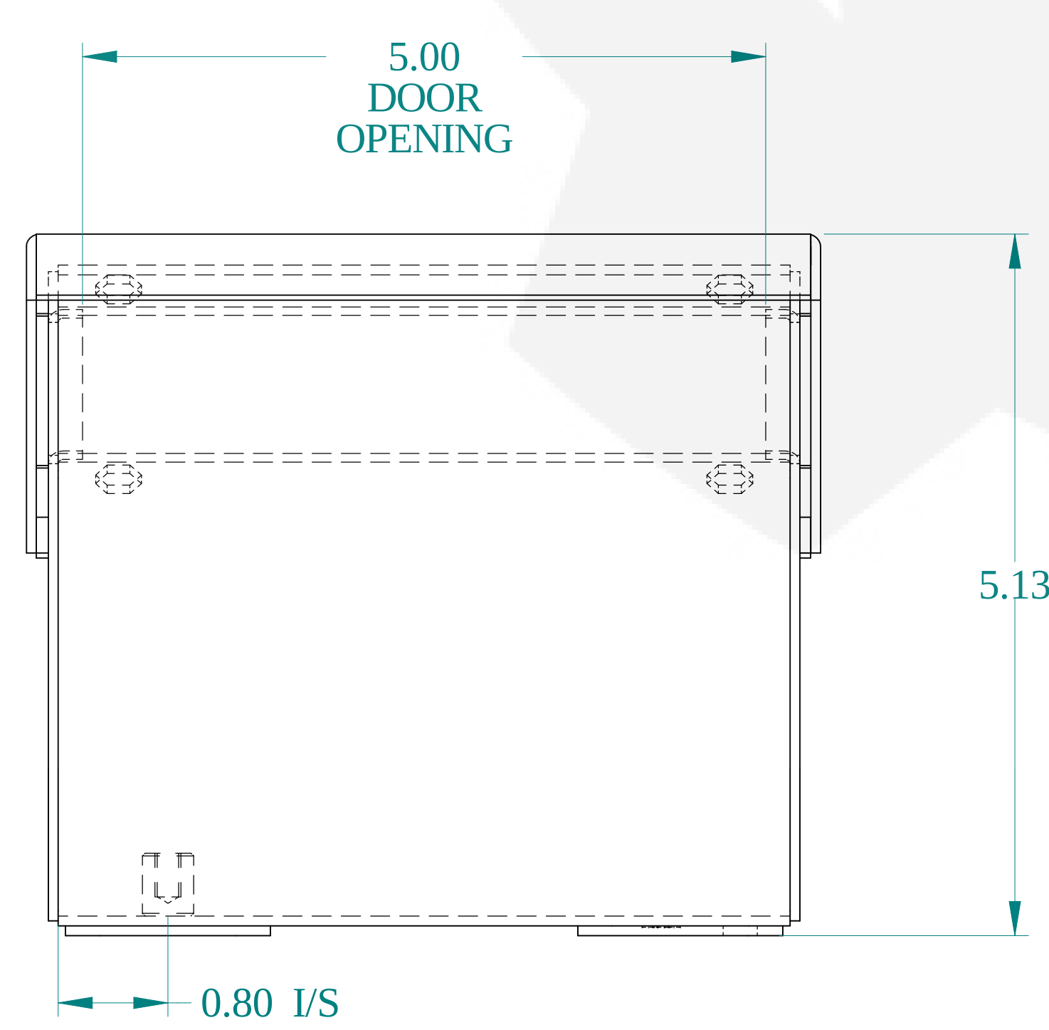
BOTTOM VIEW
