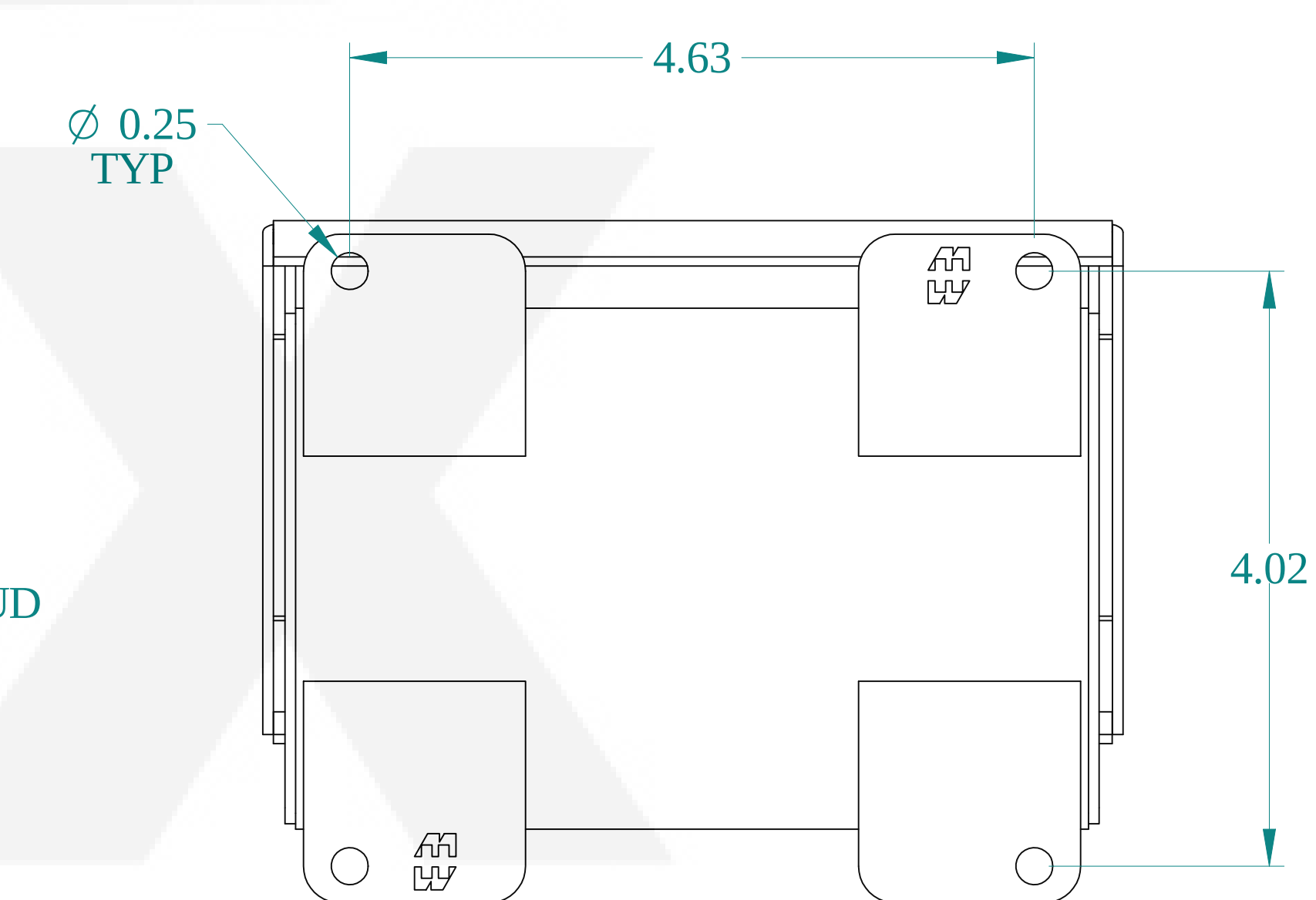
BACK VIEW
