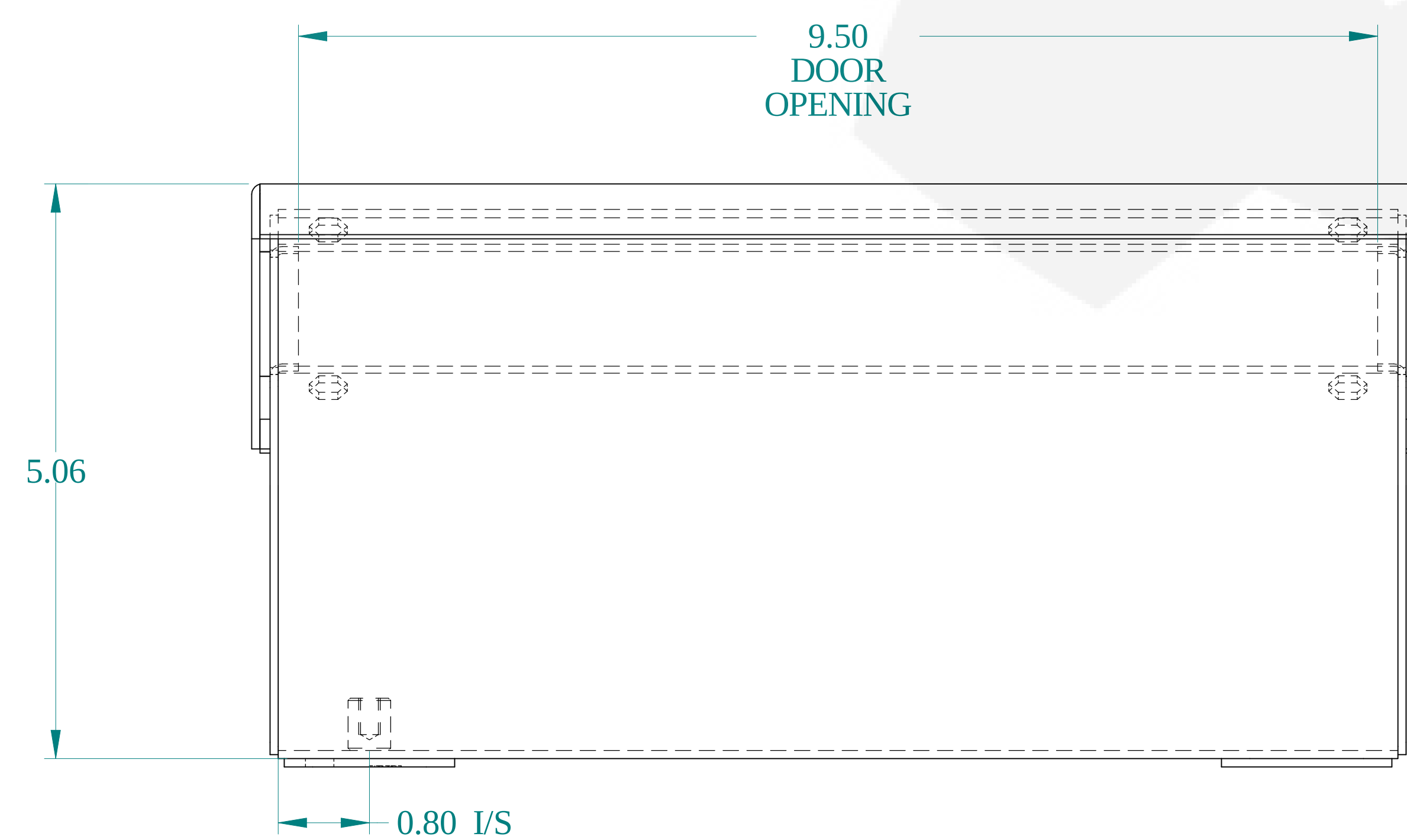
BOTTOM VIEW
