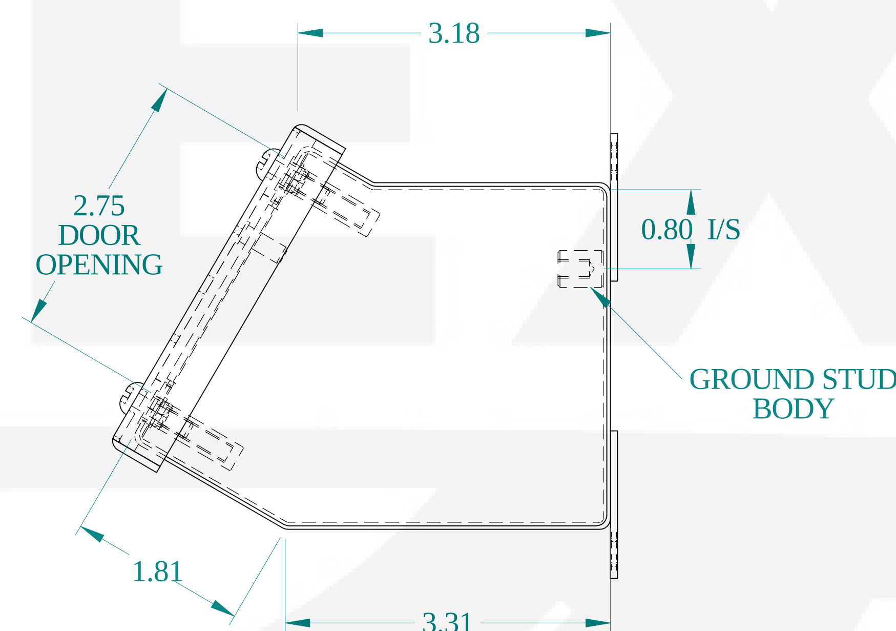
SIDE VIEW
