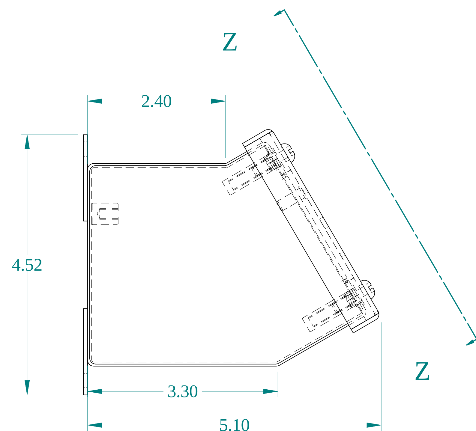
SIDE VIEW
