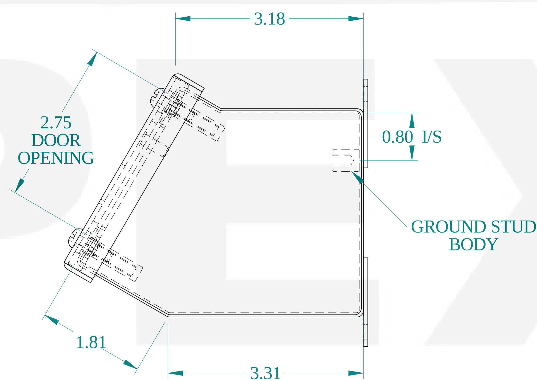
SIDE VIEW
