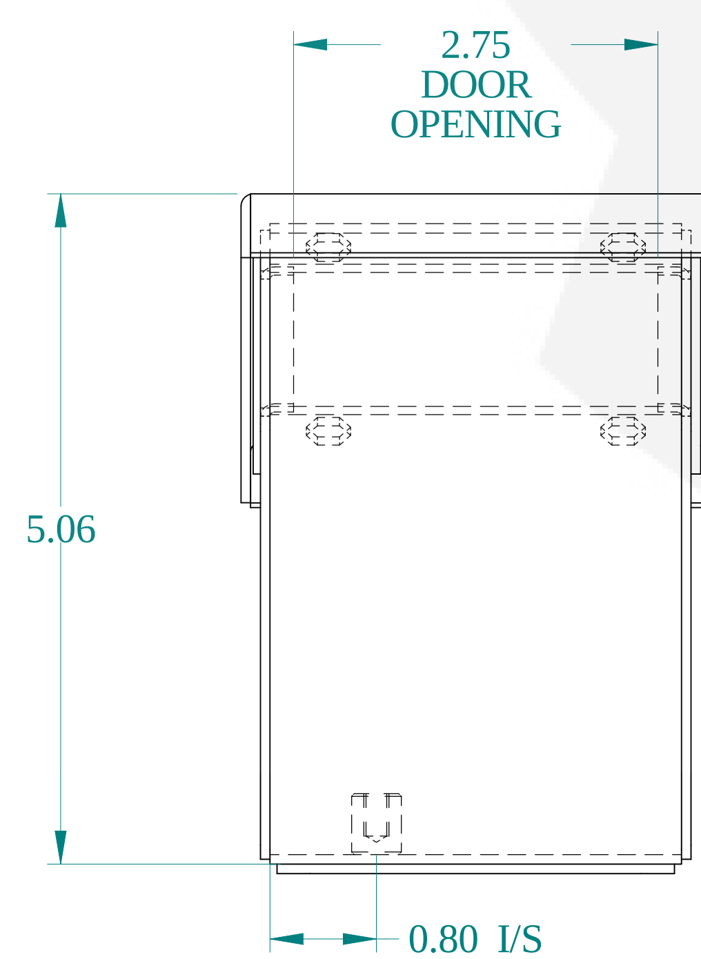
BOTTOM VIEW
