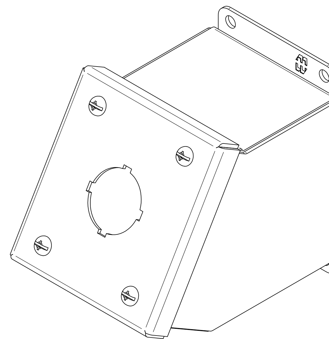
ISOMETRIC VIEWS
