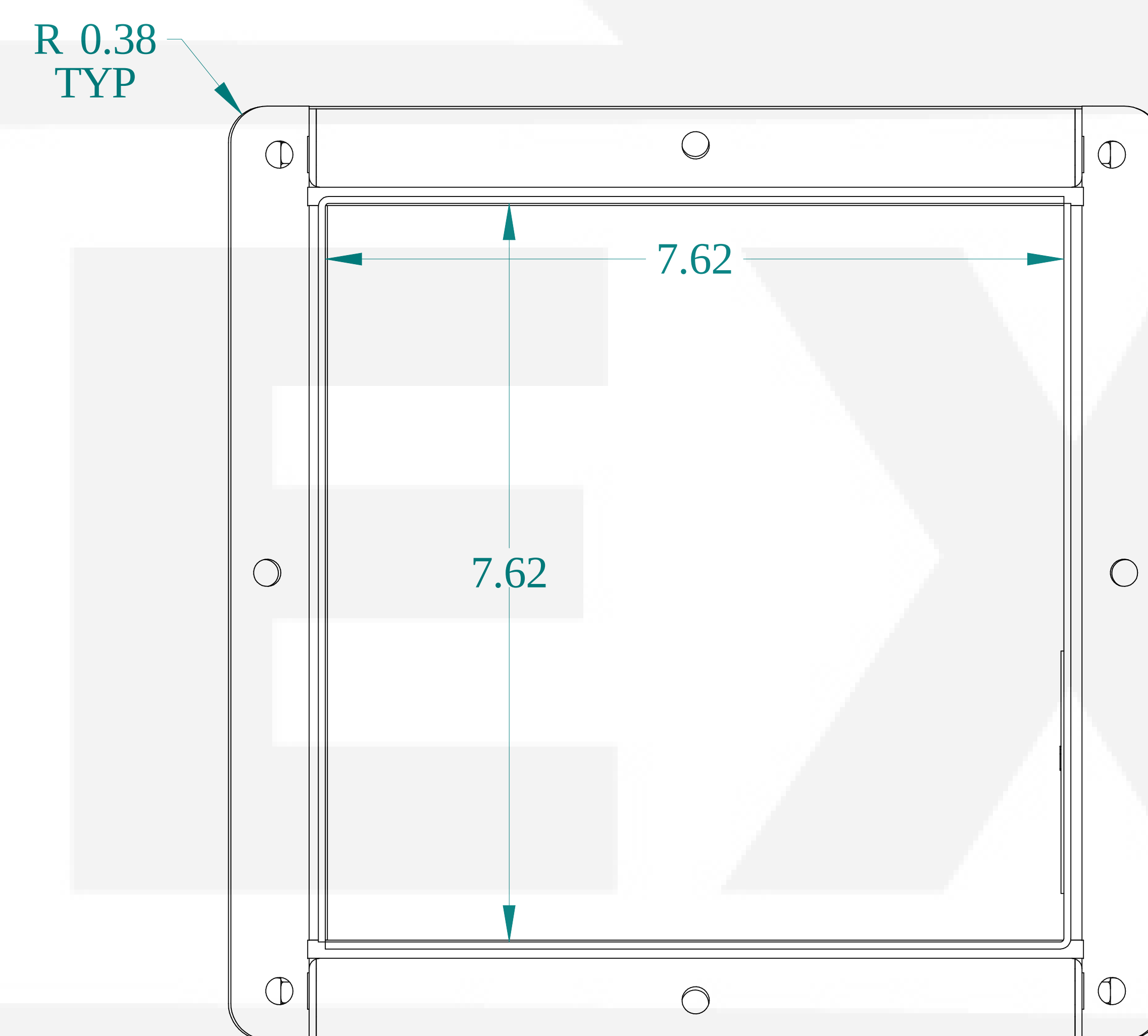
SIDE VIEW
