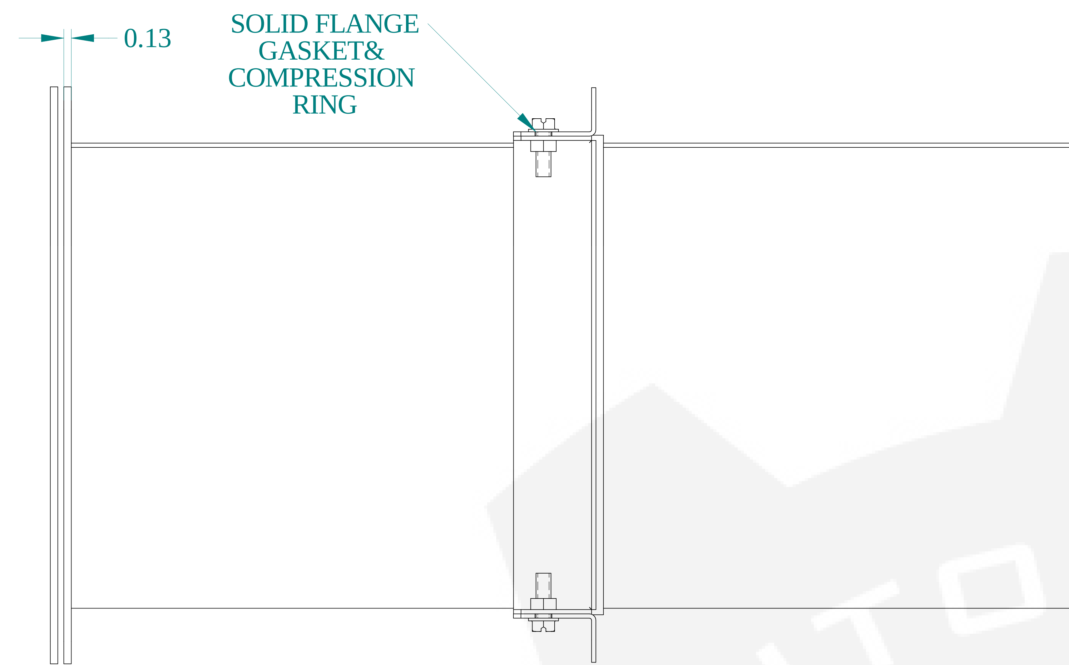
TOP VIEW
