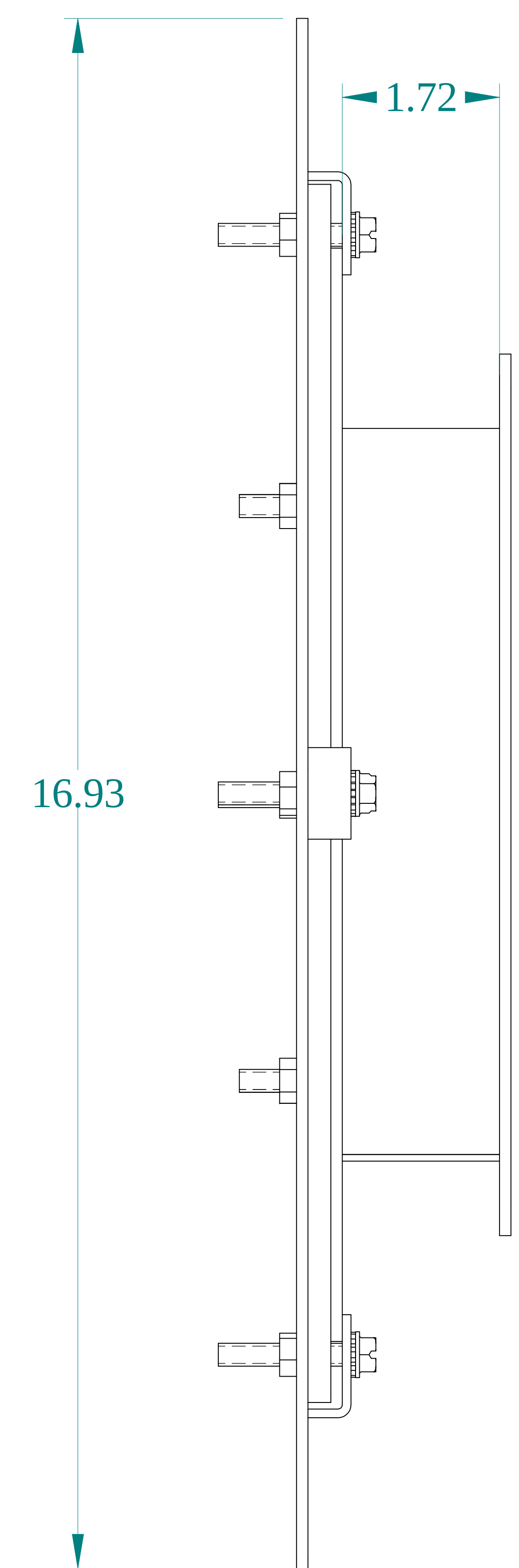
SIDE VIEW
