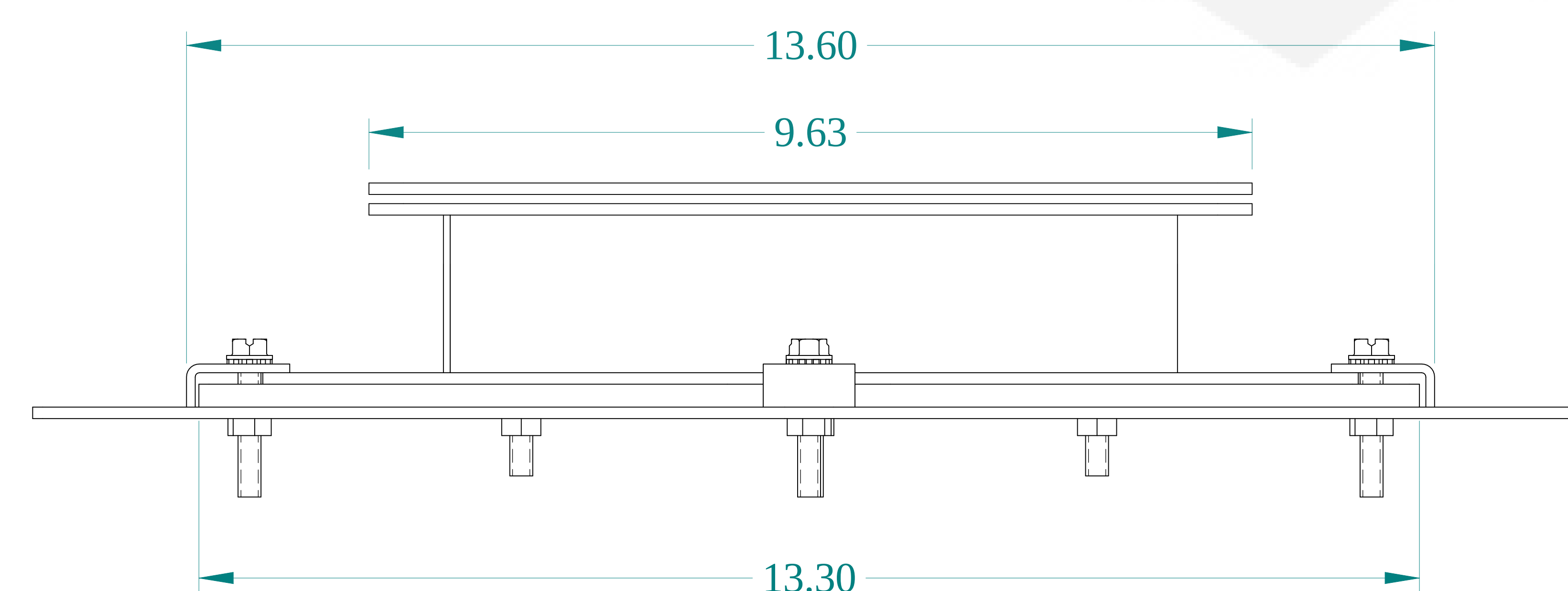
BOTTOM VIEW
