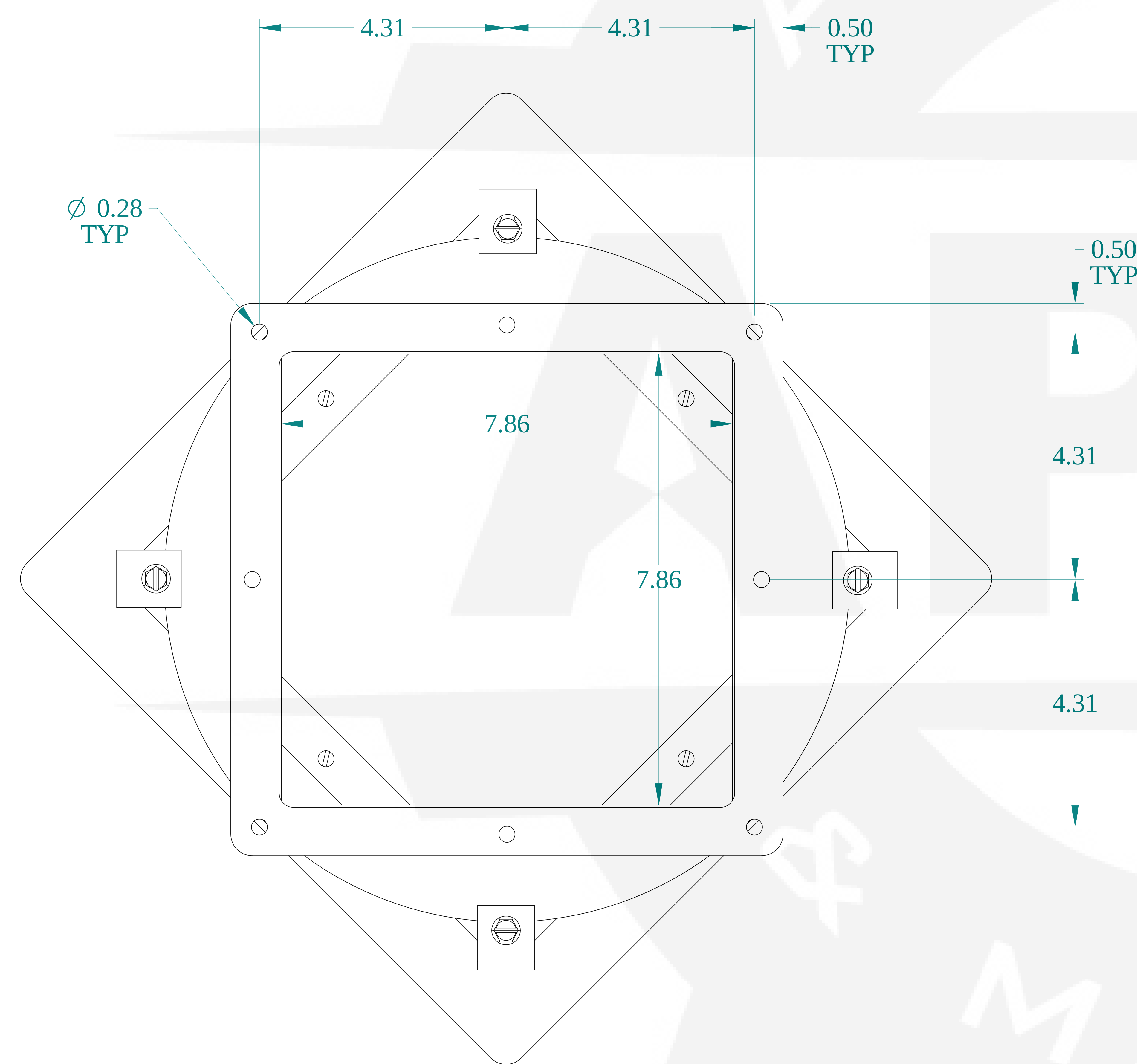
FRONT VIEW
