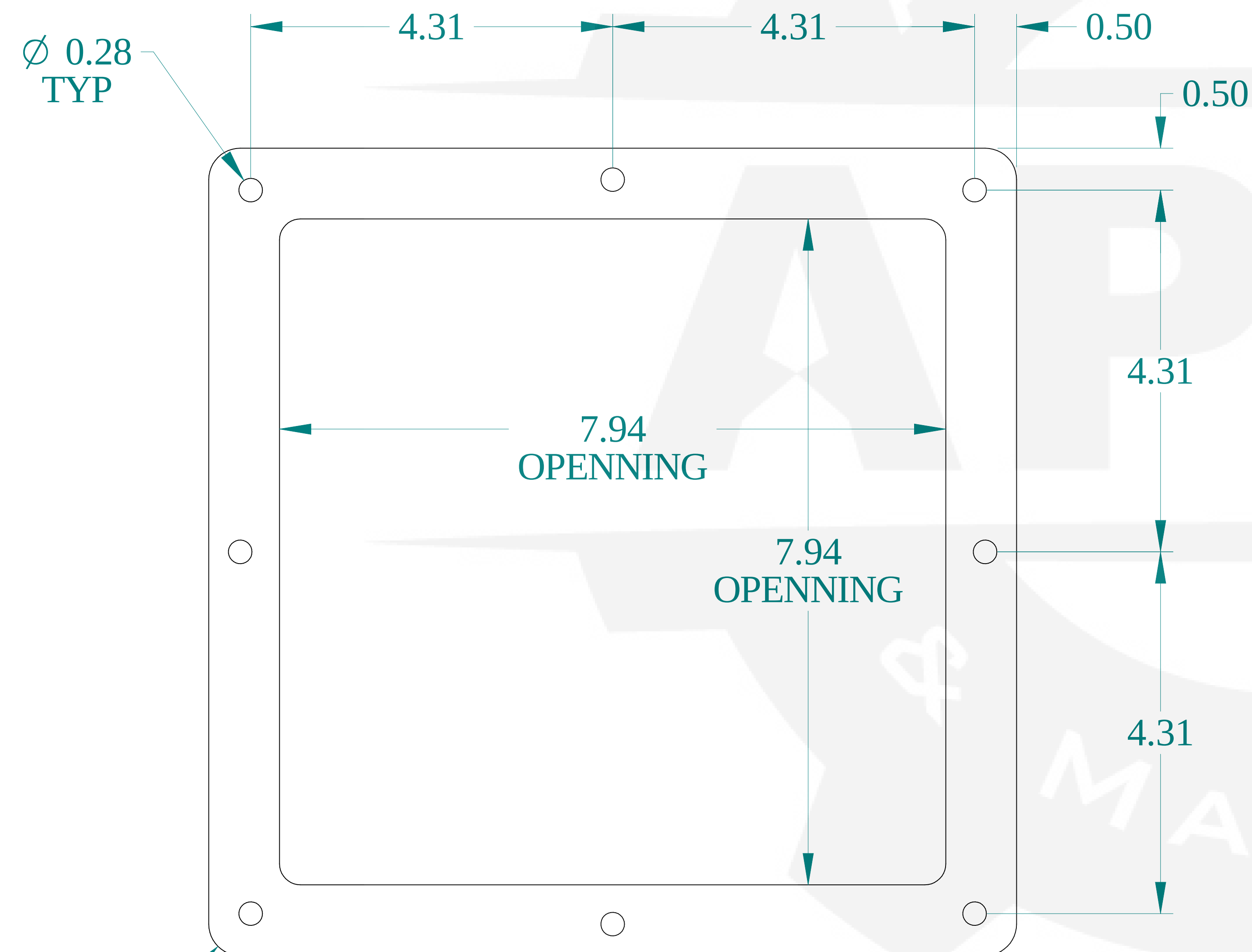
FRONT VIEW
