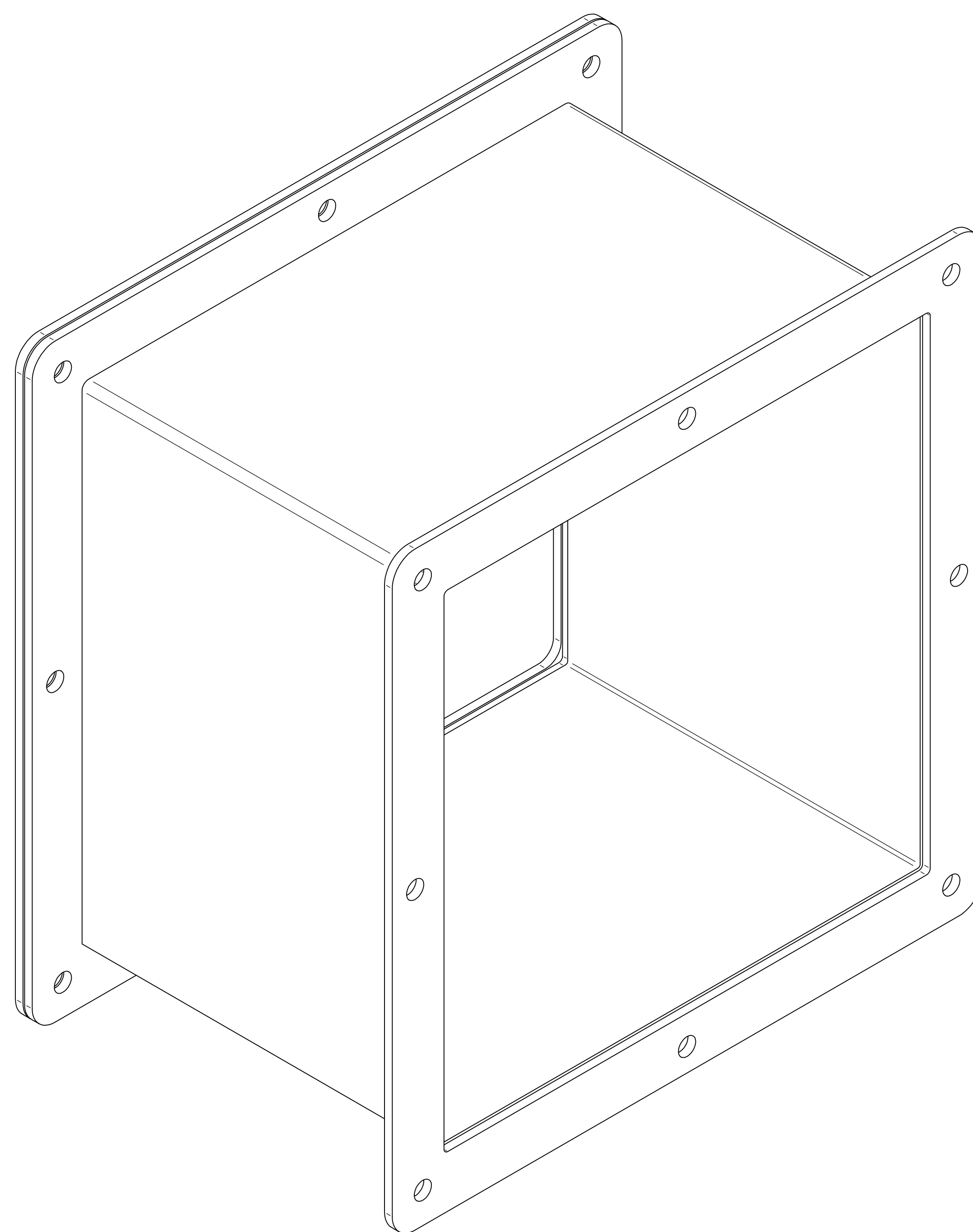
ISOMETRIC VIEWS
