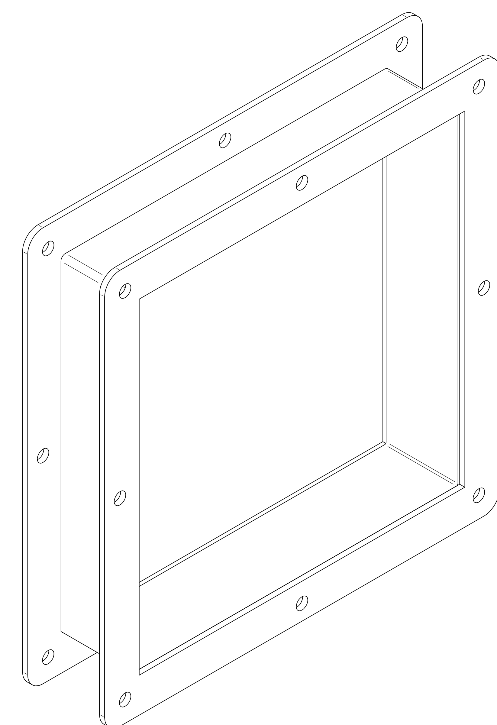
ISOMETRIC VIEWS
