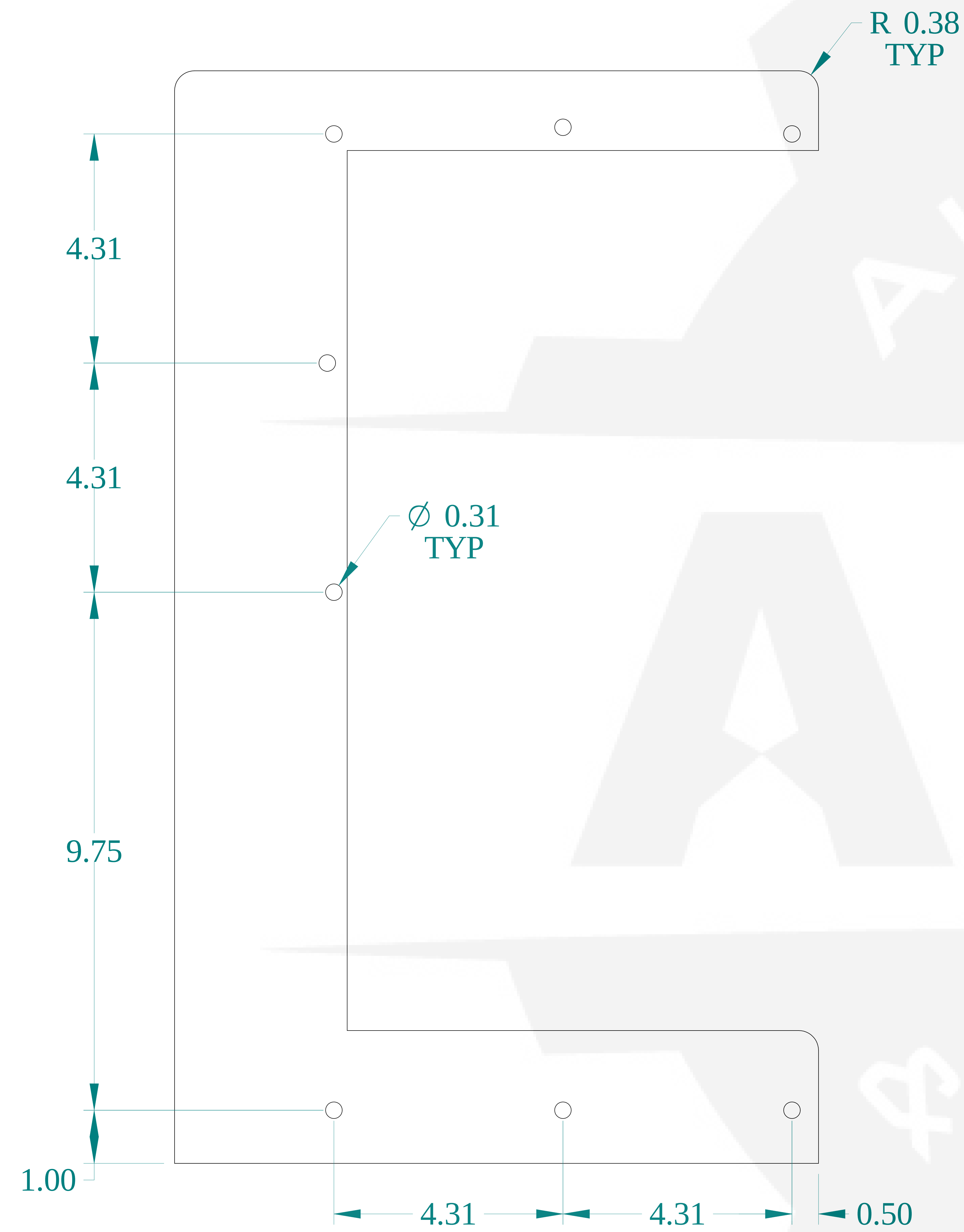
FRONT VIEW
