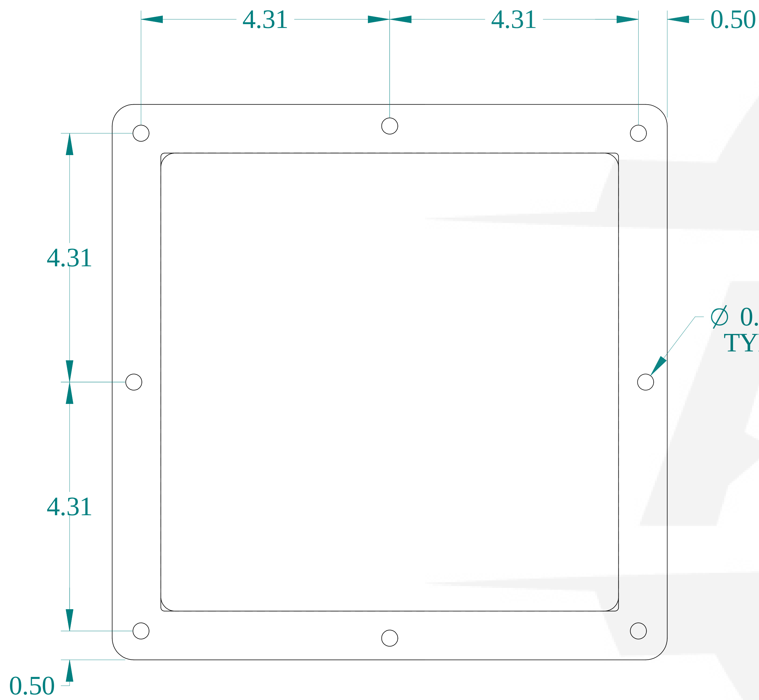
FRONT VIEW
