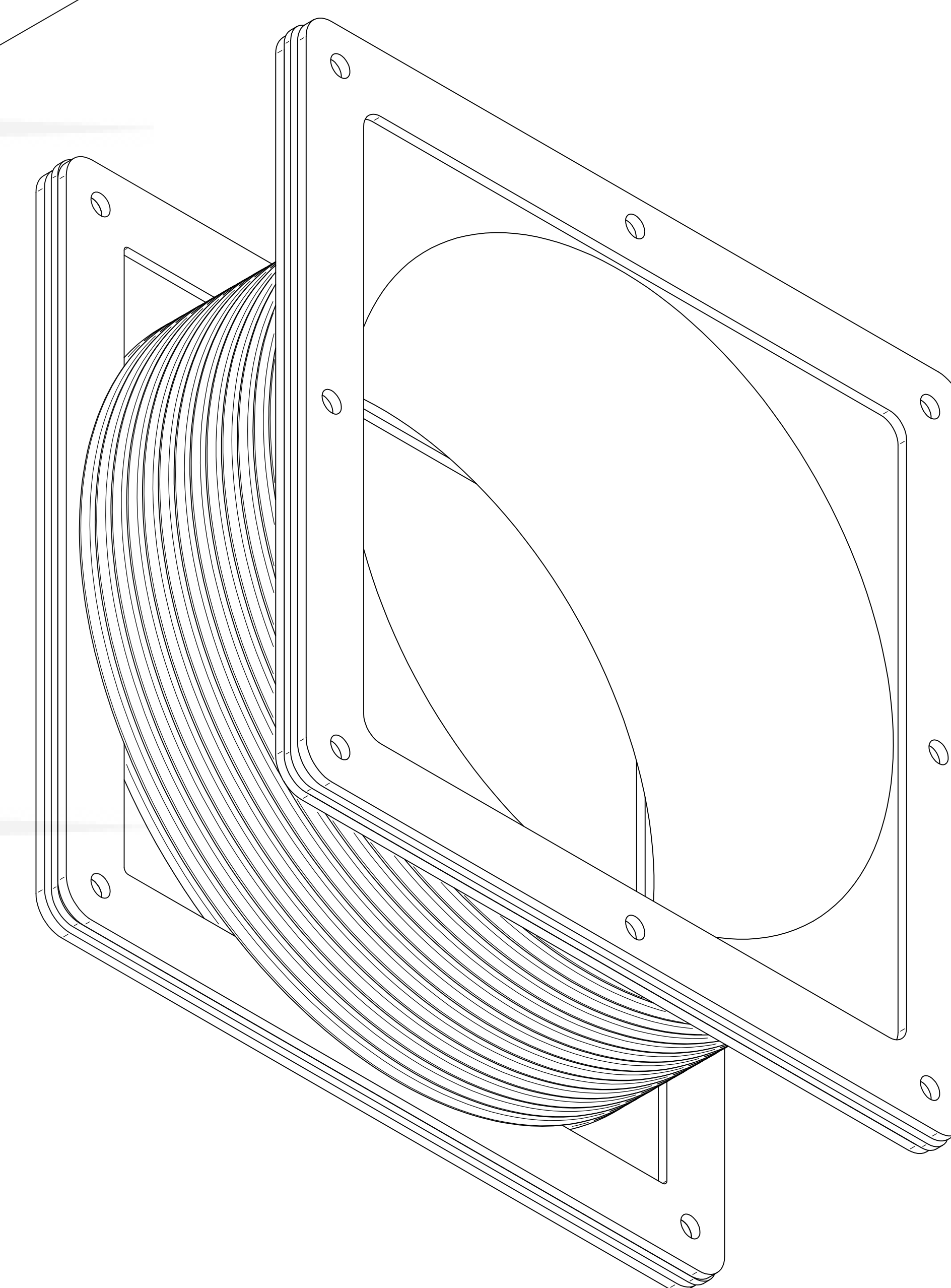
ISOMETRIC VIEWS
