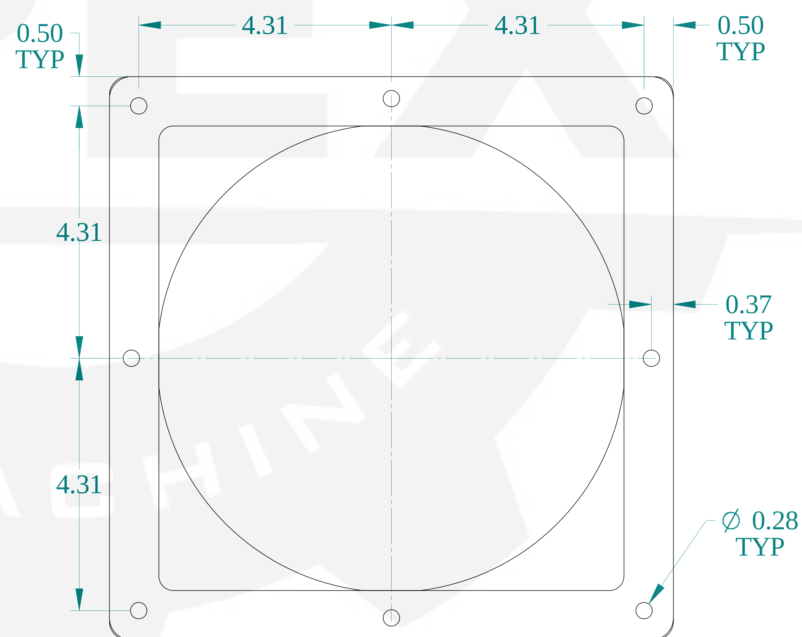
SIDE VIEW
