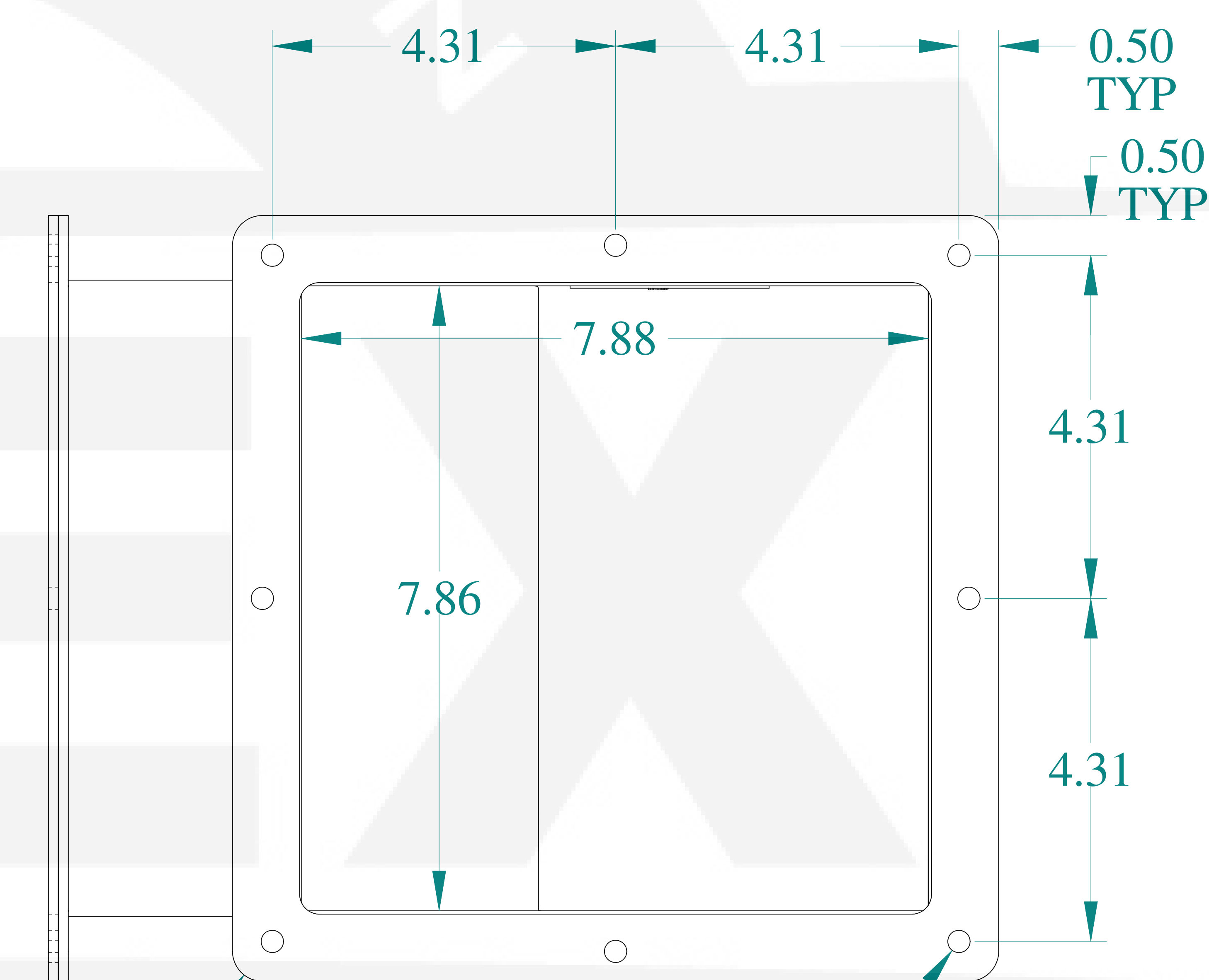
VIEW Z-Z
