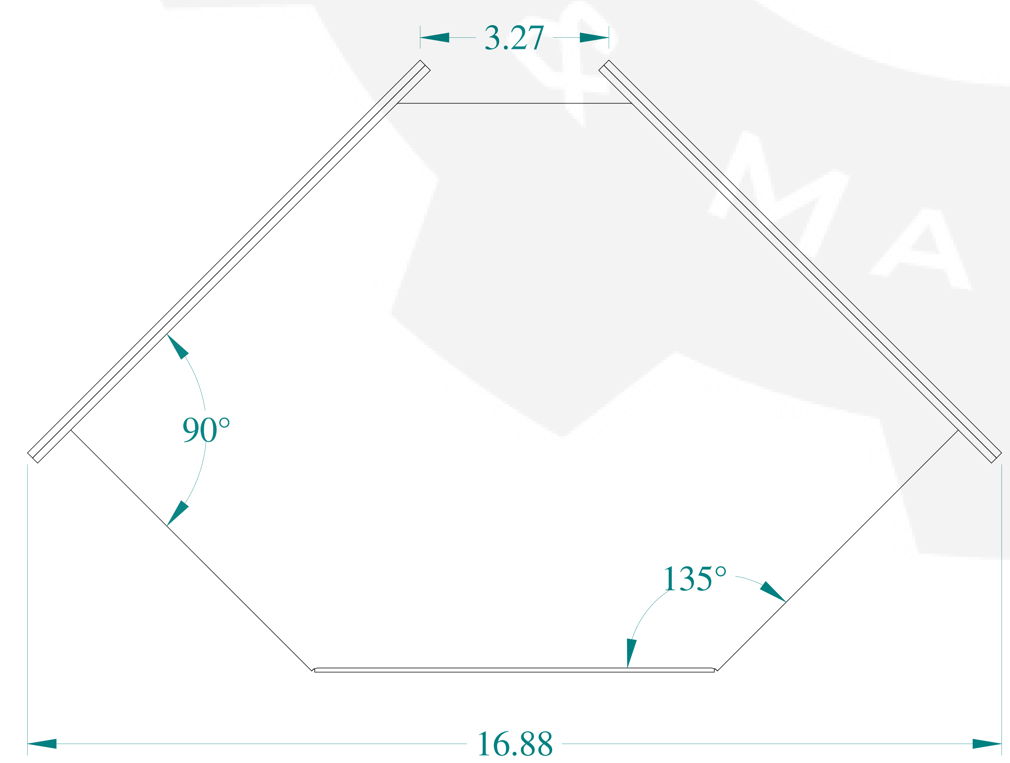
BOTTOM VIEW
