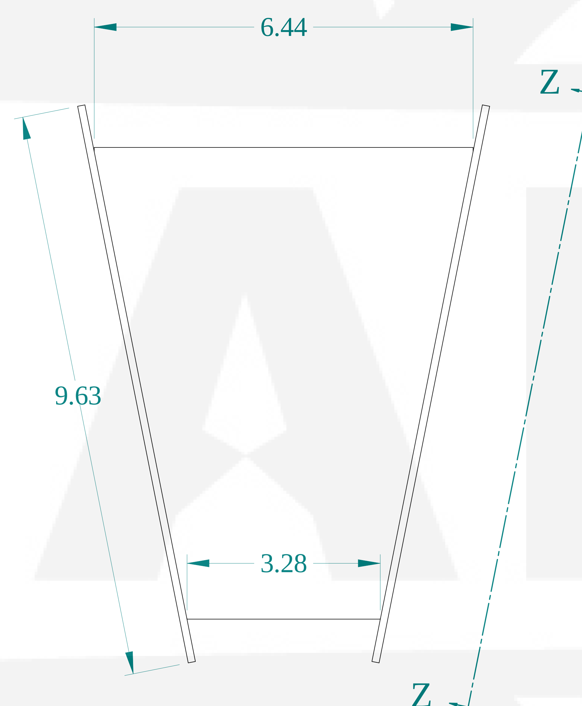
FRONT VIEW
