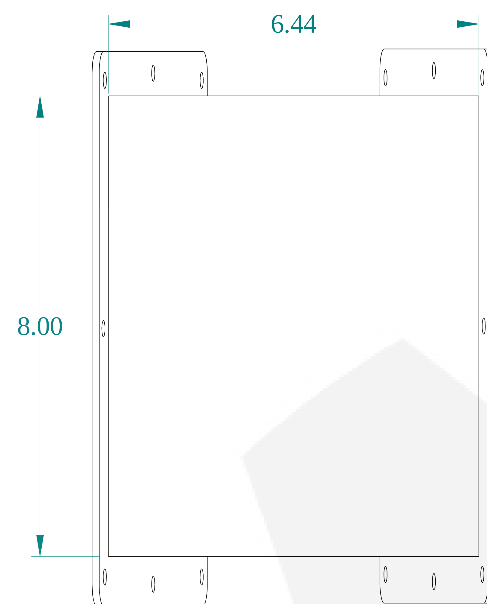
TOP VIEW
