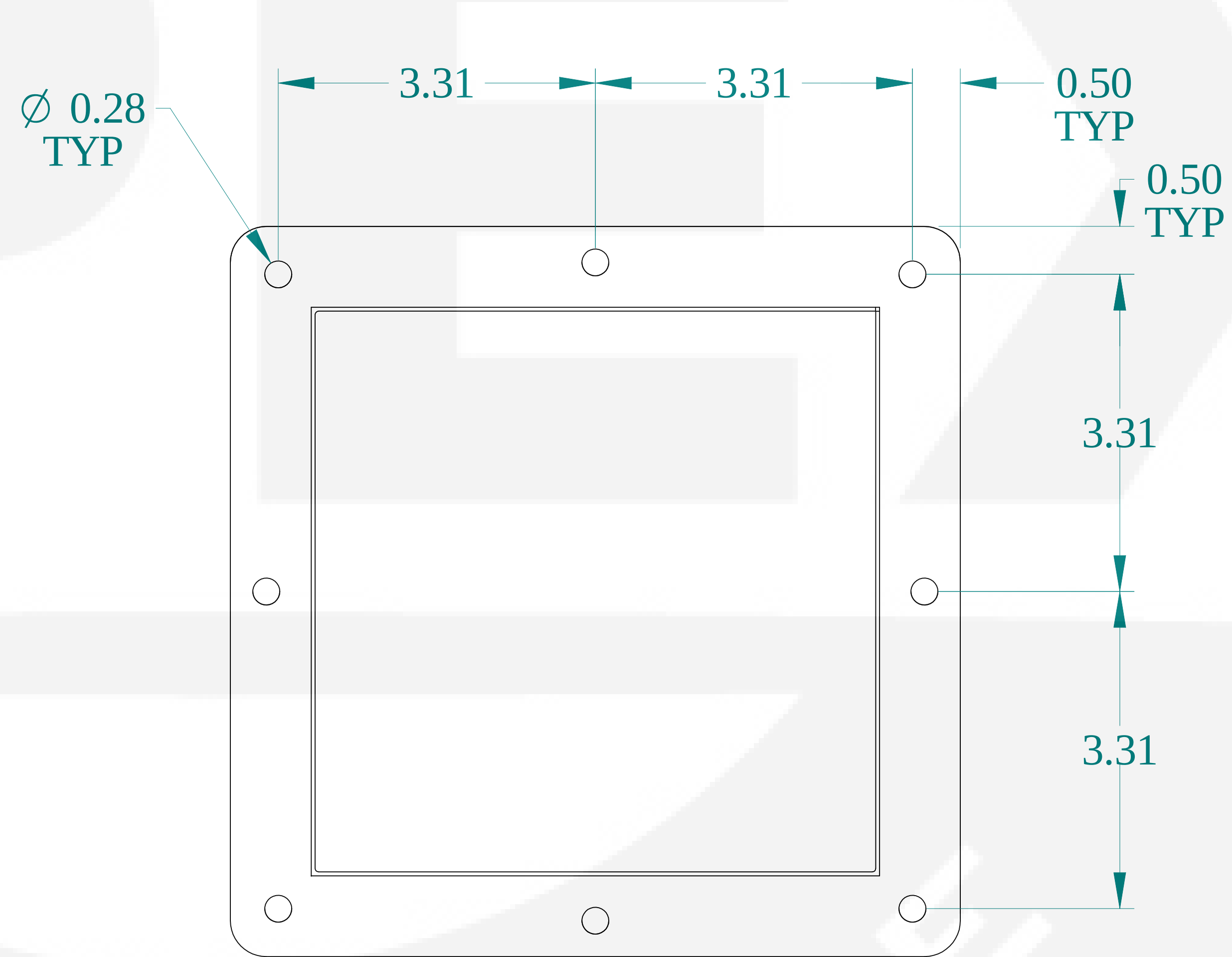
SIDE VIEW
