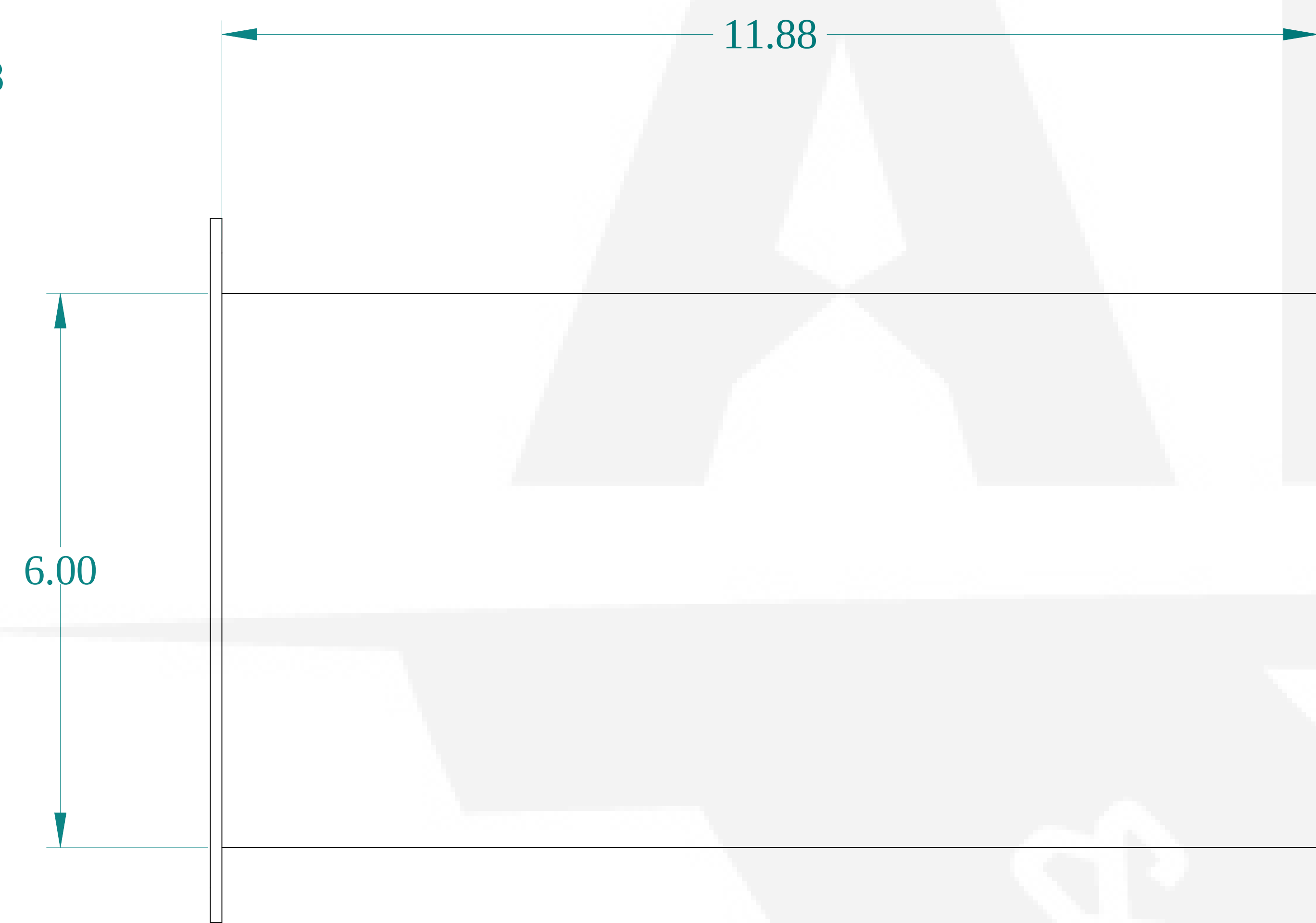
FRONT VIEW
