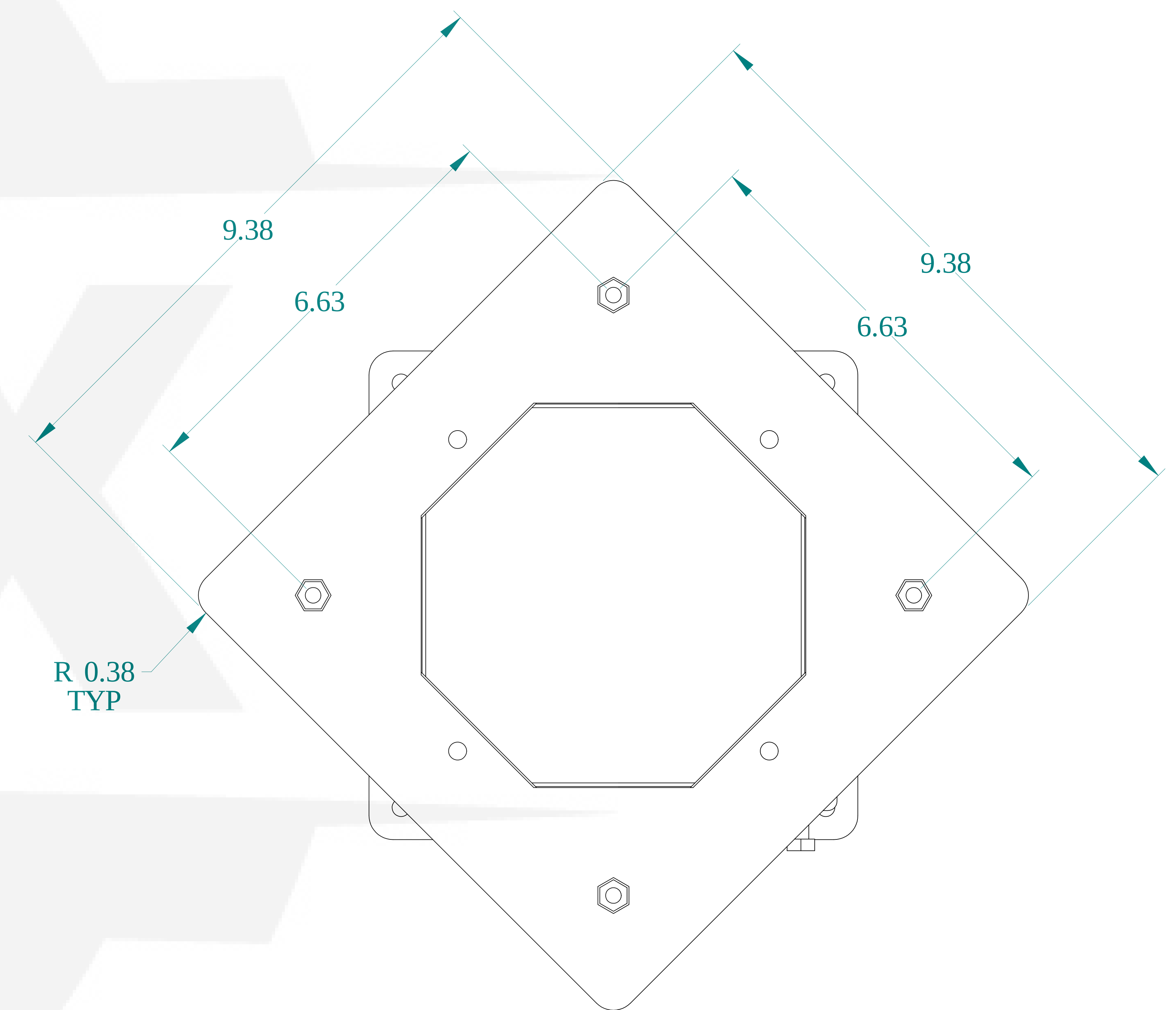
BACK VIEW
