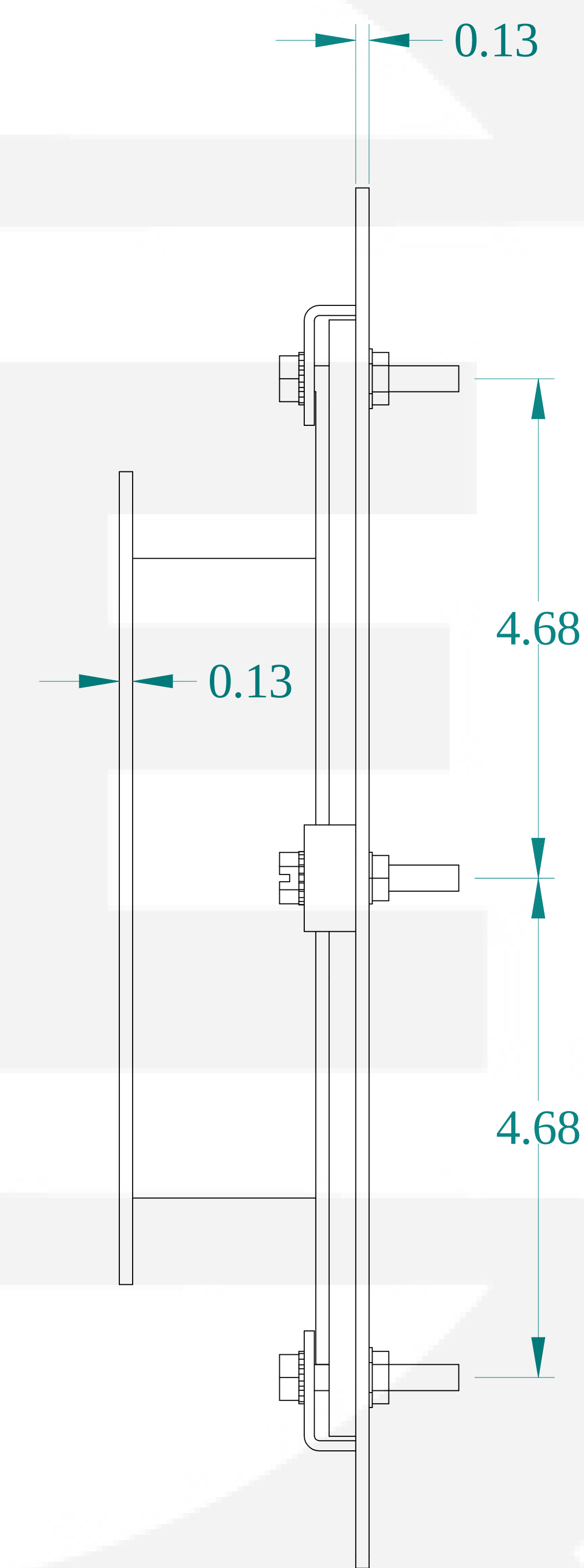
SIDE VIEW
