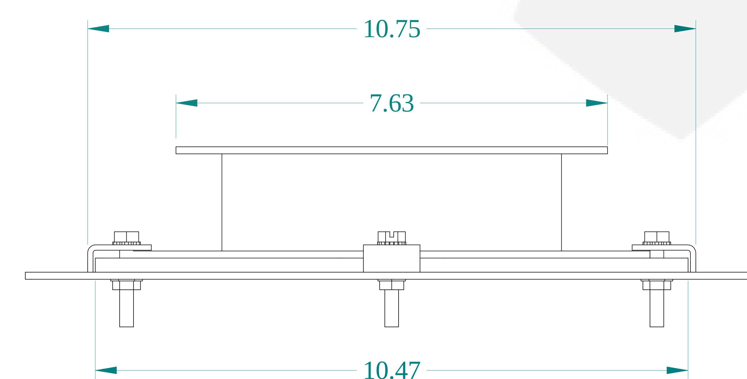
BOTTOM VIEW
