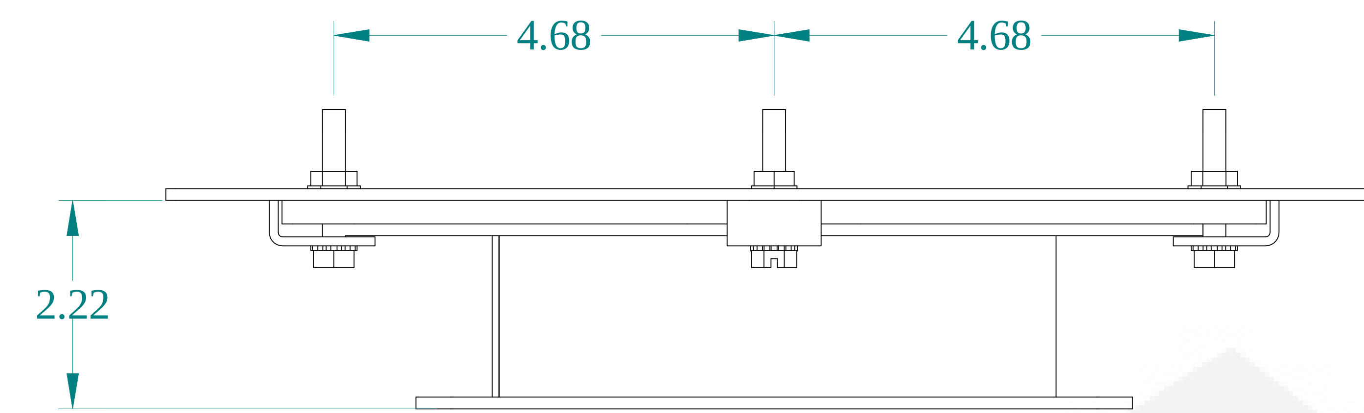
TOP VIEW
