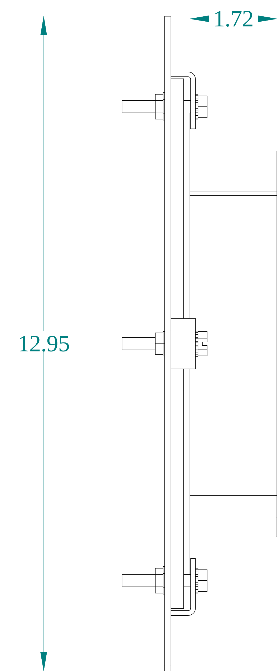
SIDE VIEW
