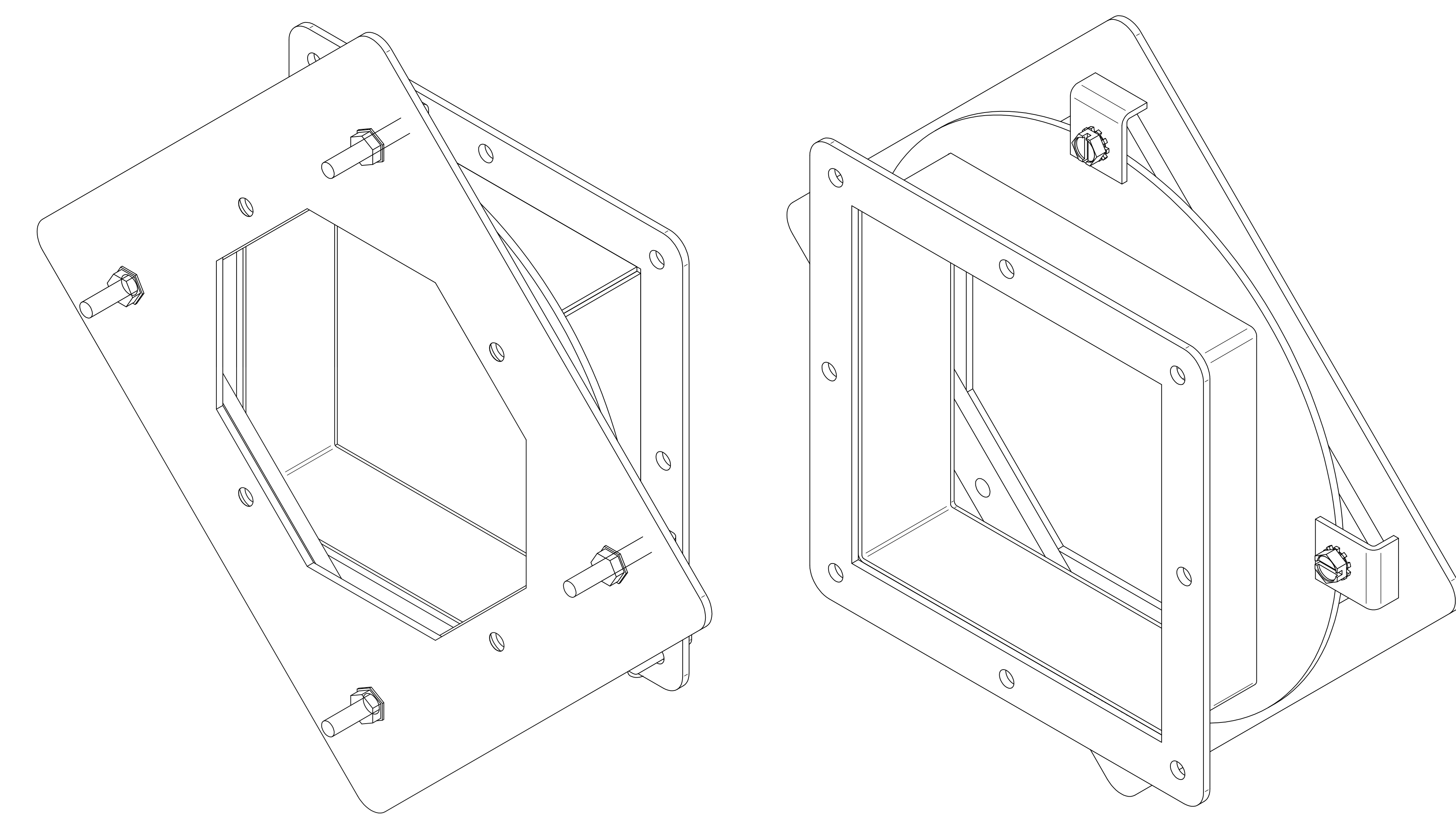
ISOMETRIC VIEWS
