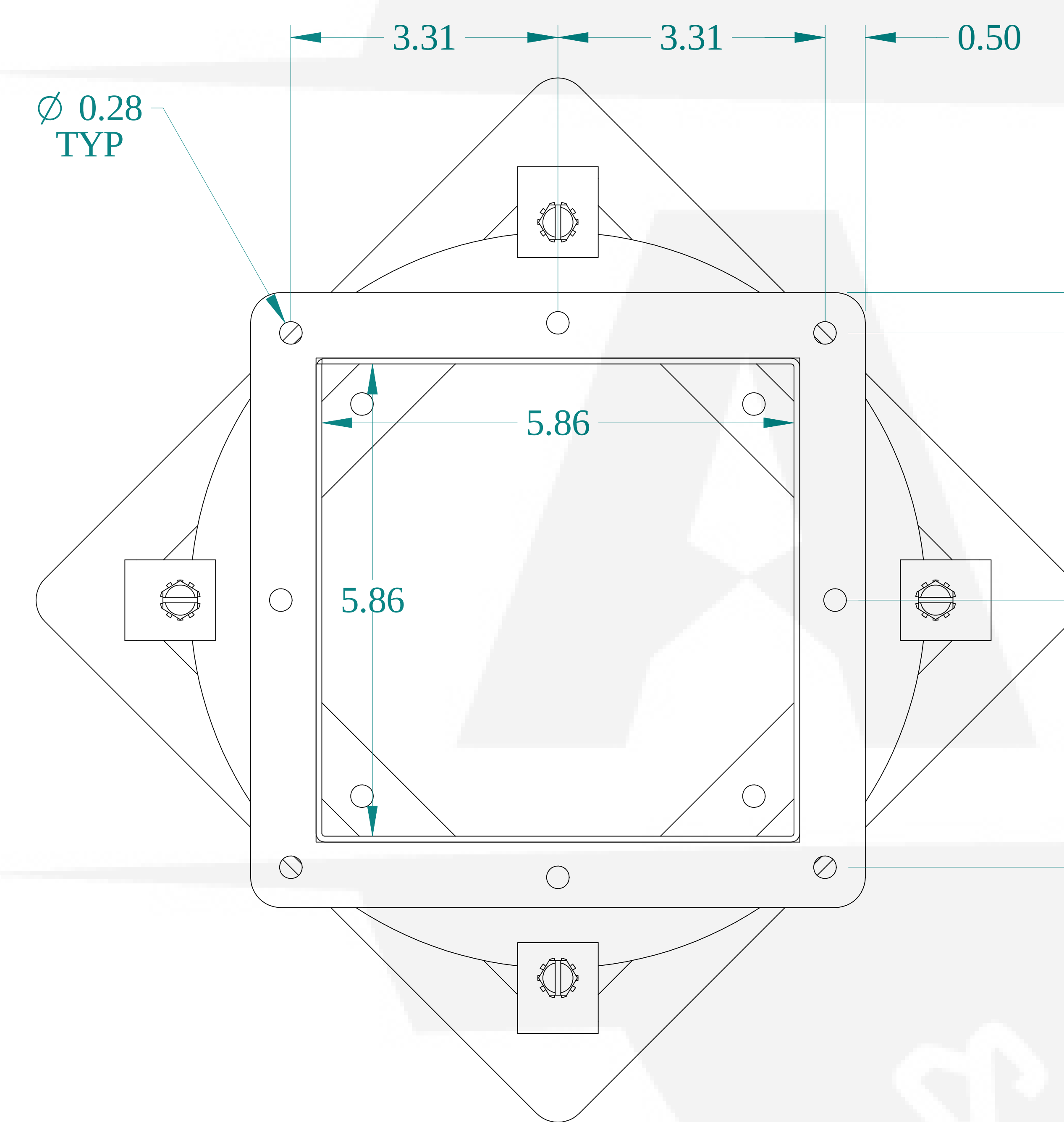
FRONT VIEW
