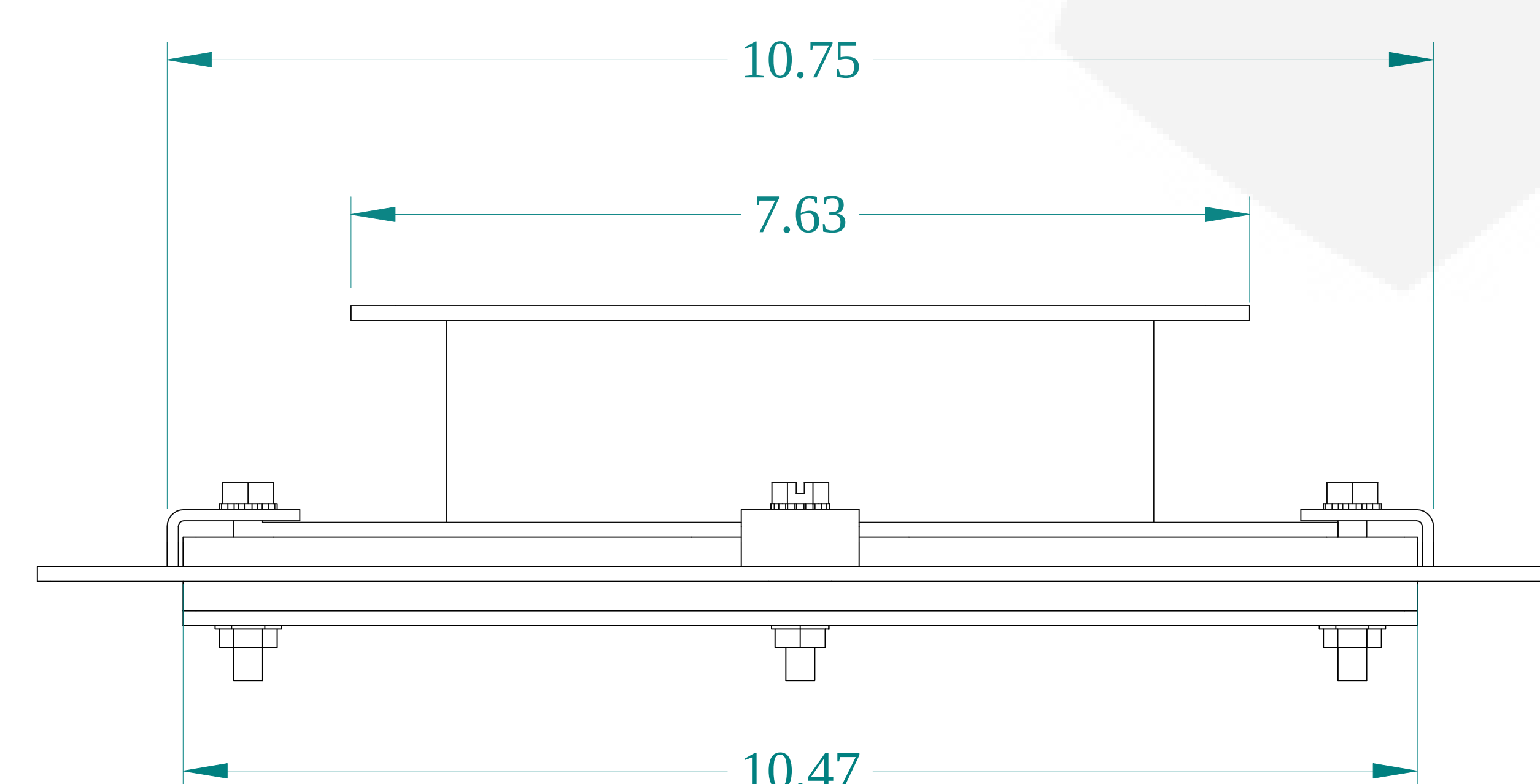
BOTTOM VIEW
