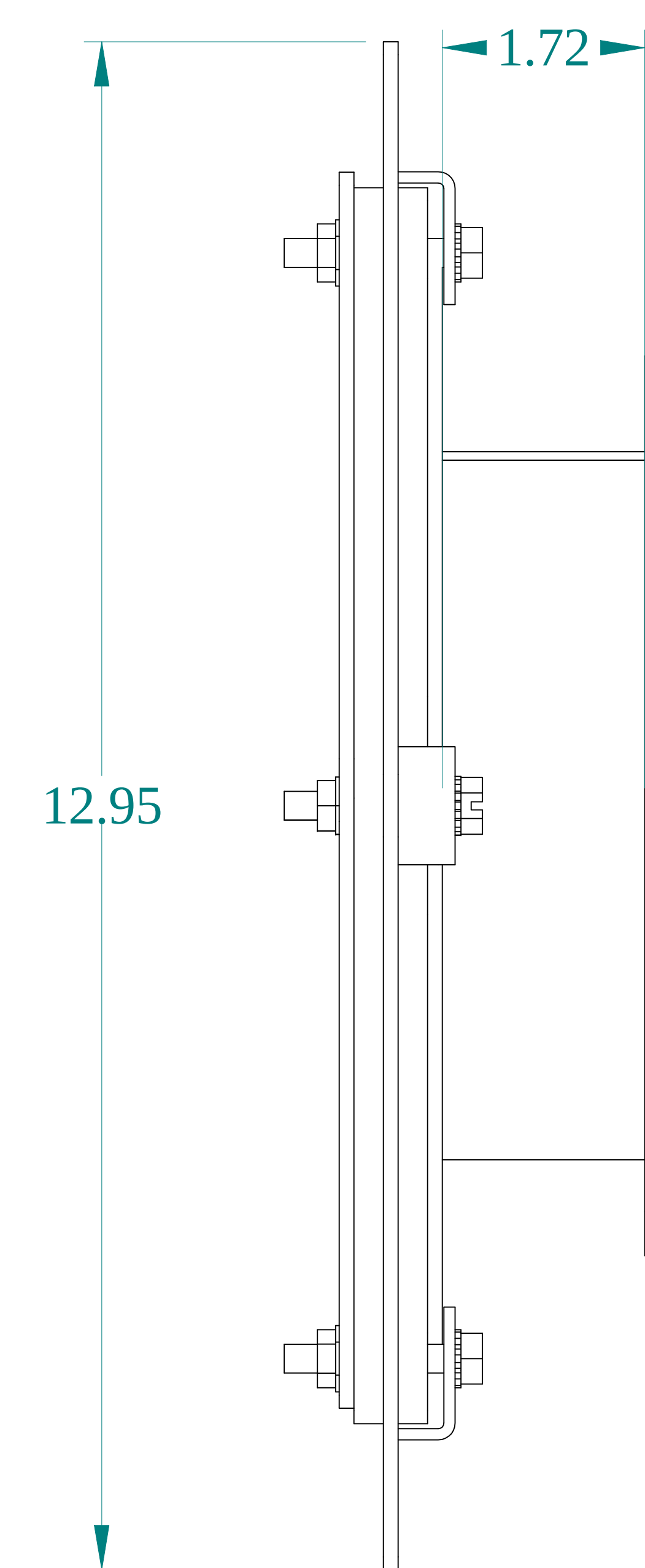
SIDE VIEW
