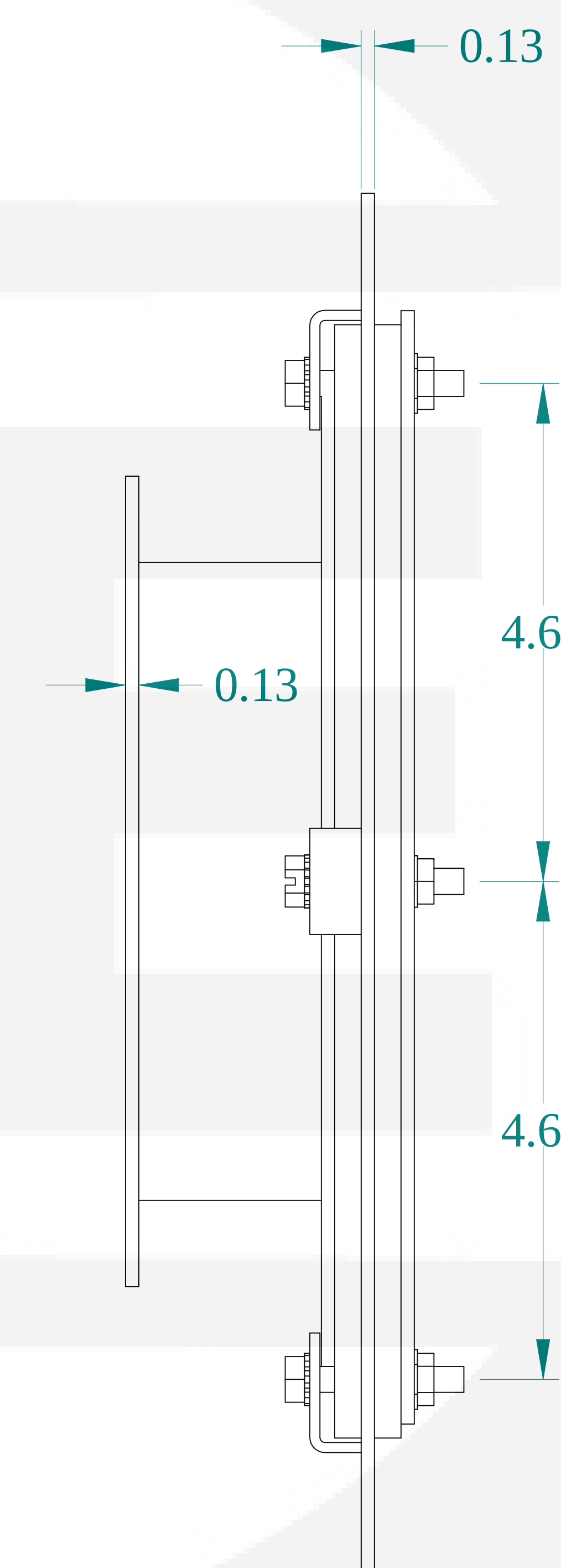
SIDE VIEW
