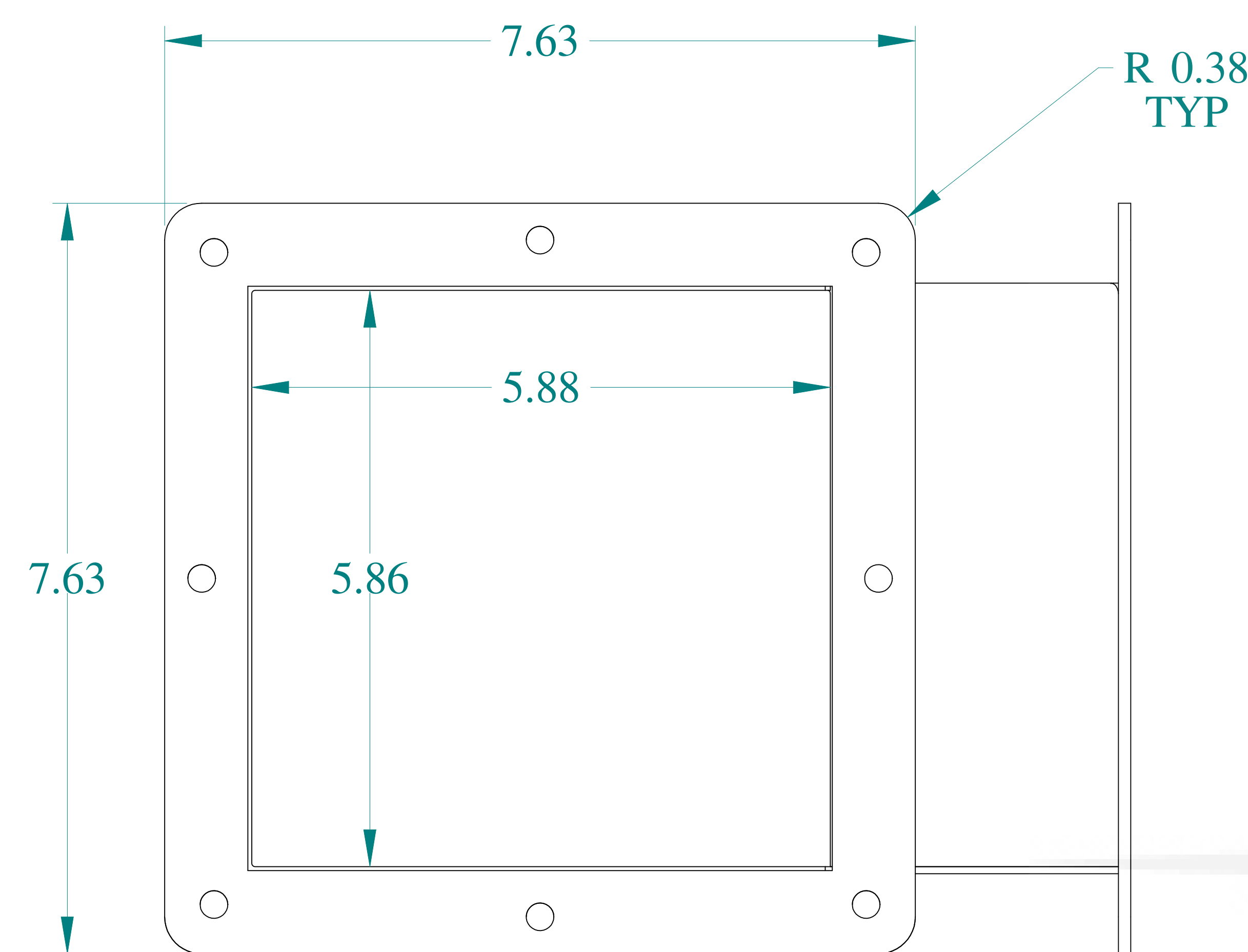
SIDE VIEW
