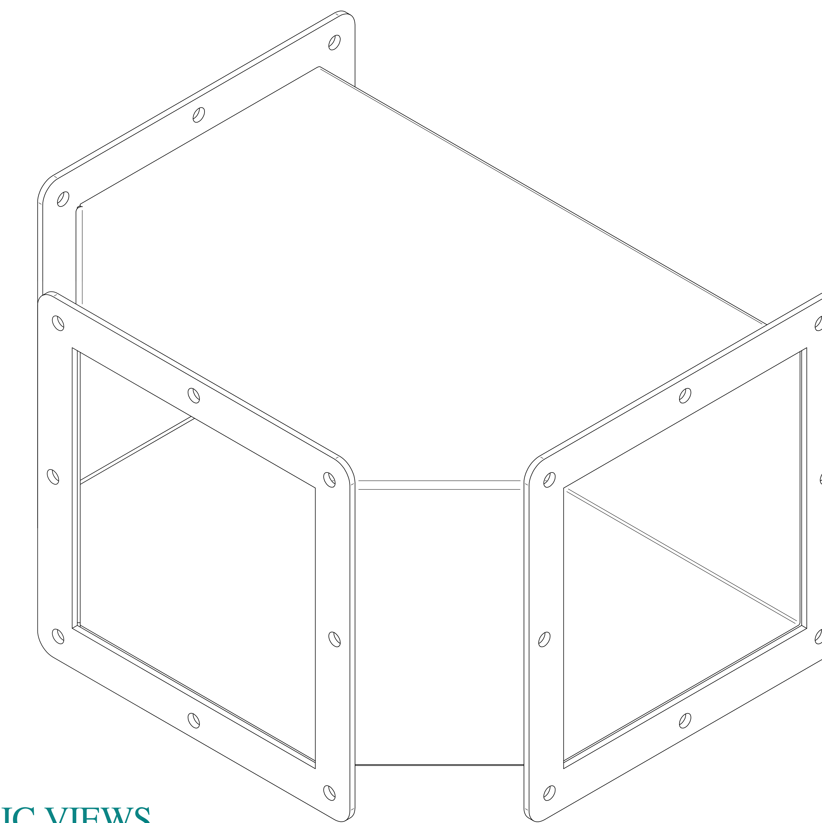
ISOMETRIC VIEWS
