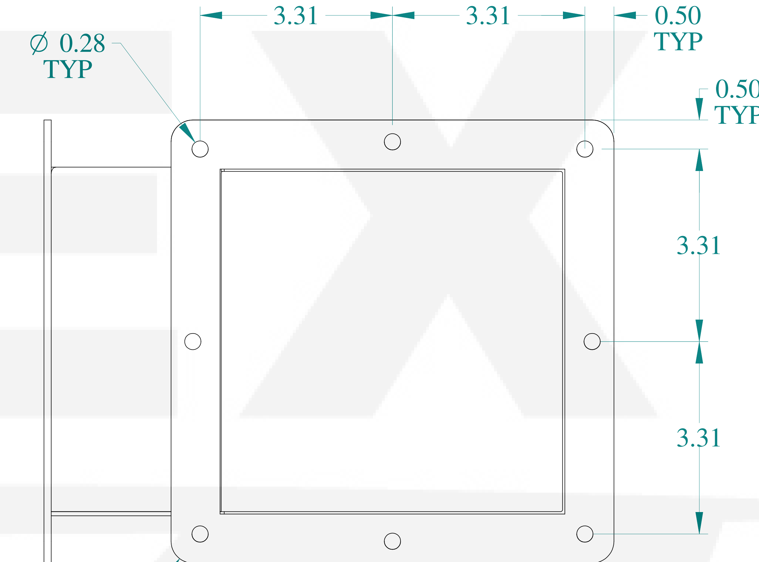
SIDE VIEW
