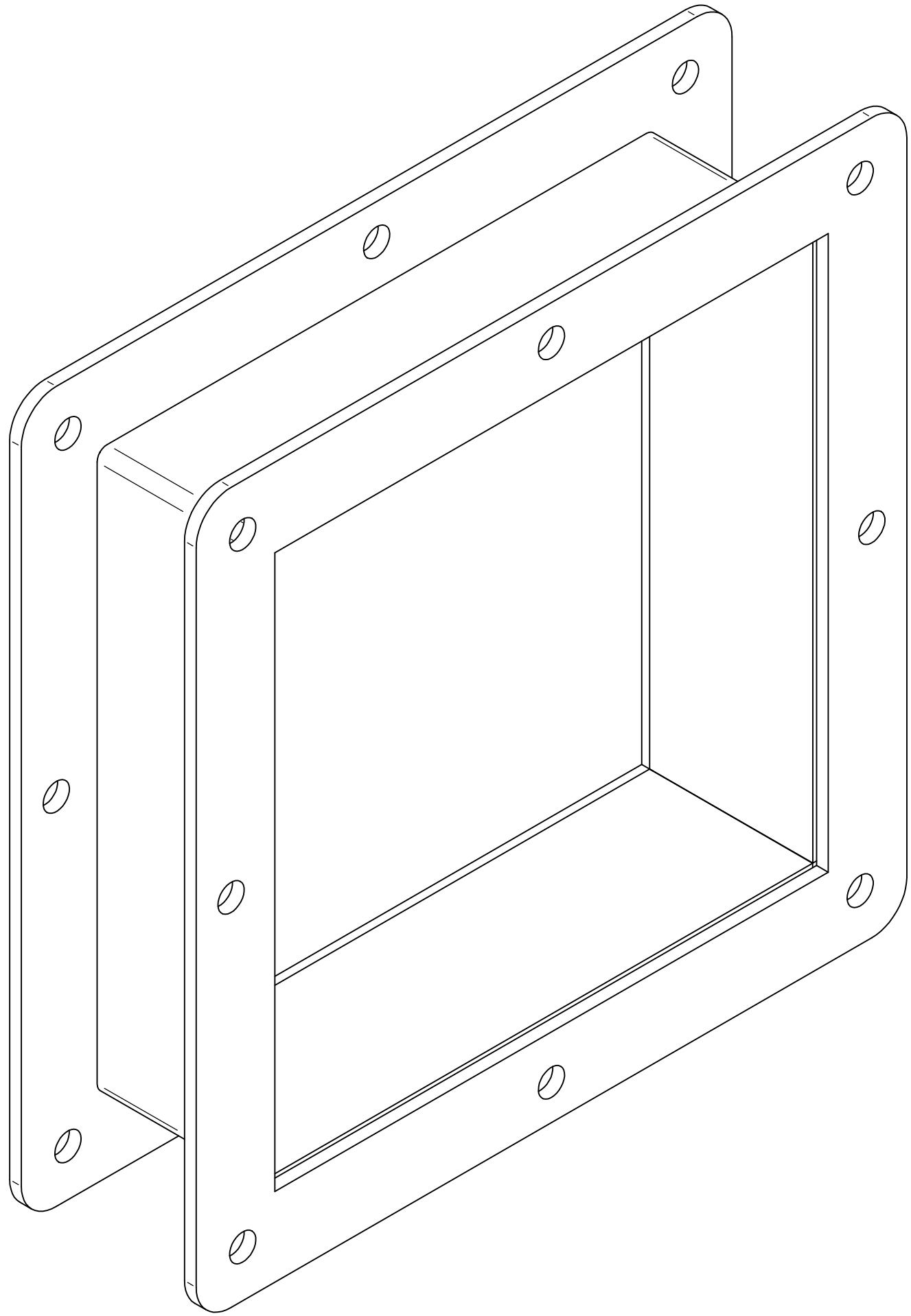
ISOMETRIC VIEWS
