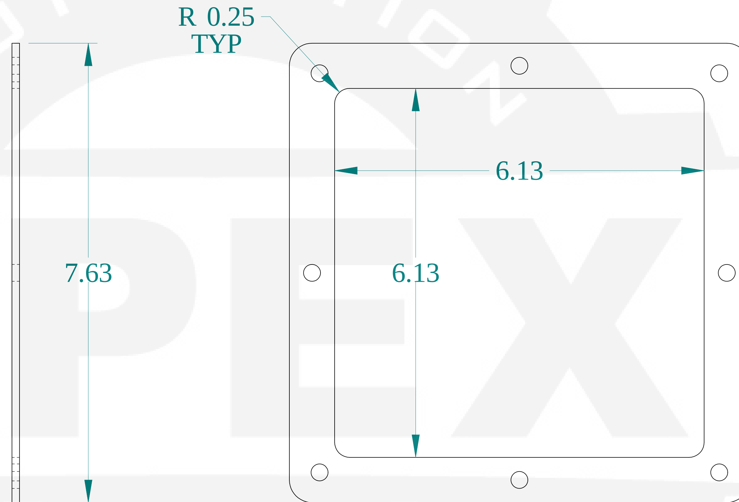
BACK VIEW
