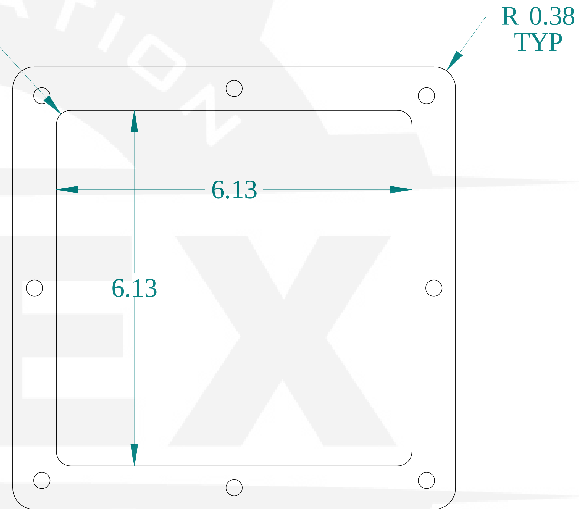
BACK VIEW
