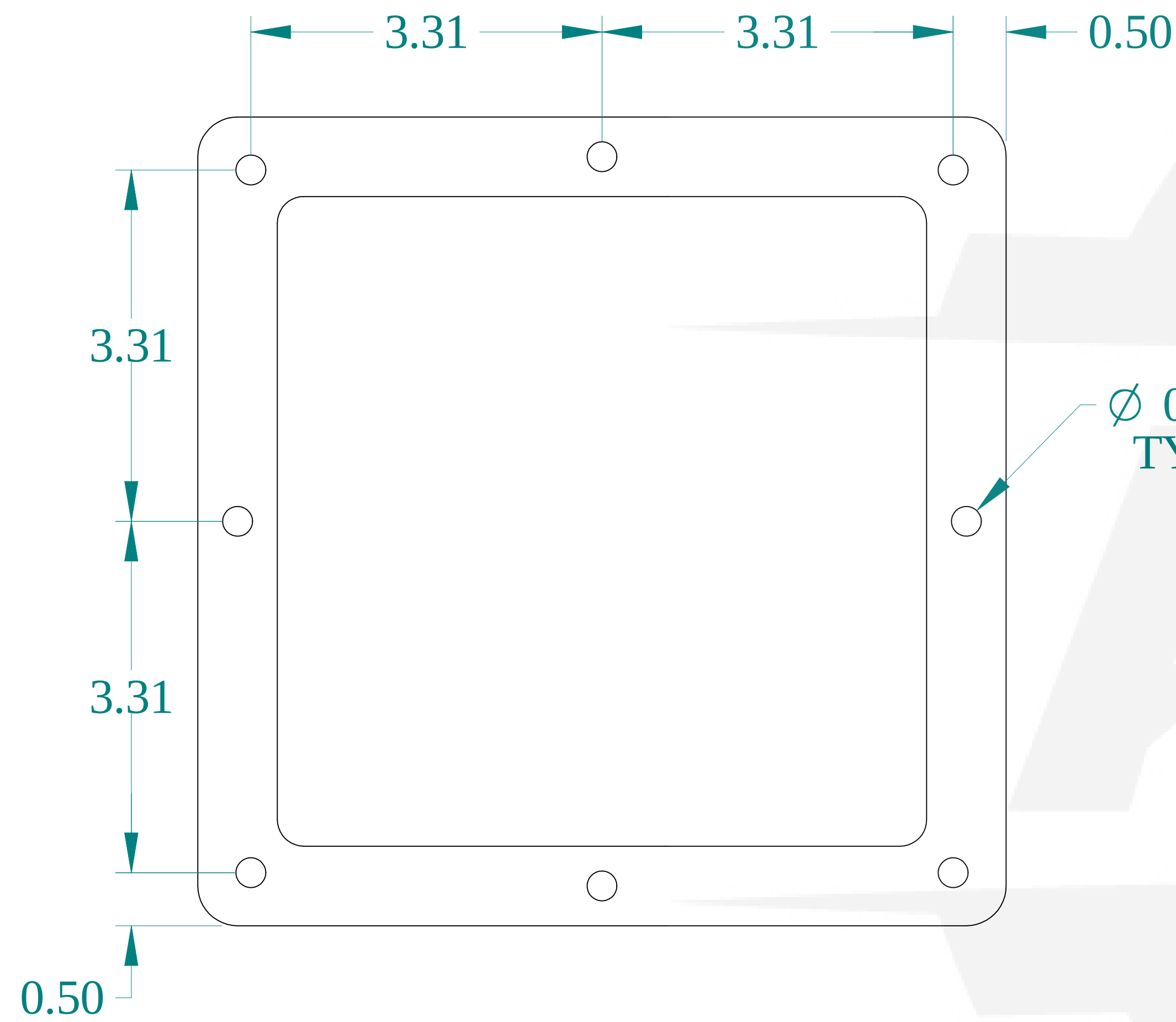
FRONT VIEW
