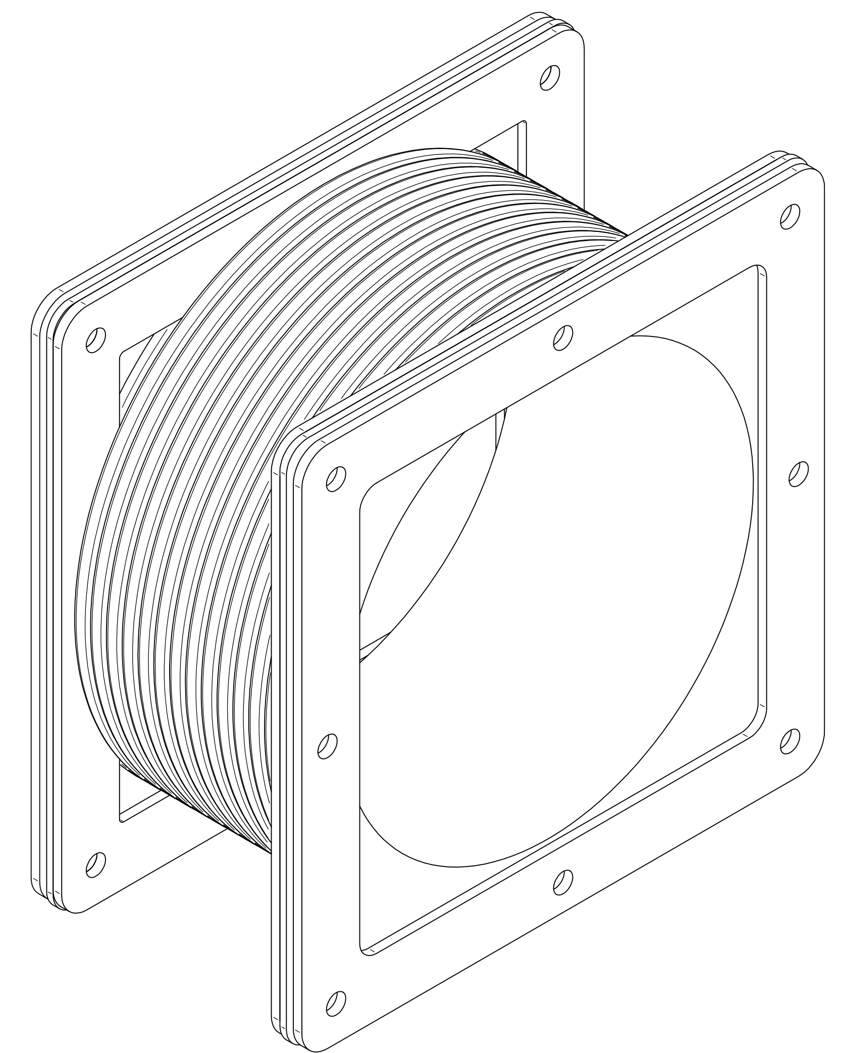
ISOMETRIC VIEWS
