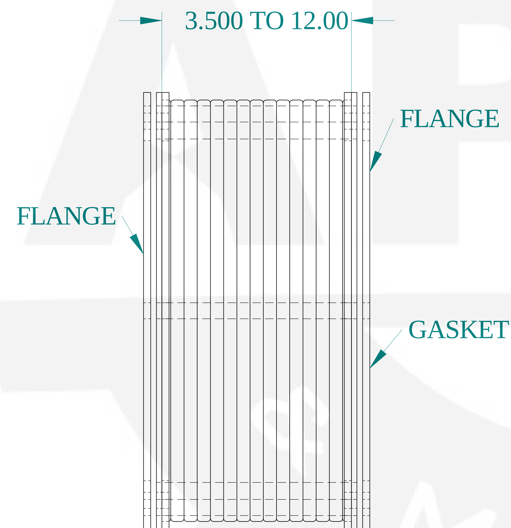
FRONT VIEW
