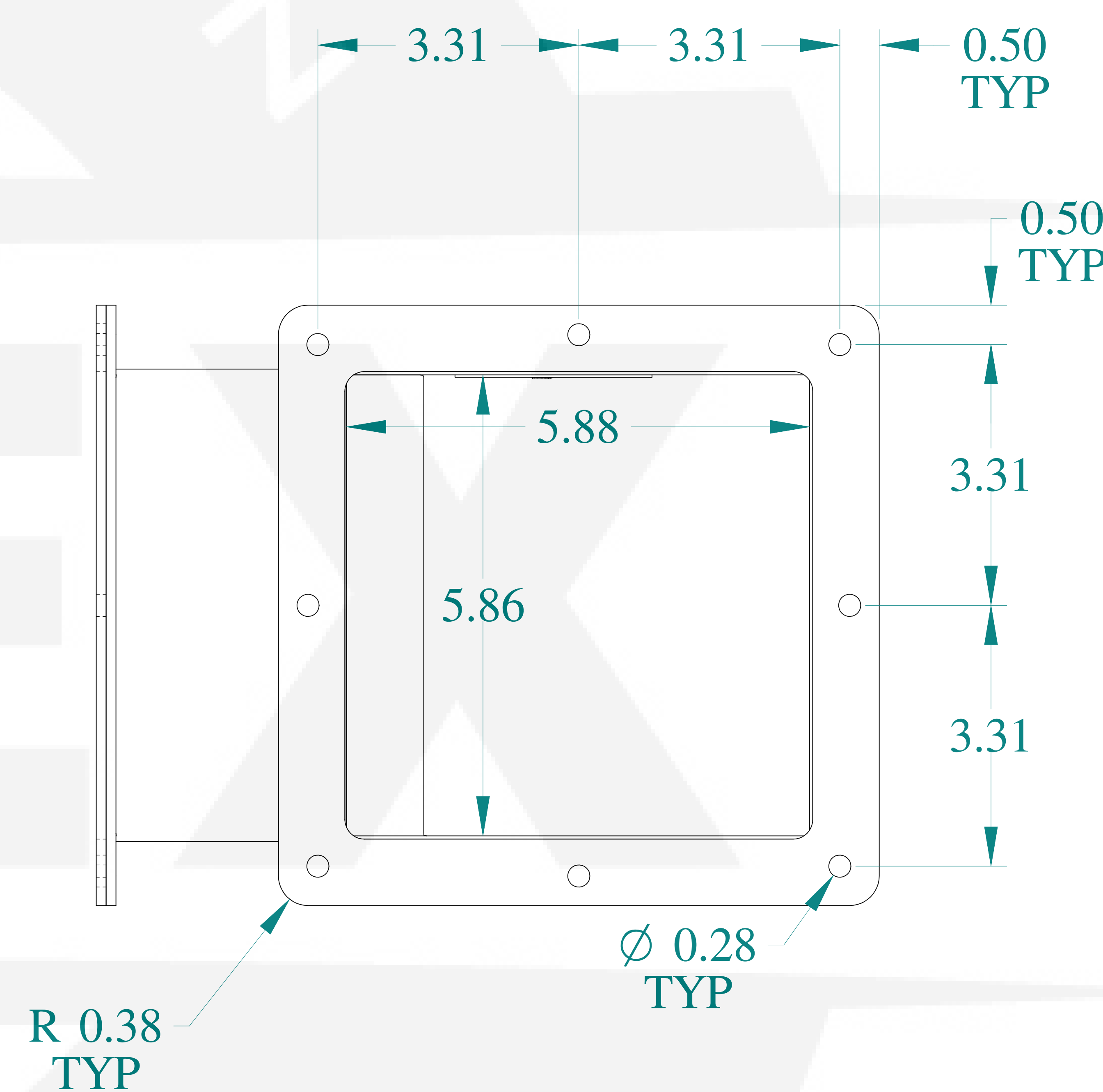
VIEW Z-Z
