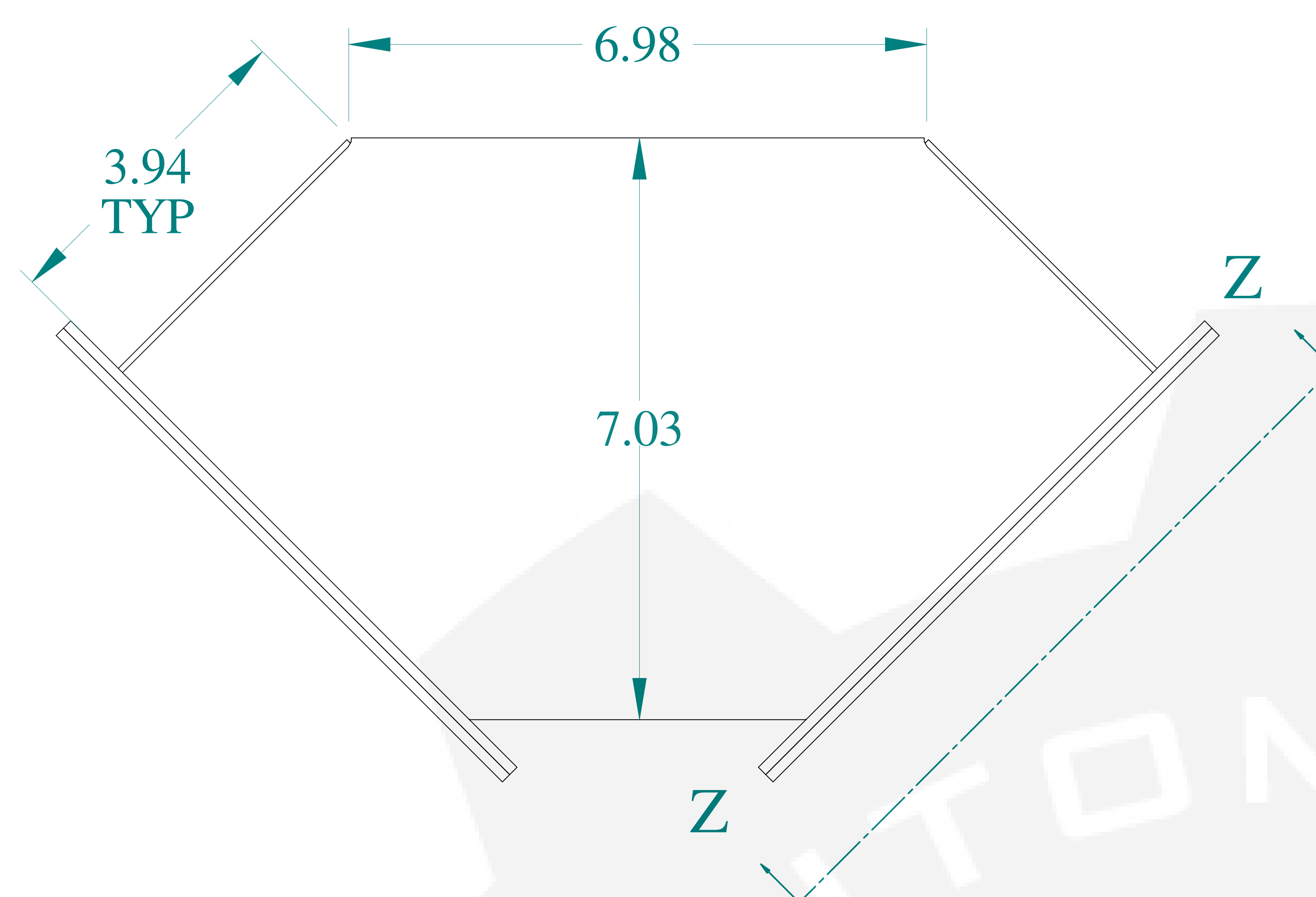
TOP VIEW
