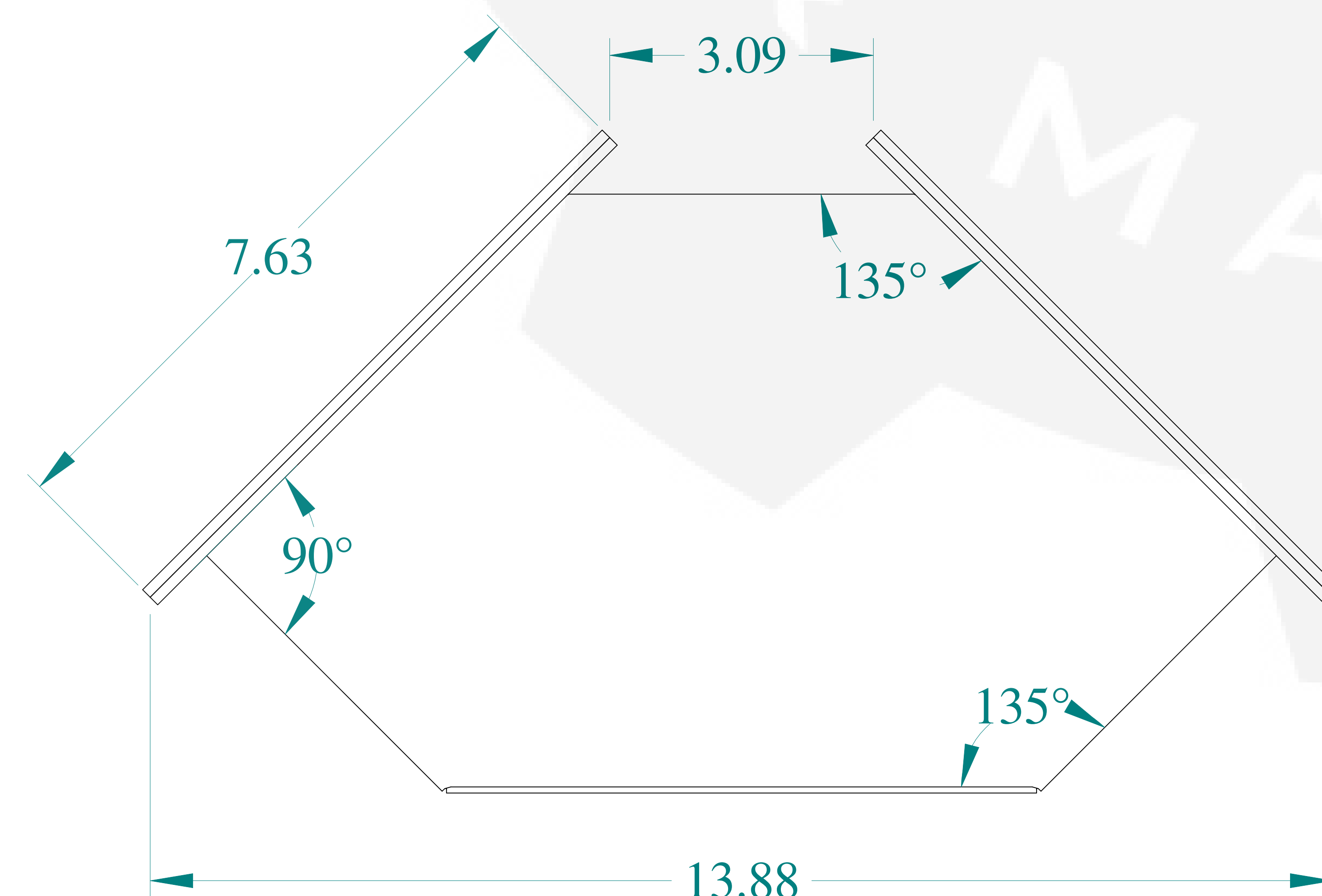
BOTTOM VIEW
