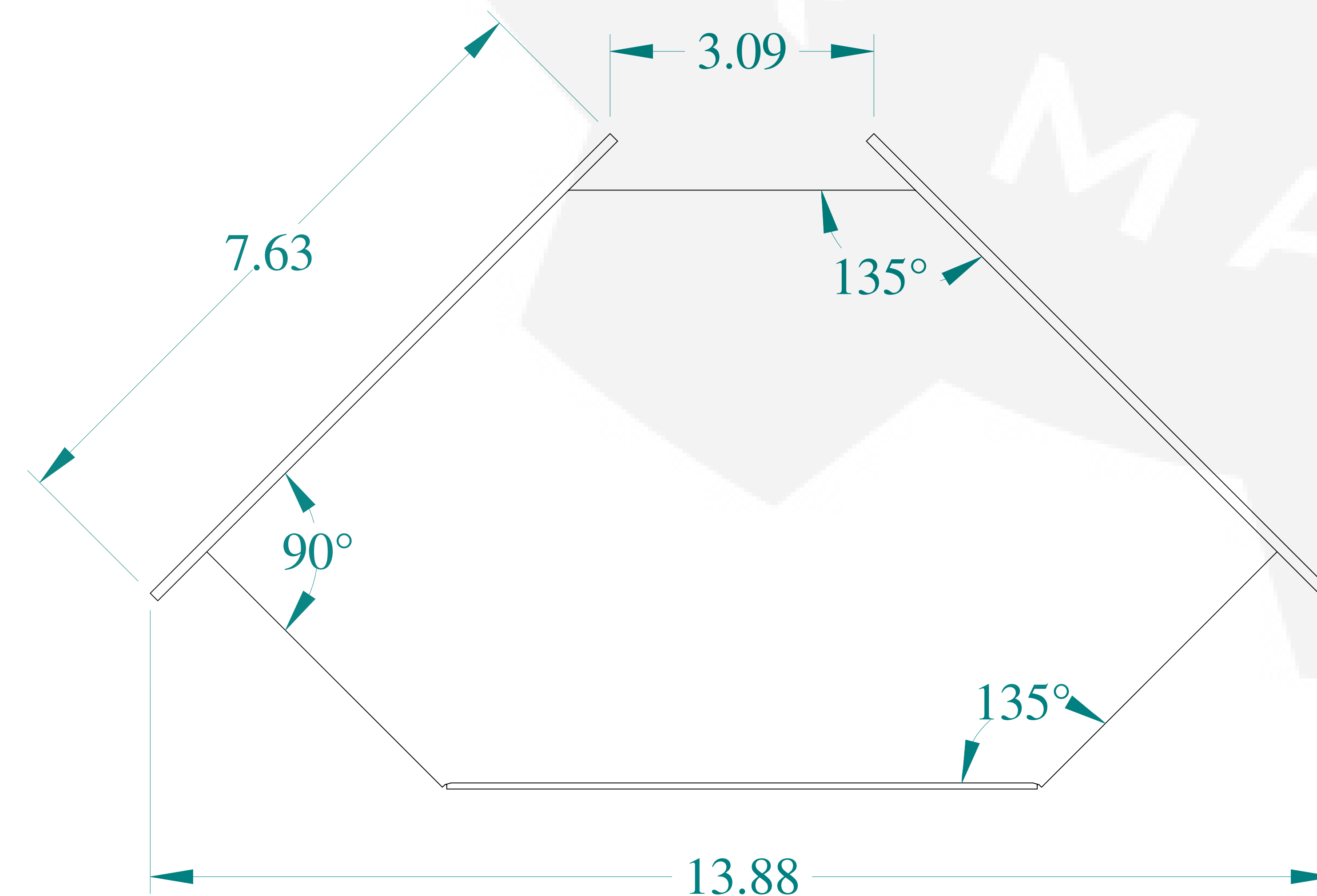
BOTTOM VIEW
