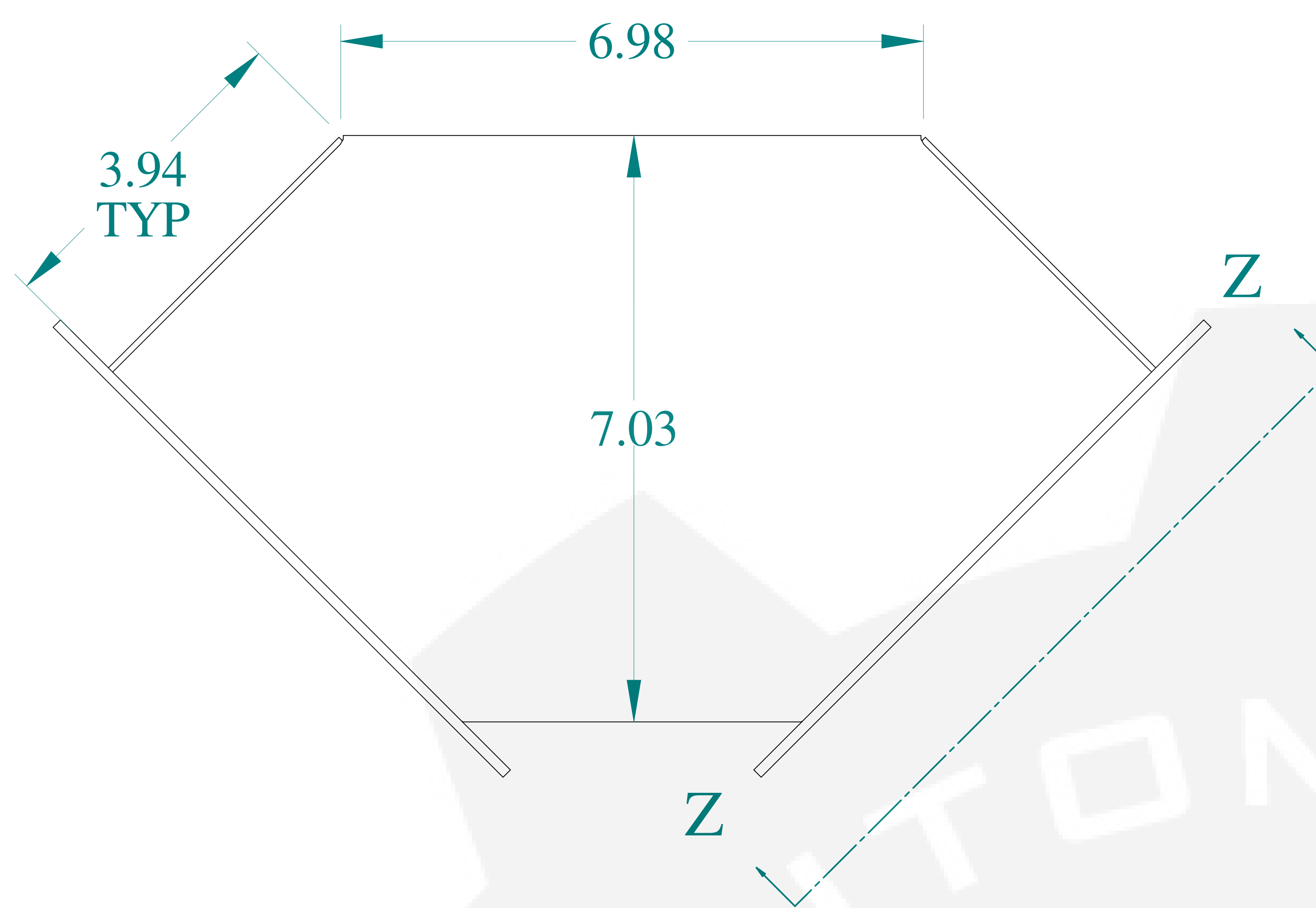
TOP VIEW
