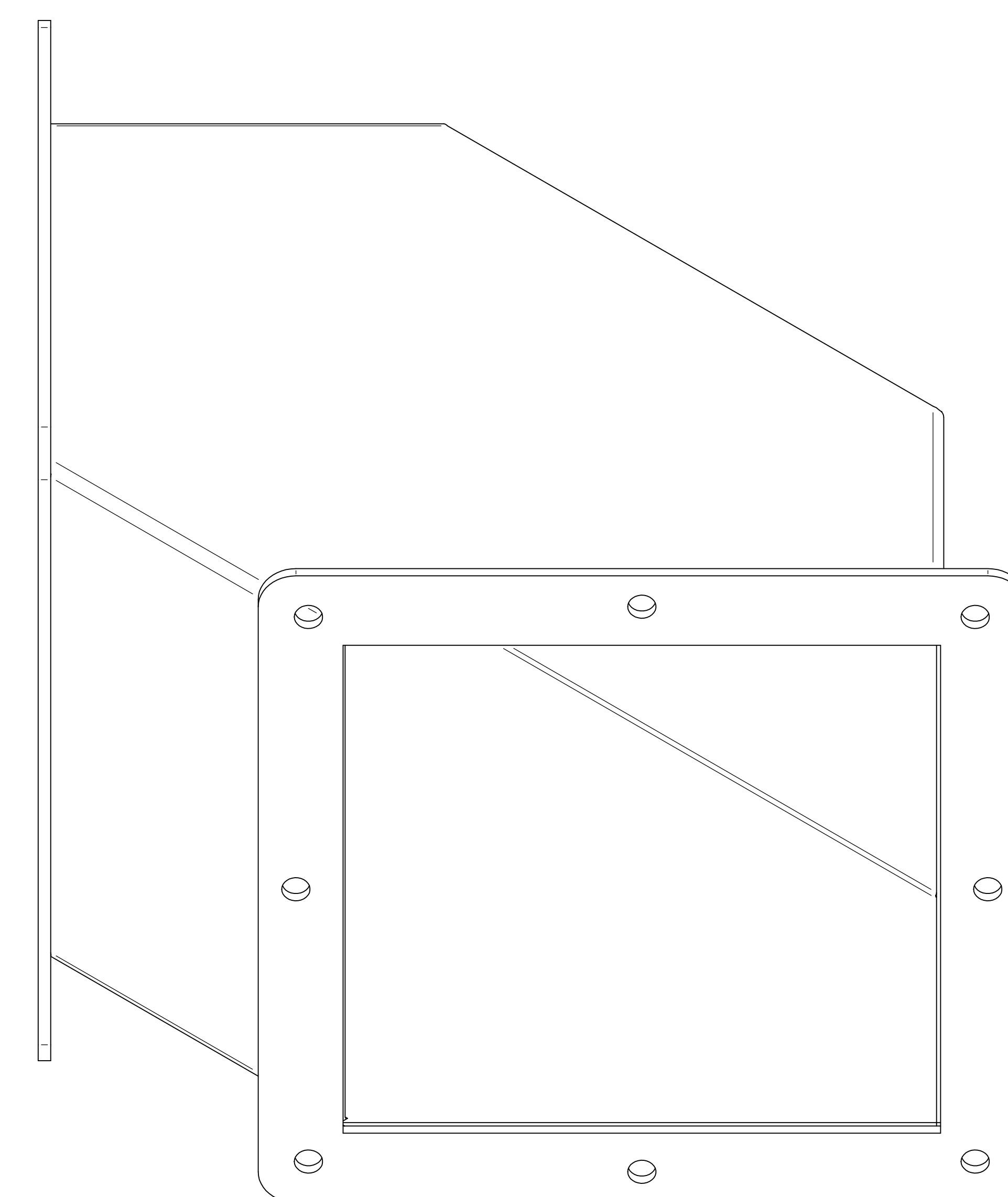
ISOMETRIC VIEWS
