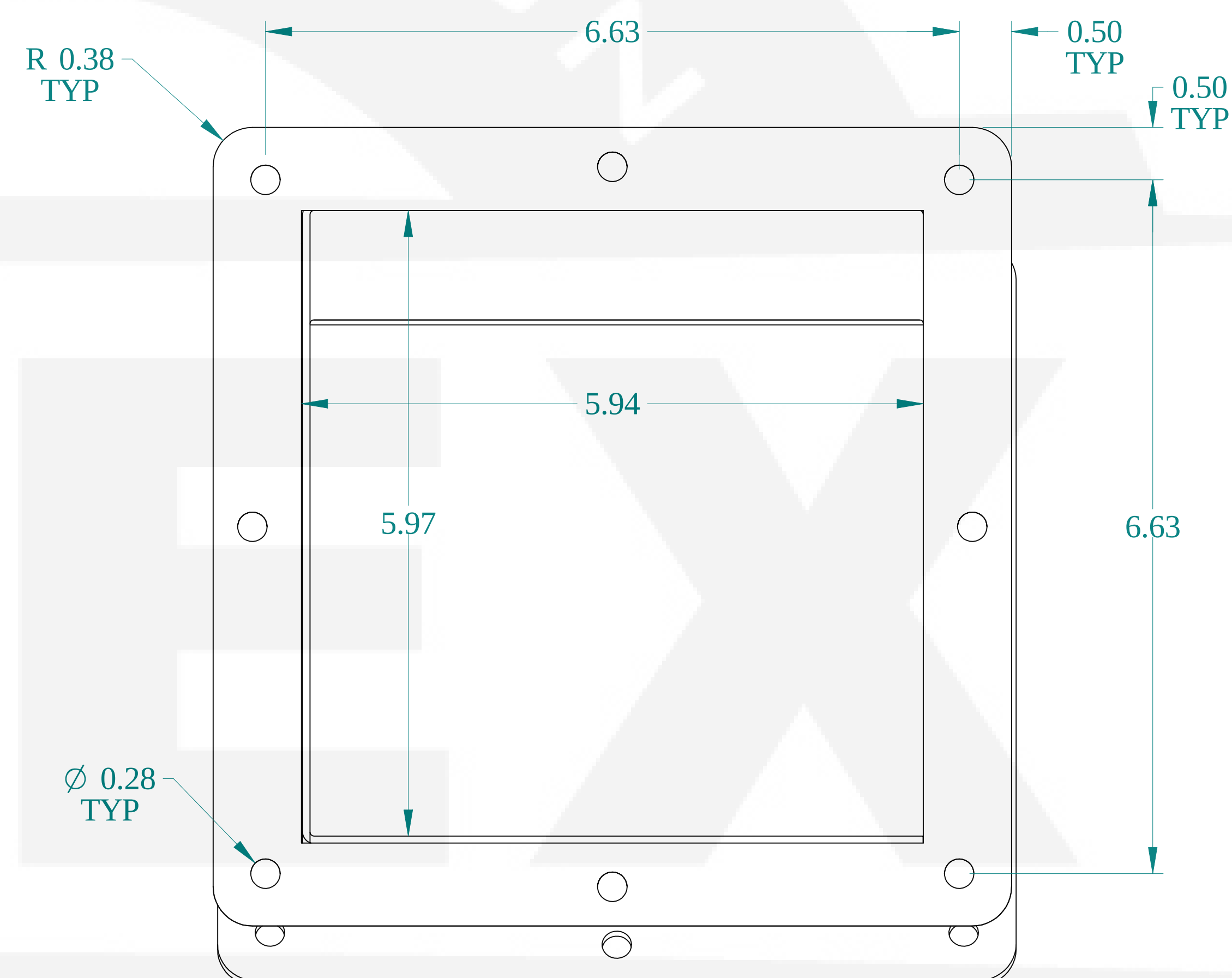
VIEW Z-Z
