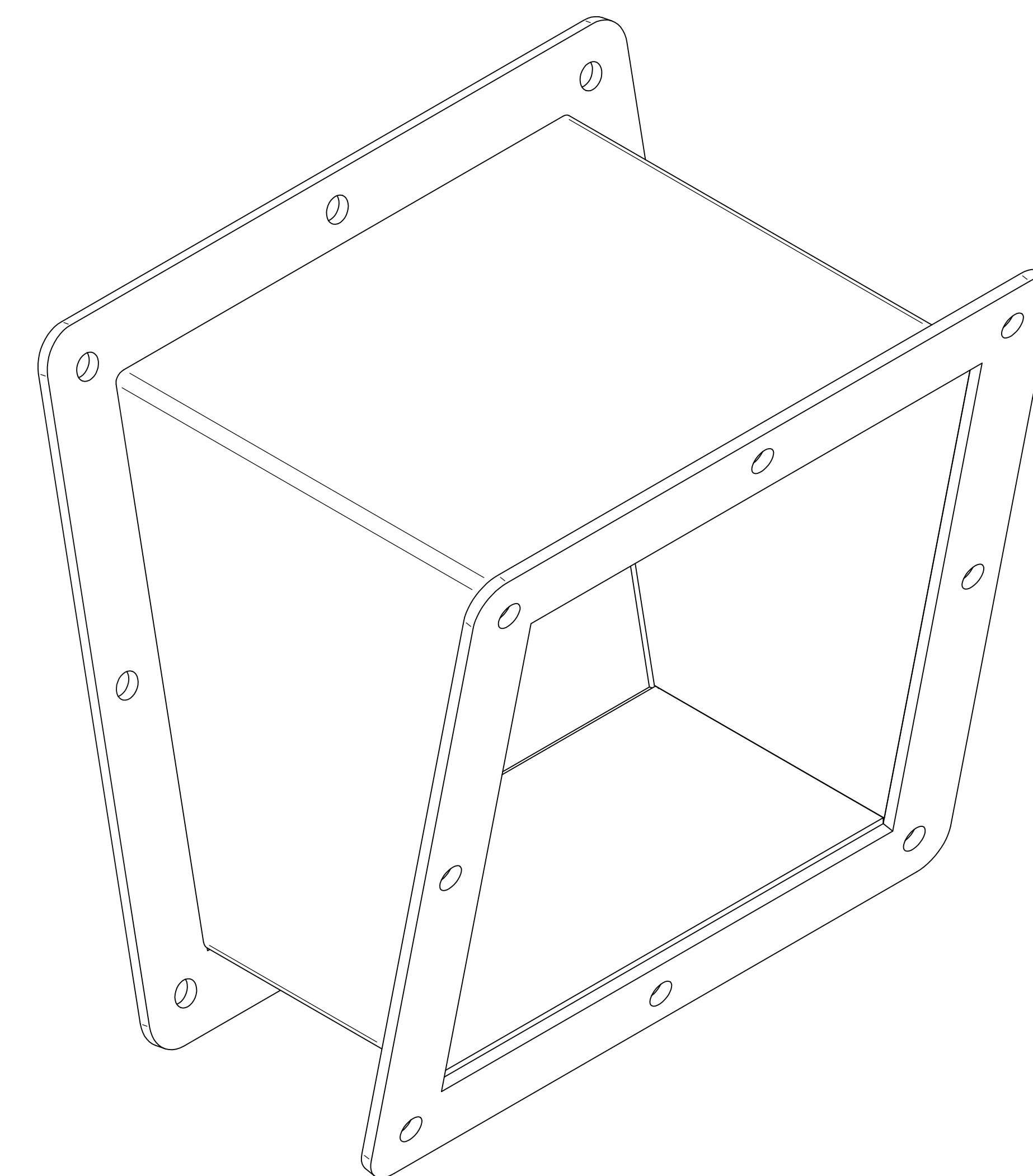
ISOMETRIC VIEWS
