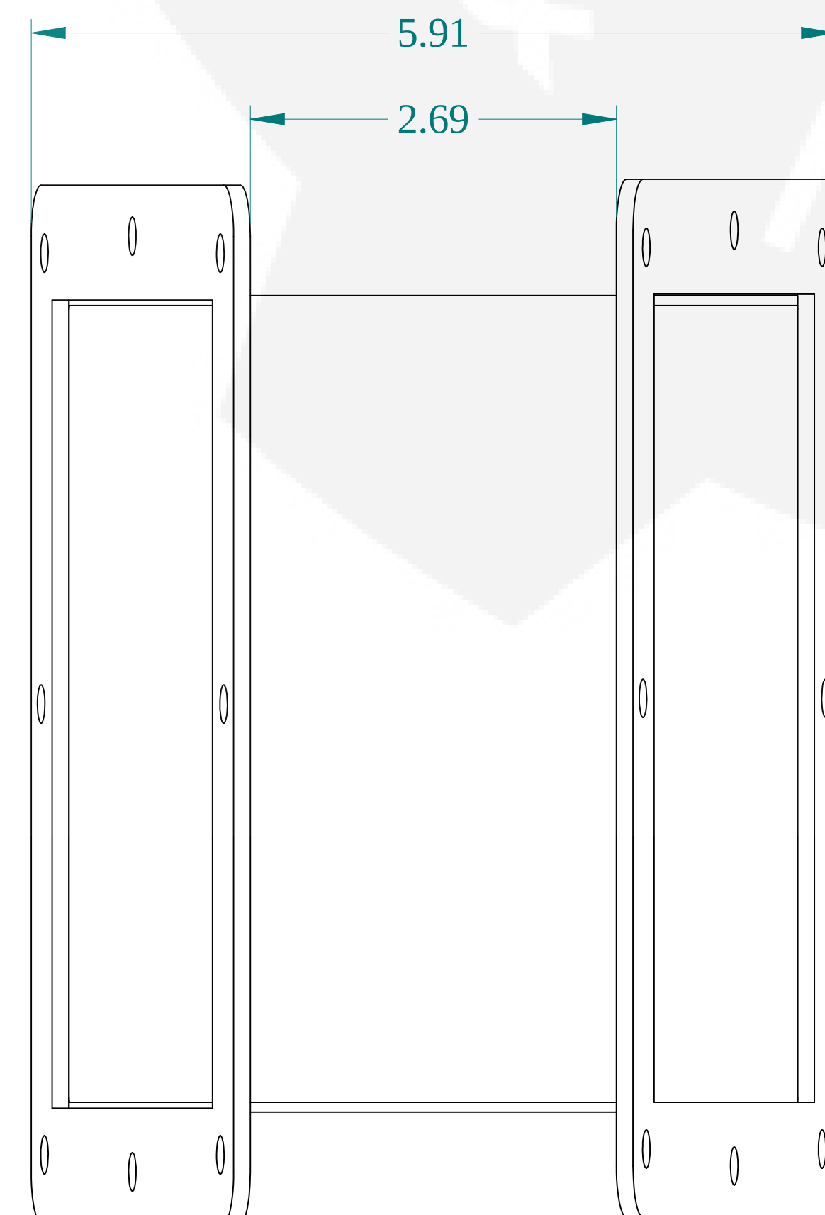
BOTTOM VIEW
