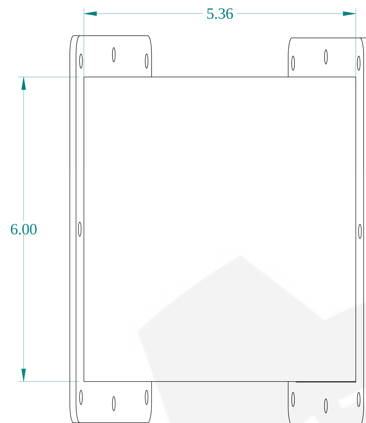
TOP VIEW
