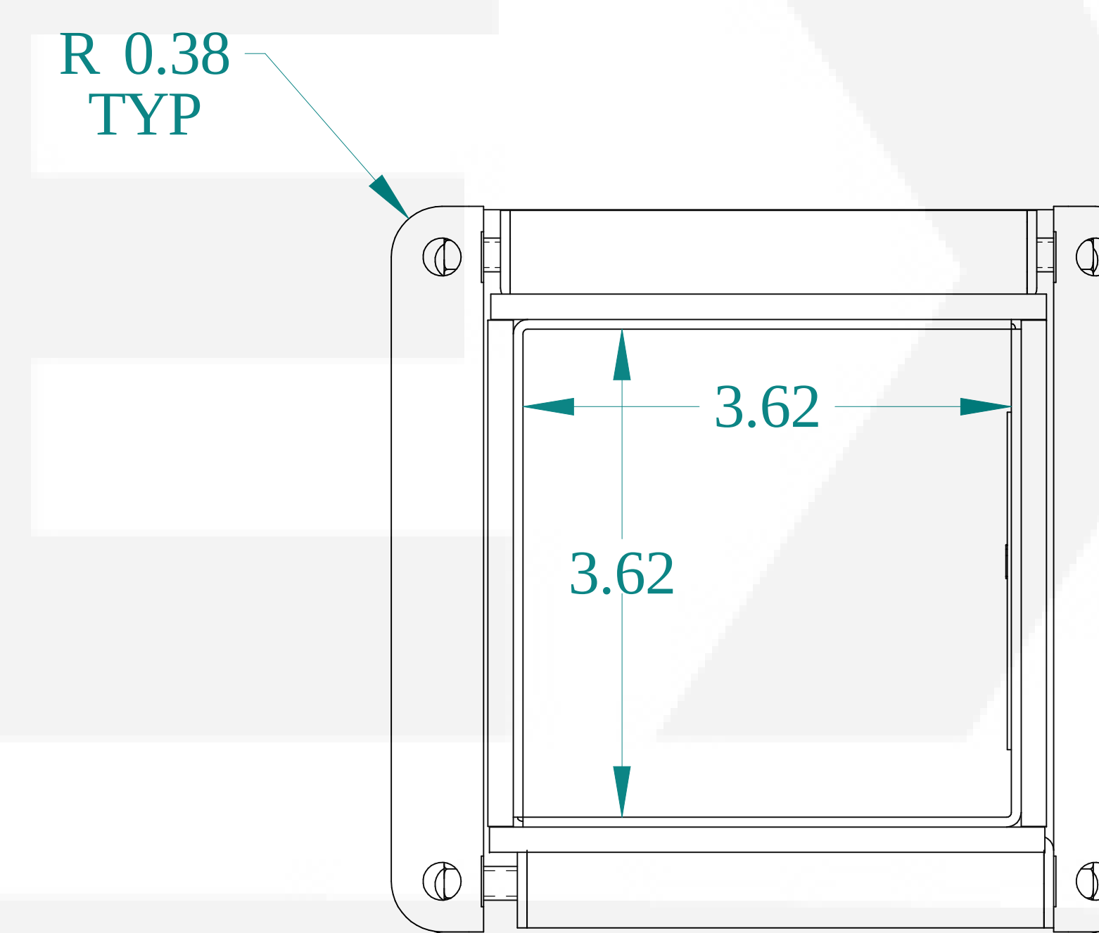
SIDE VIEW
