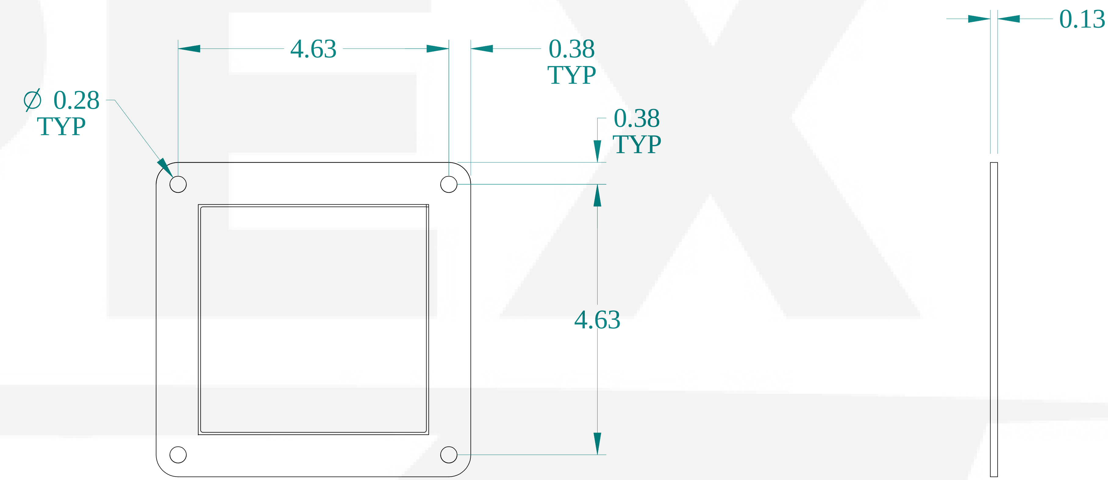
SIDE VIEW
