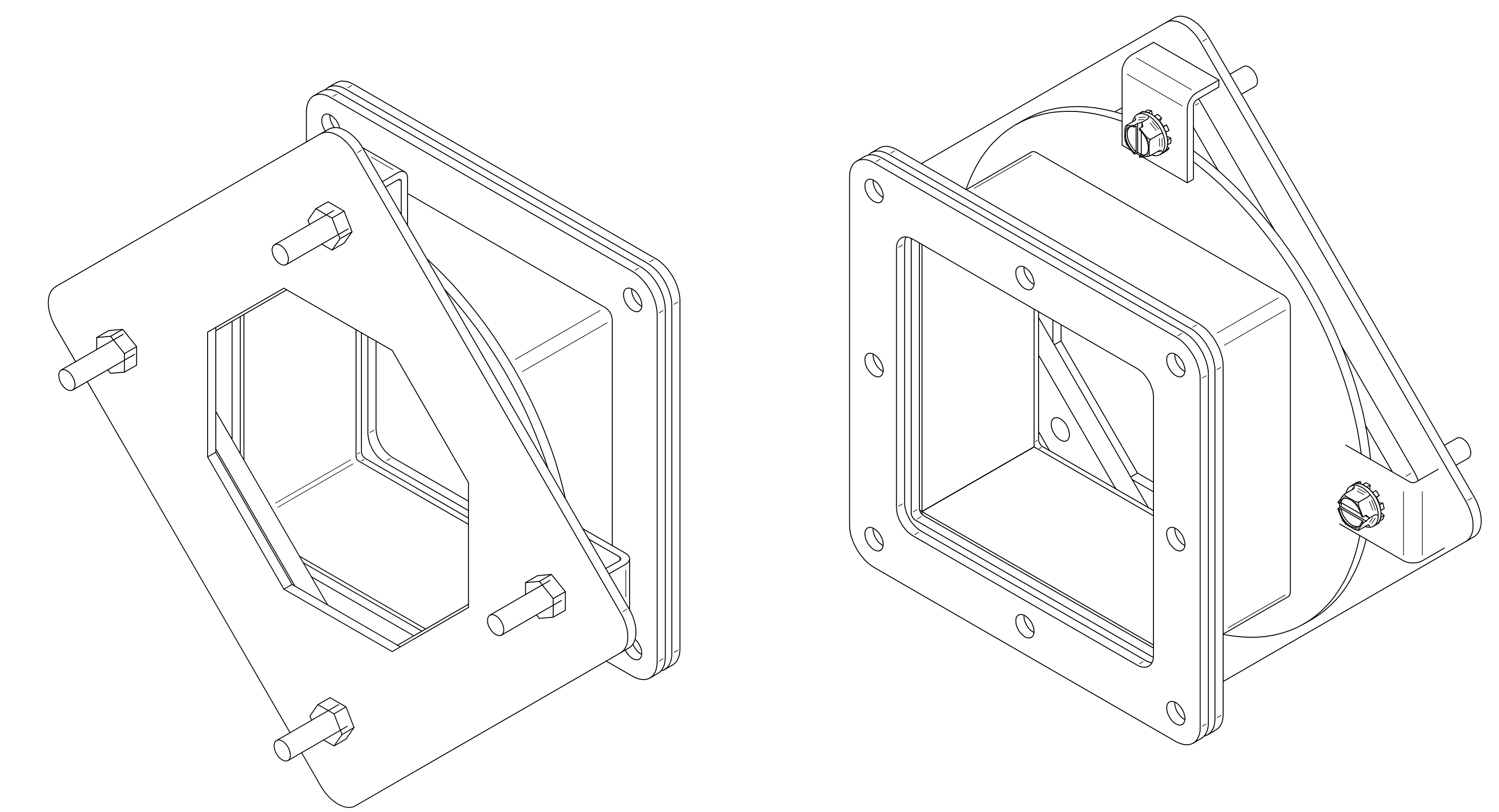
ISOMETRIC VIEWS
