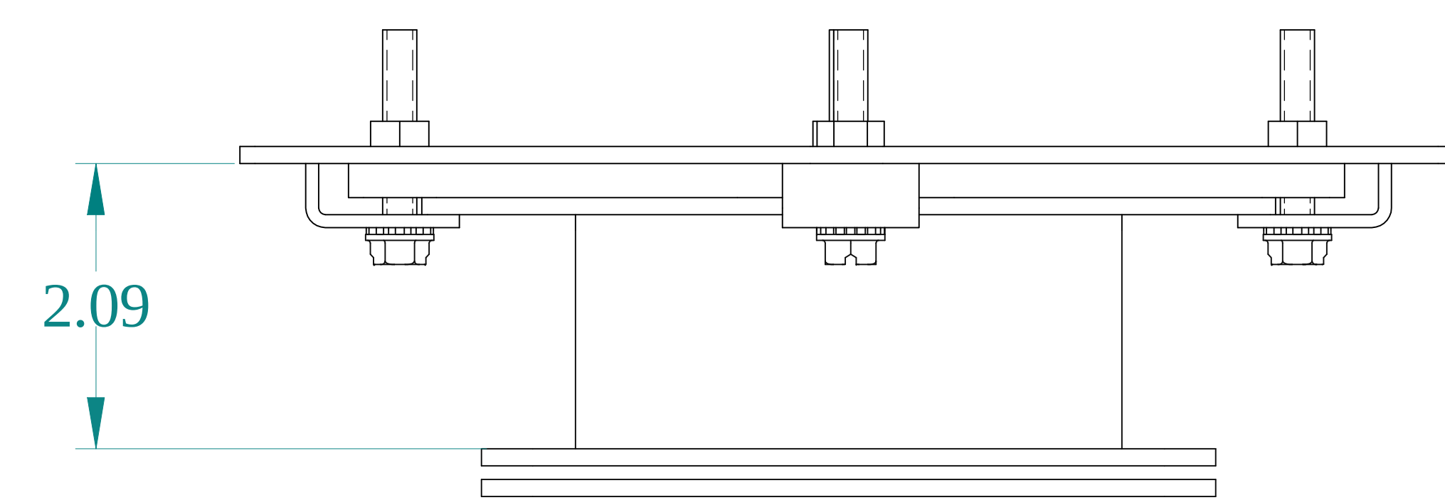
TOP VIEW
