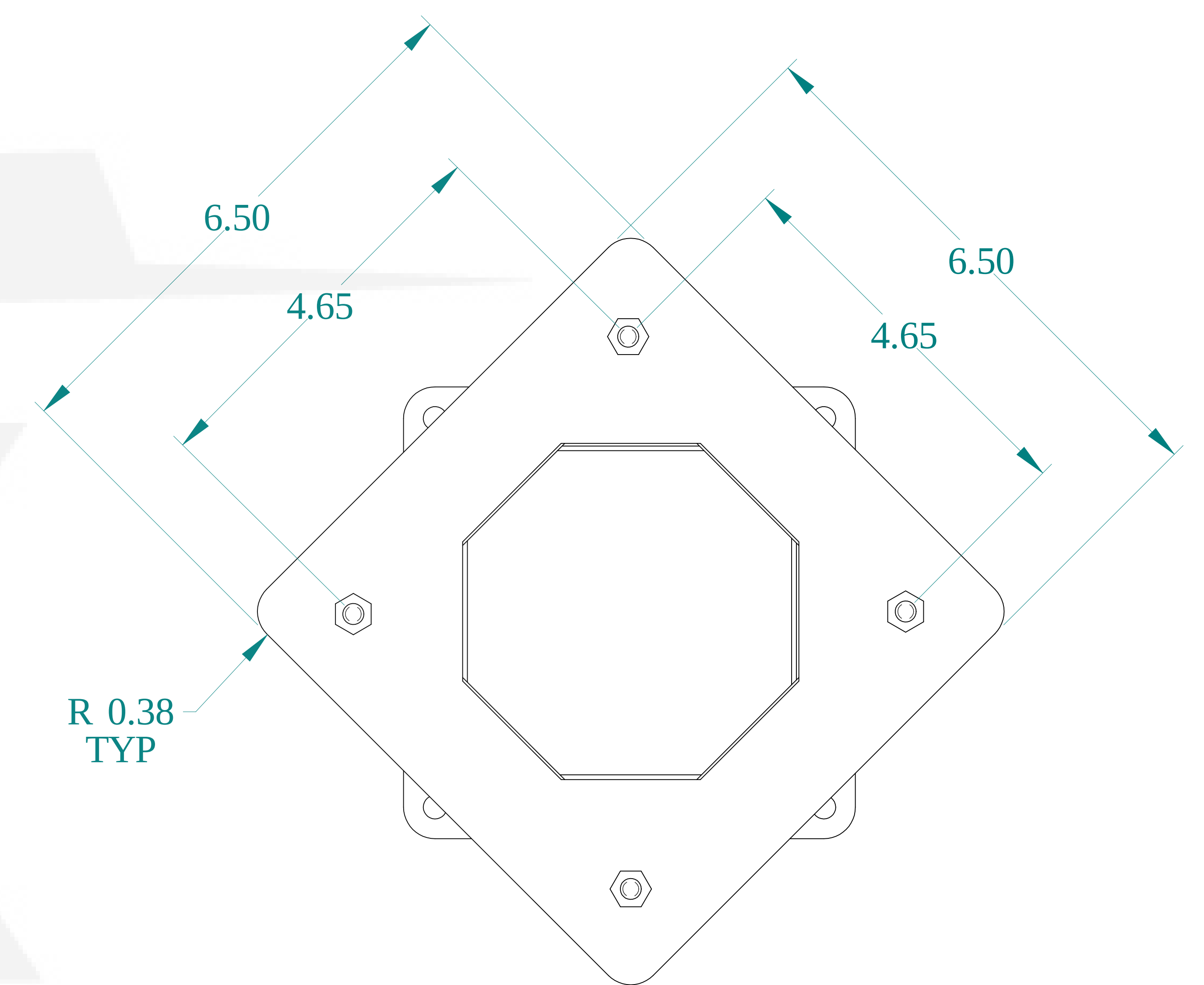
BACK VIEW
