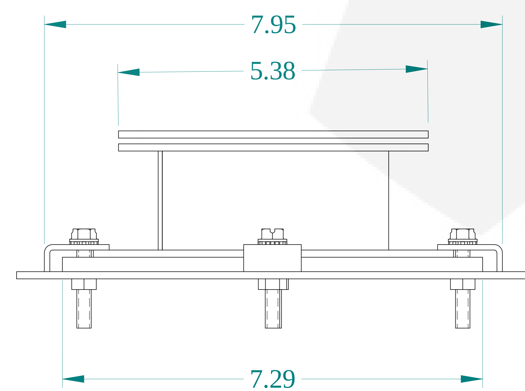
BOTTOM VIEW
