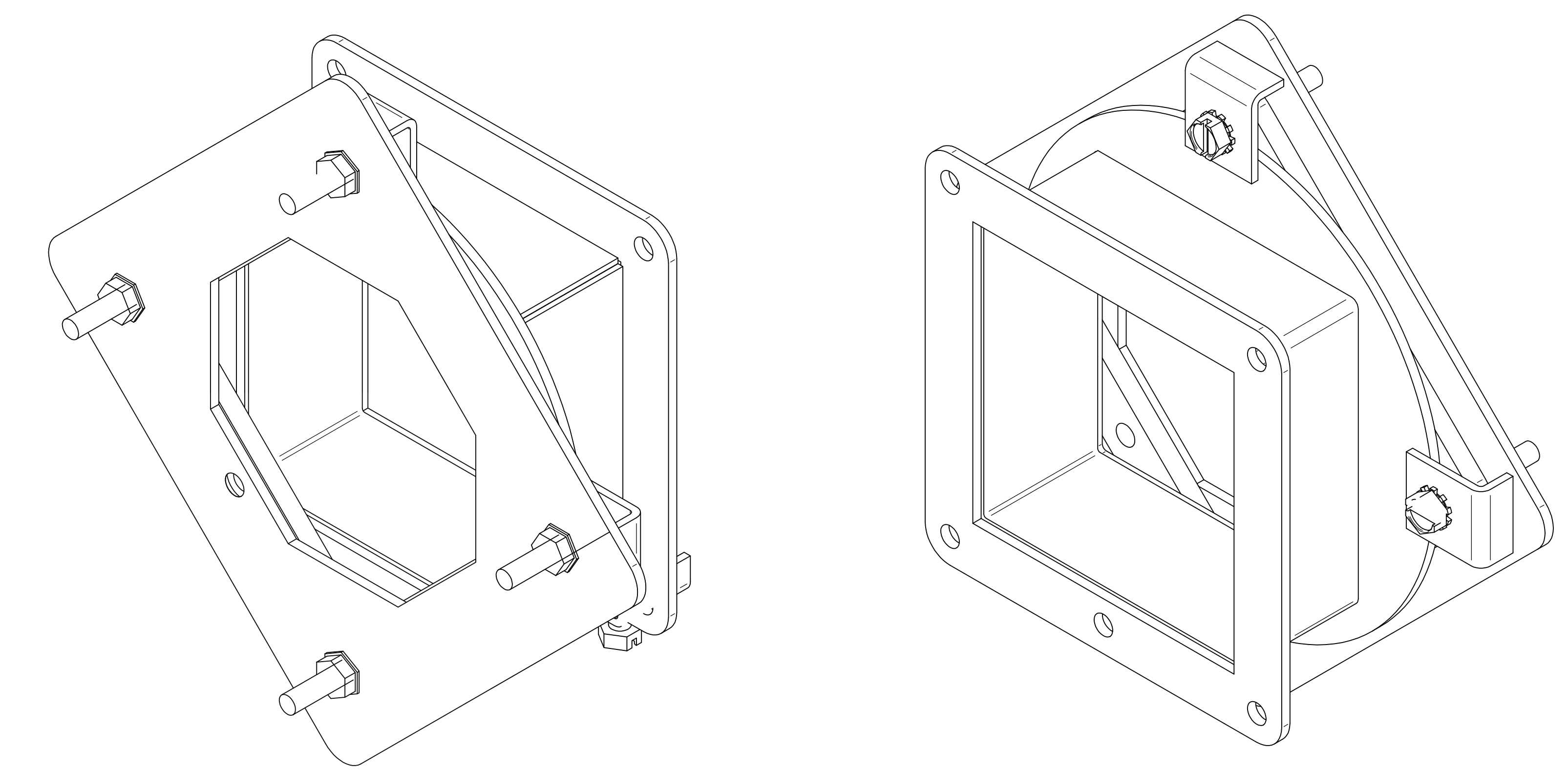
ISOMETRIC VIEWS
