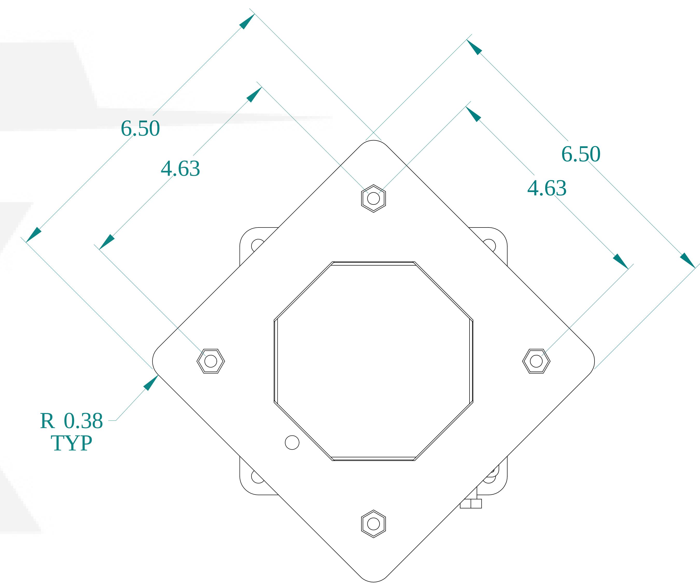
BACK VIEW
