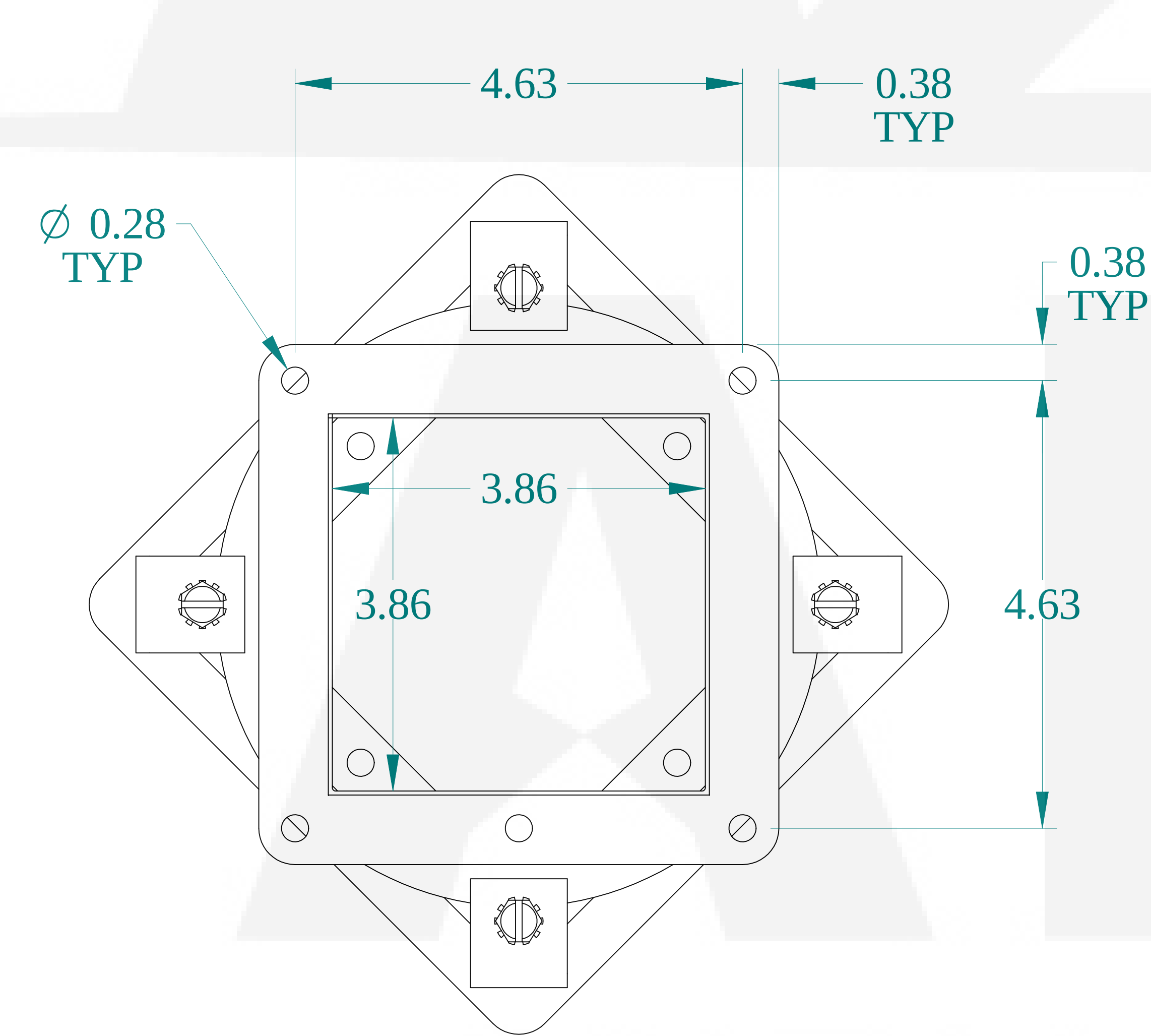
FRONT VIEW
