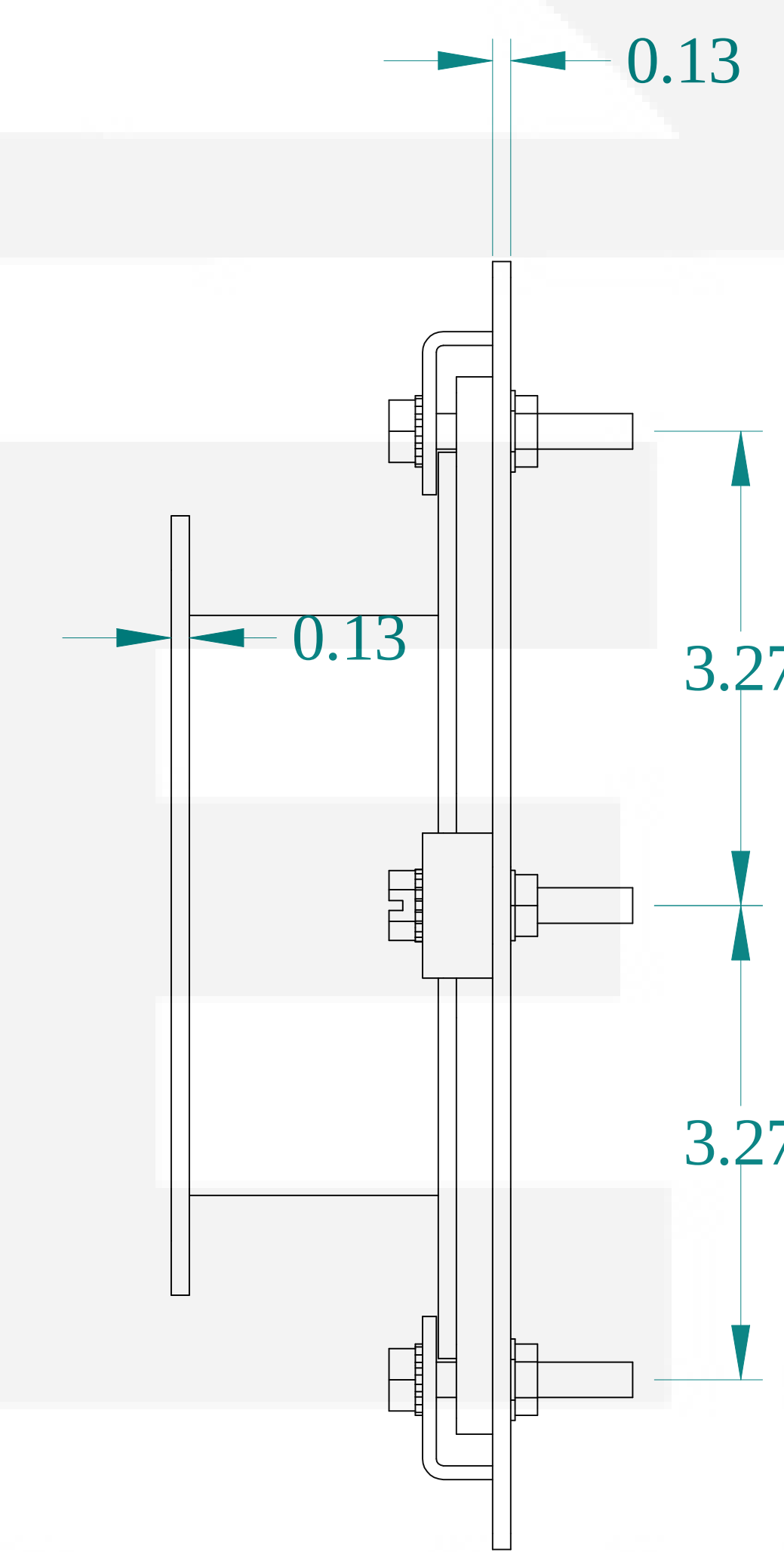
SIDE VIEW
