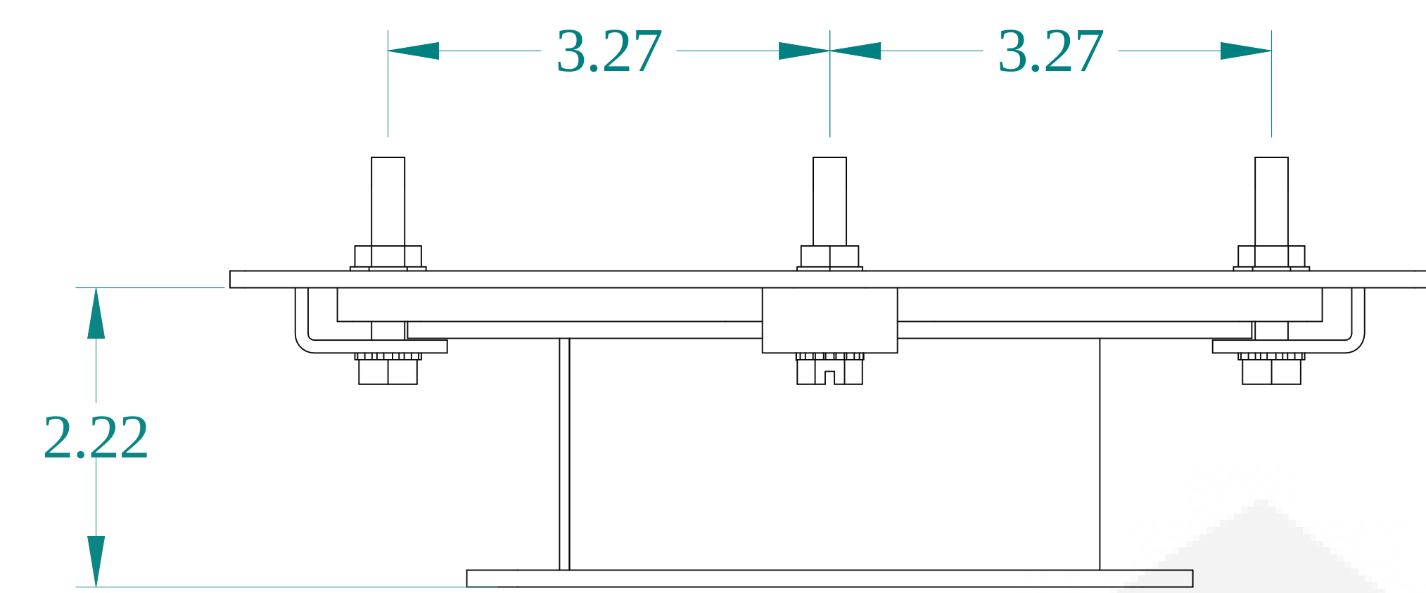
TOP VIEW
