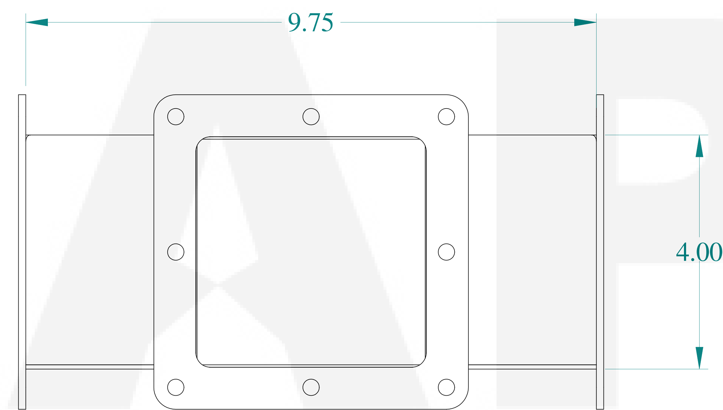
FRONT VIEW
