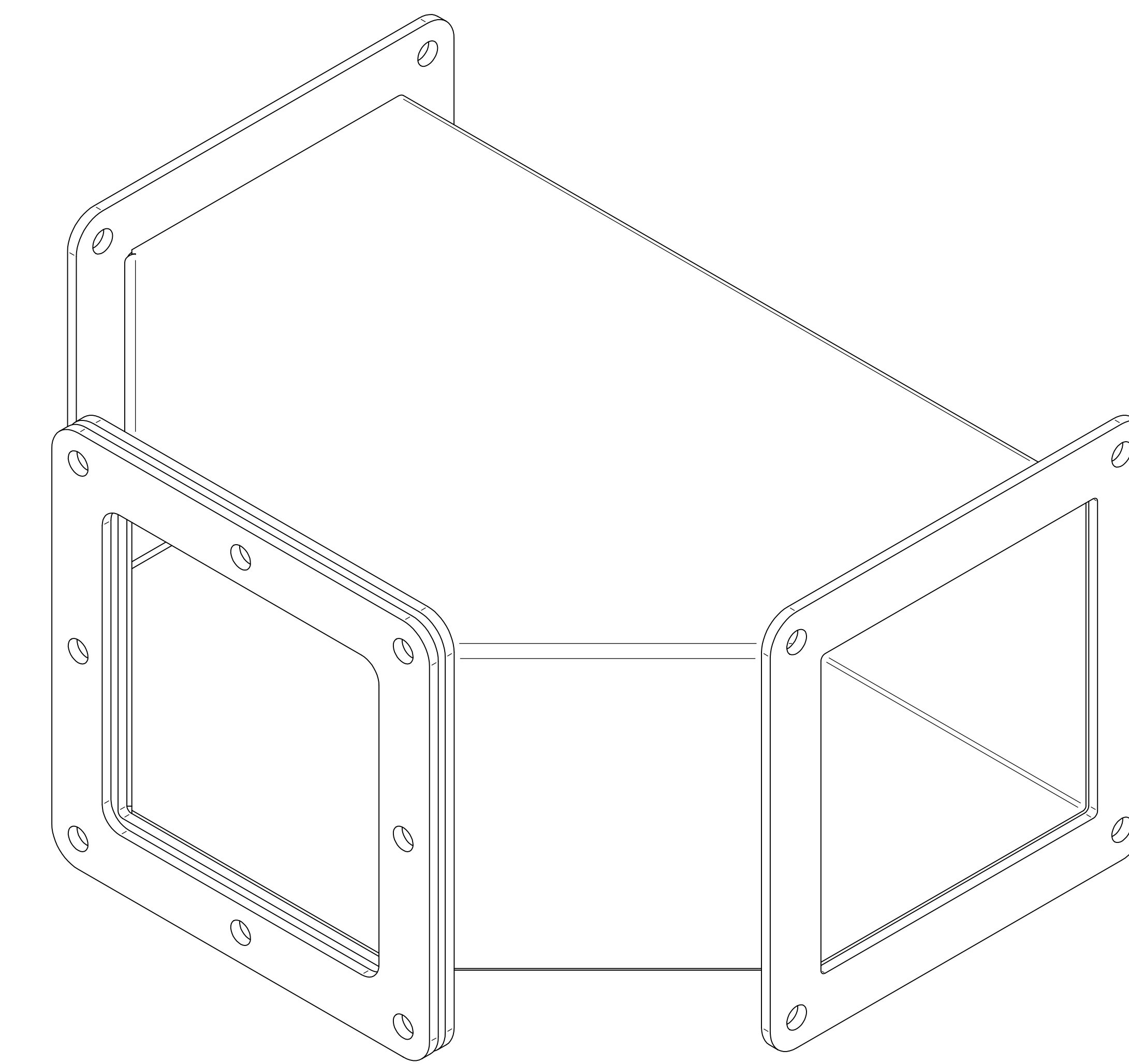
ISOMETRIC VIEWS
