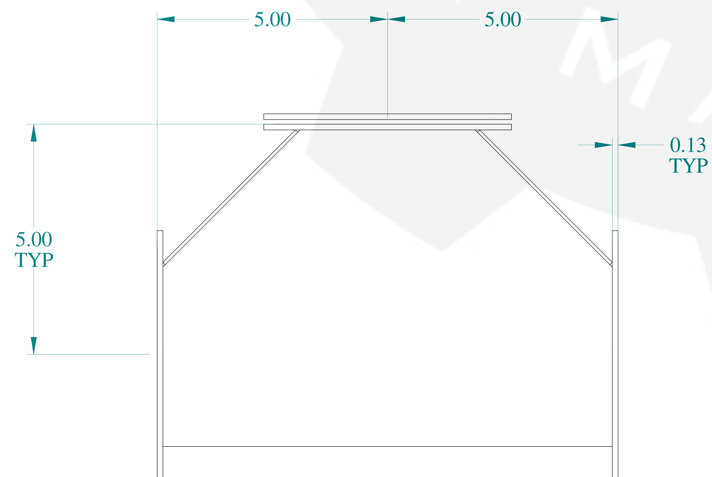
BOTTOM VIEW
