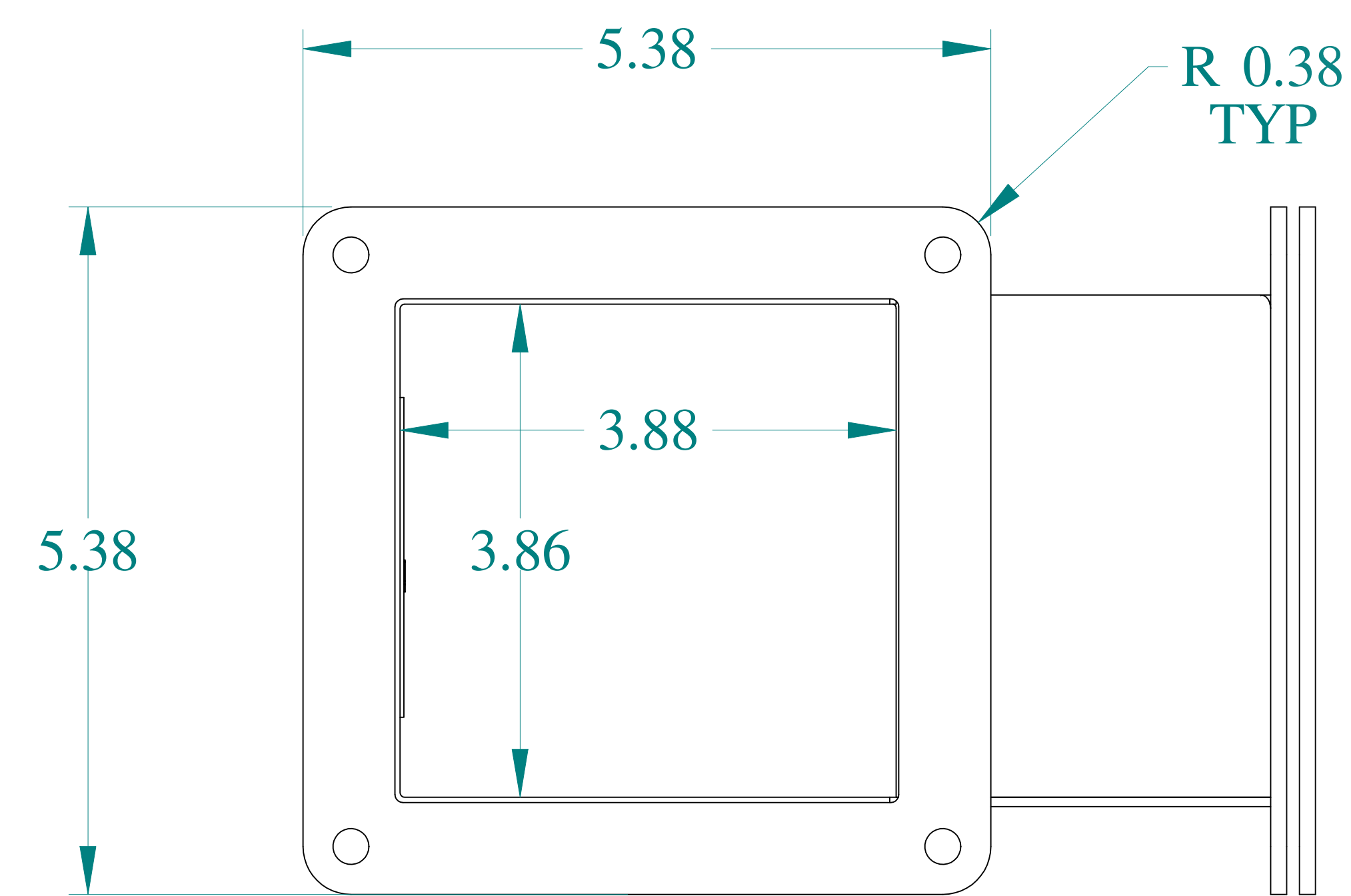
SIDE VIEW
