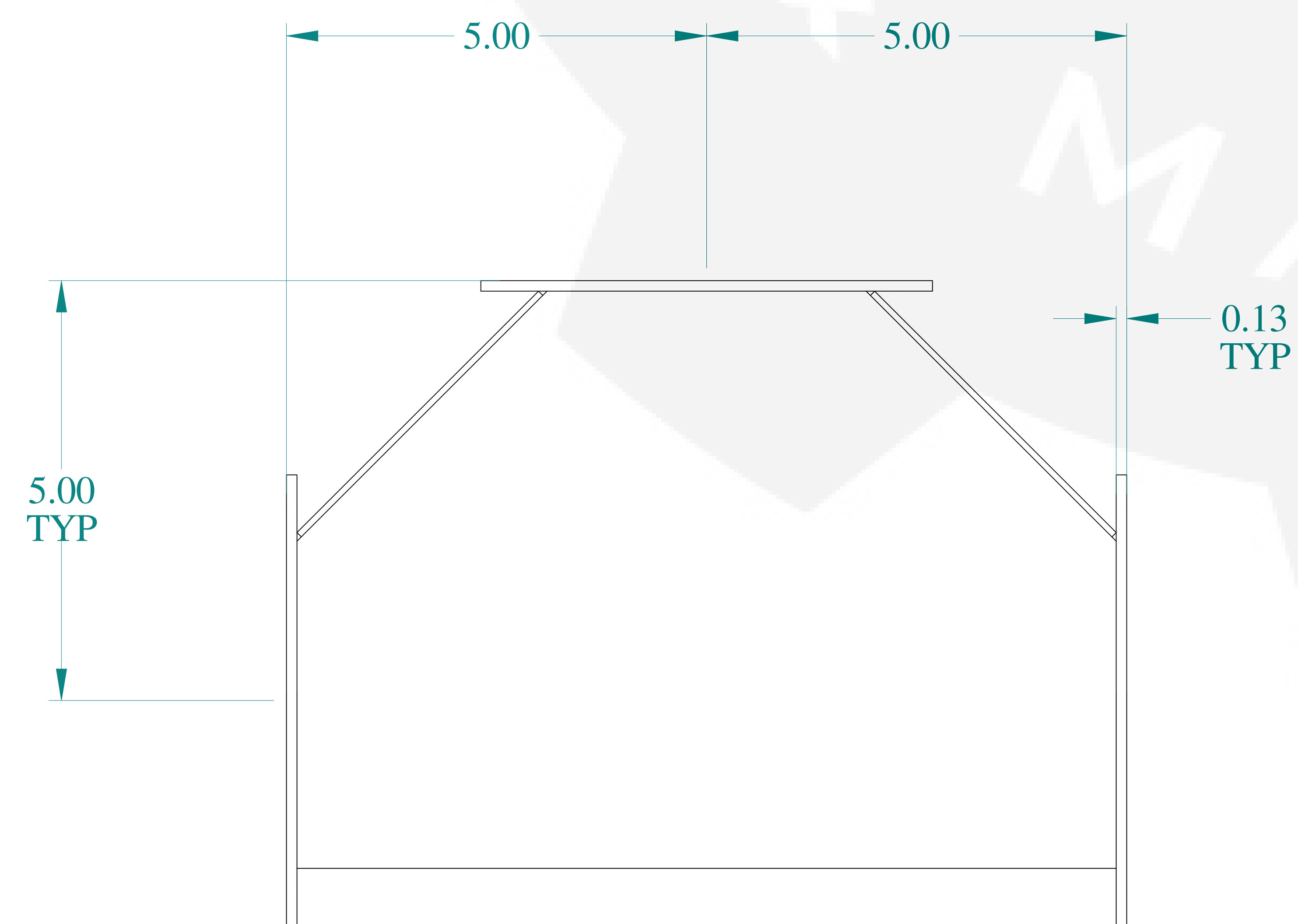
BOTTOM VIEW
