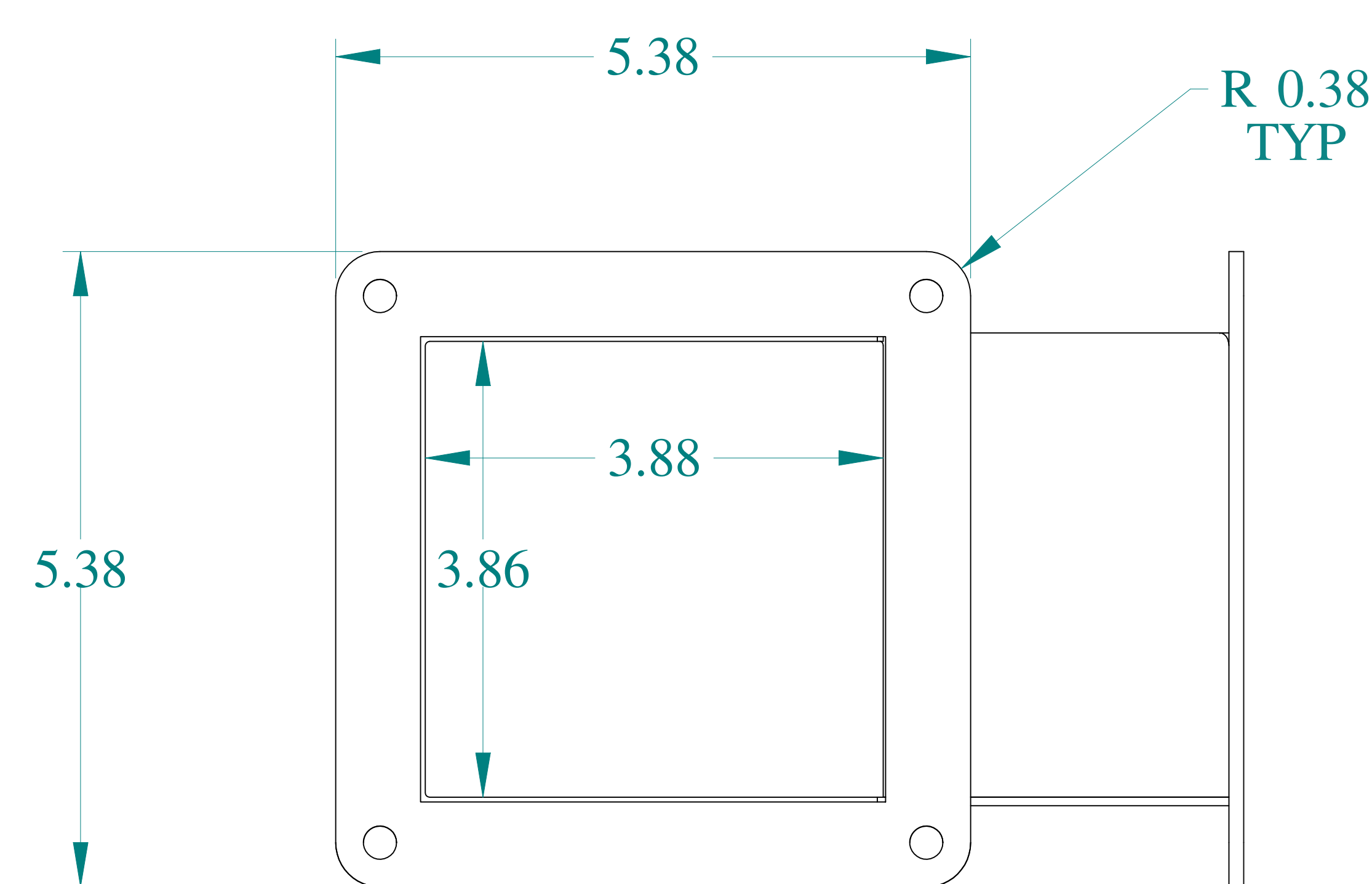
SIDE VIEW
