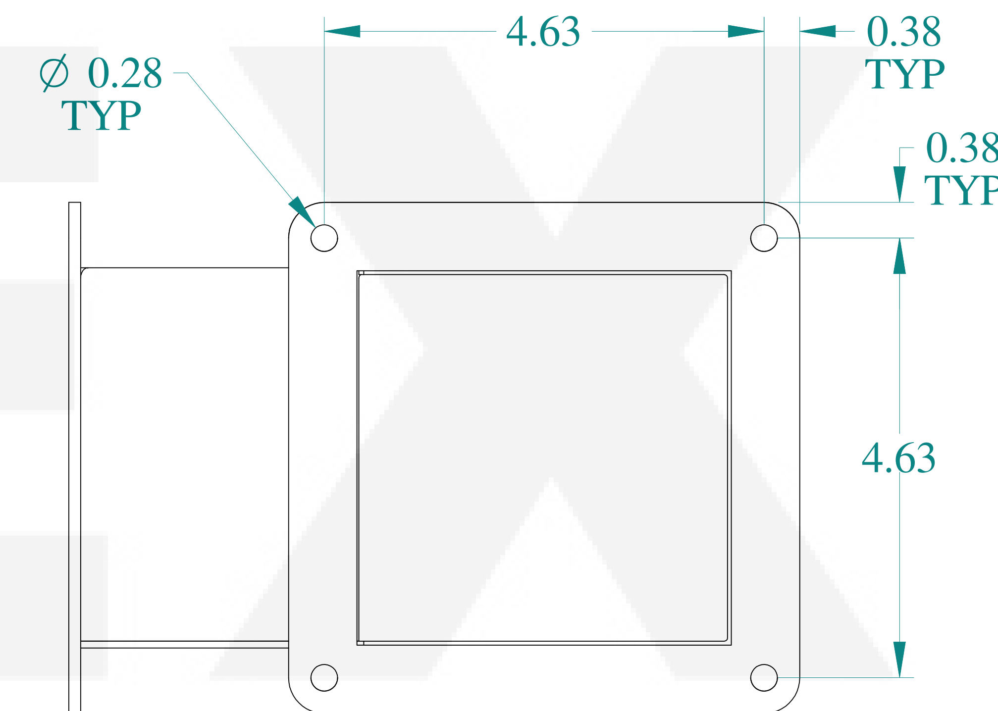
SIDE VIEW
