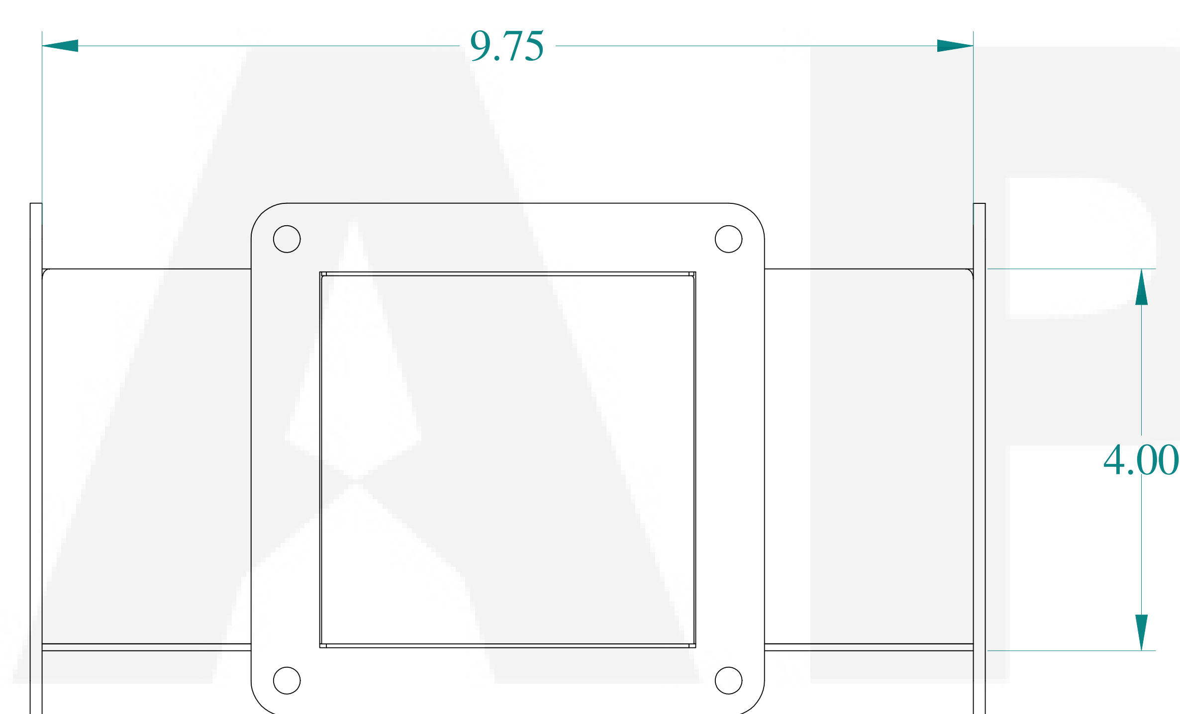
FRONT VIEW
