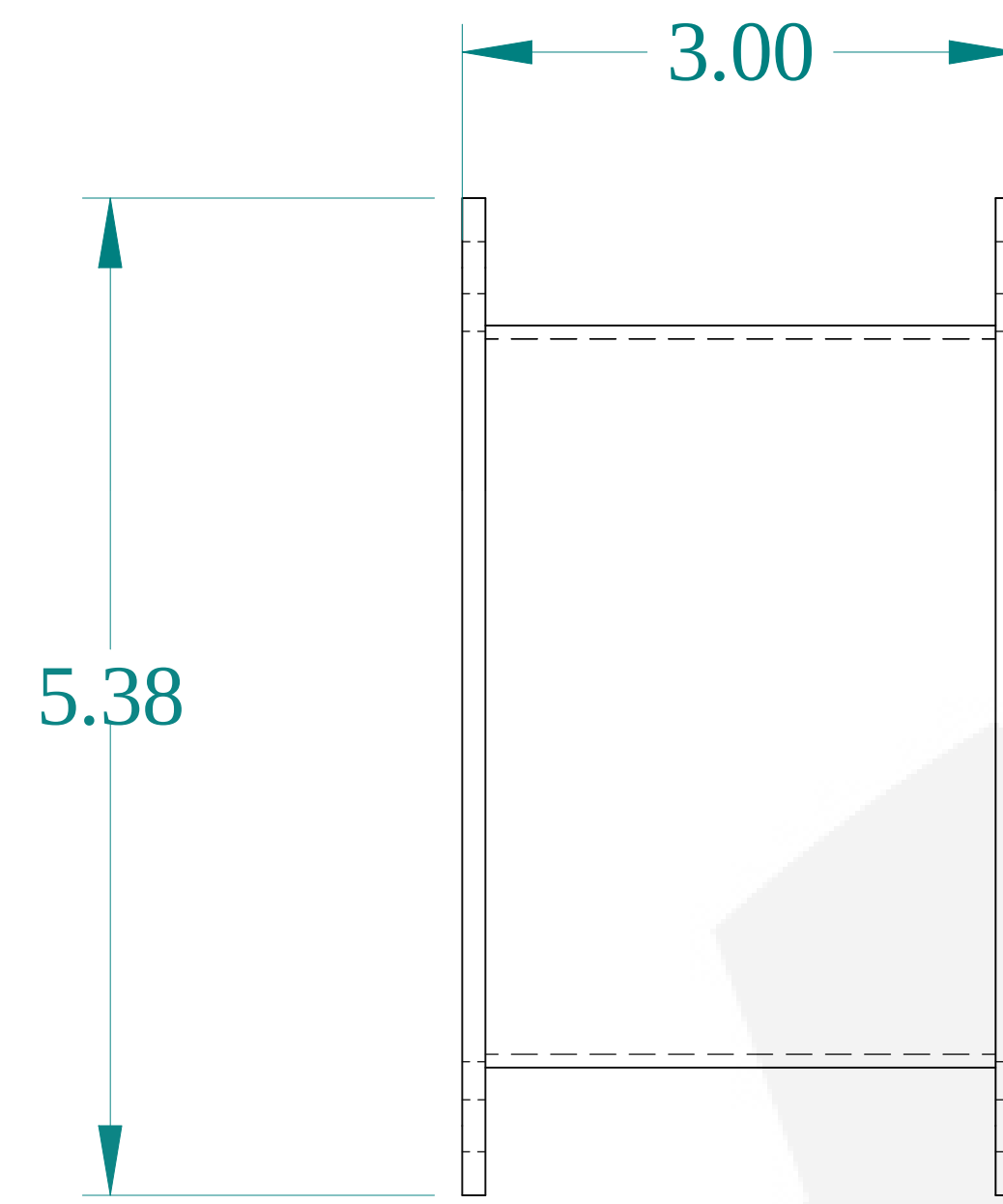
TOP VIEW
