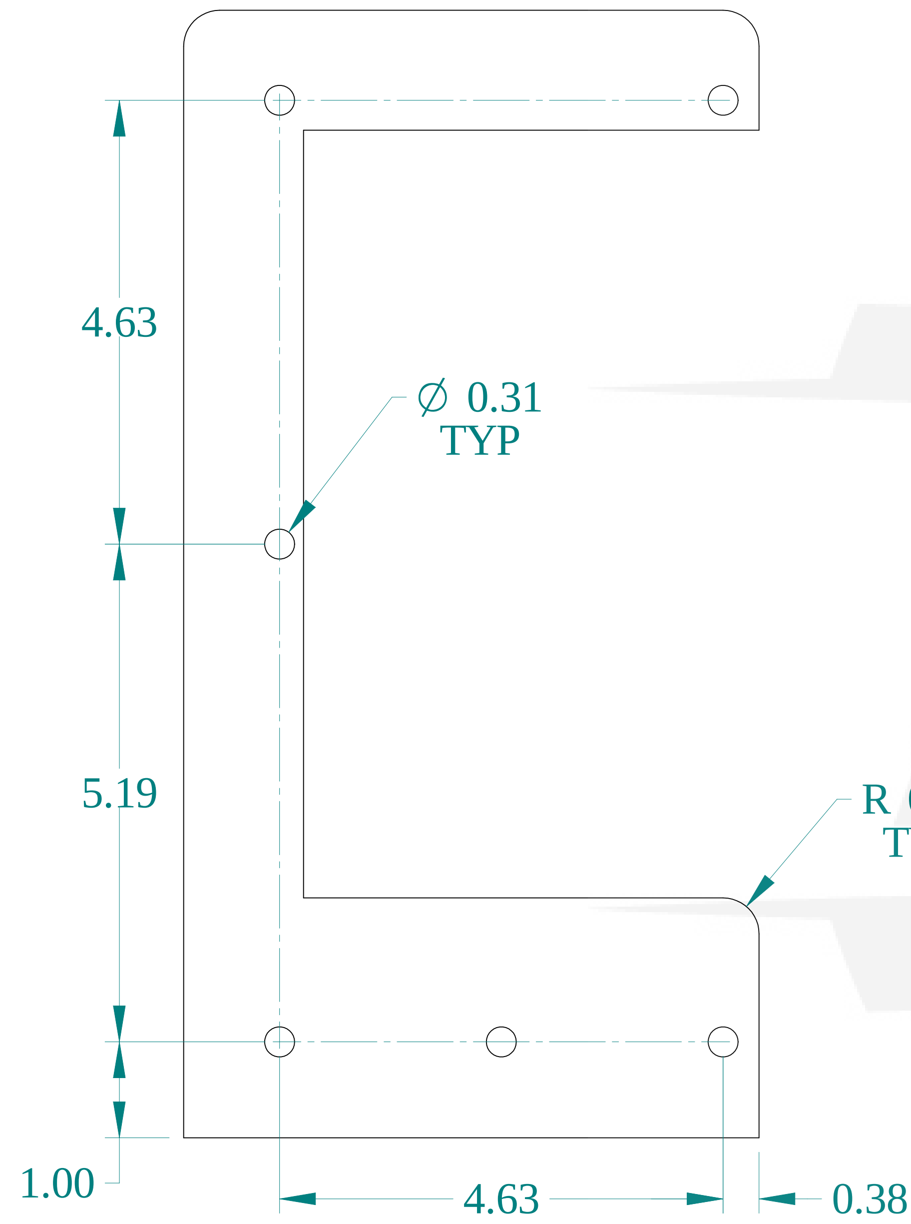
FRONT VIEW
