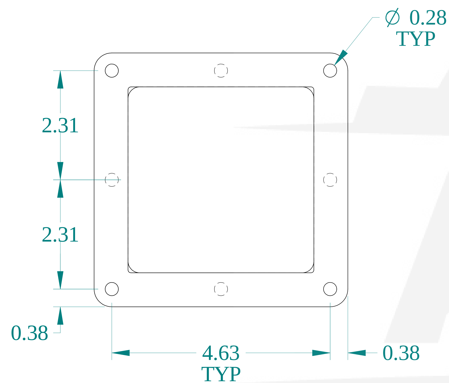
FRONT VIEW
