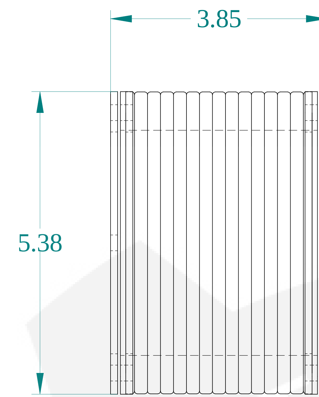
TOP VIEW
