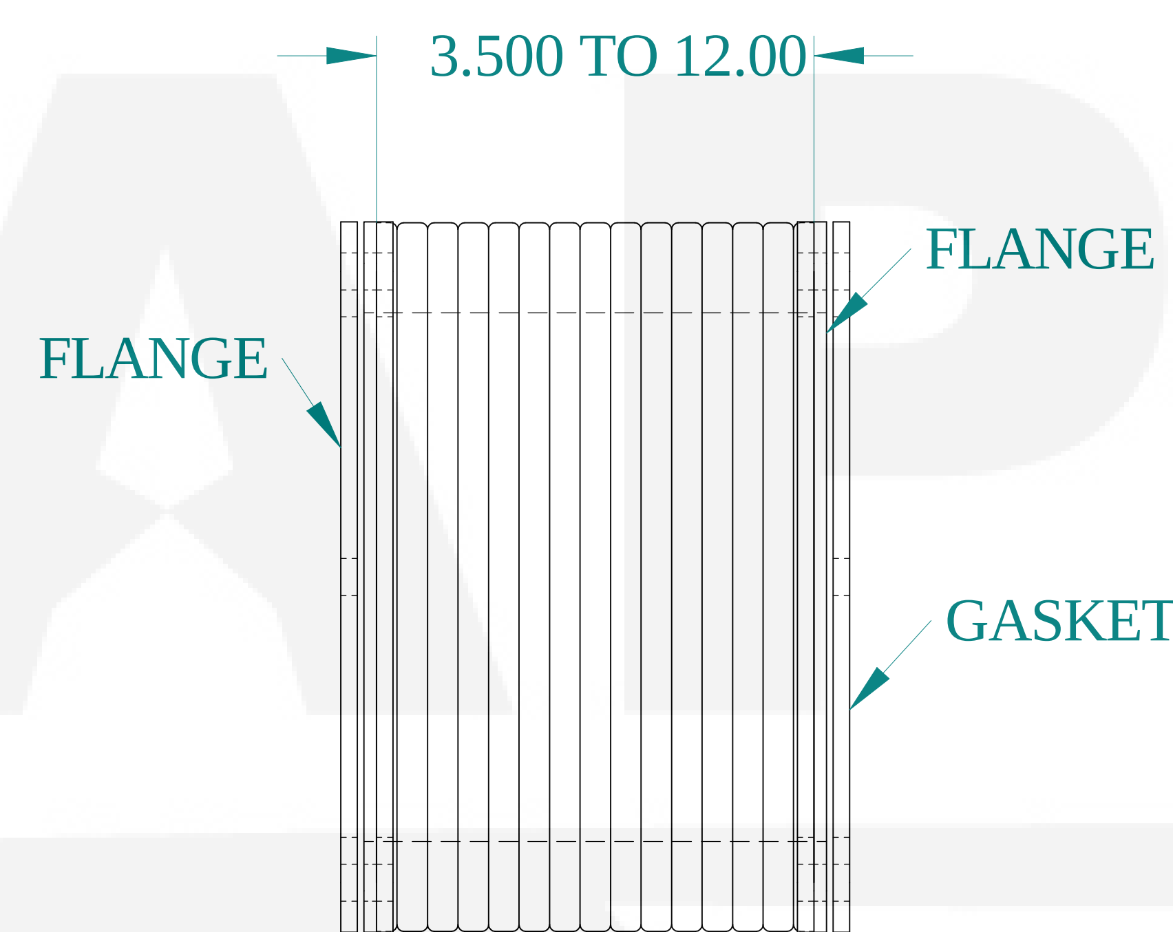
FRONT VIEW
