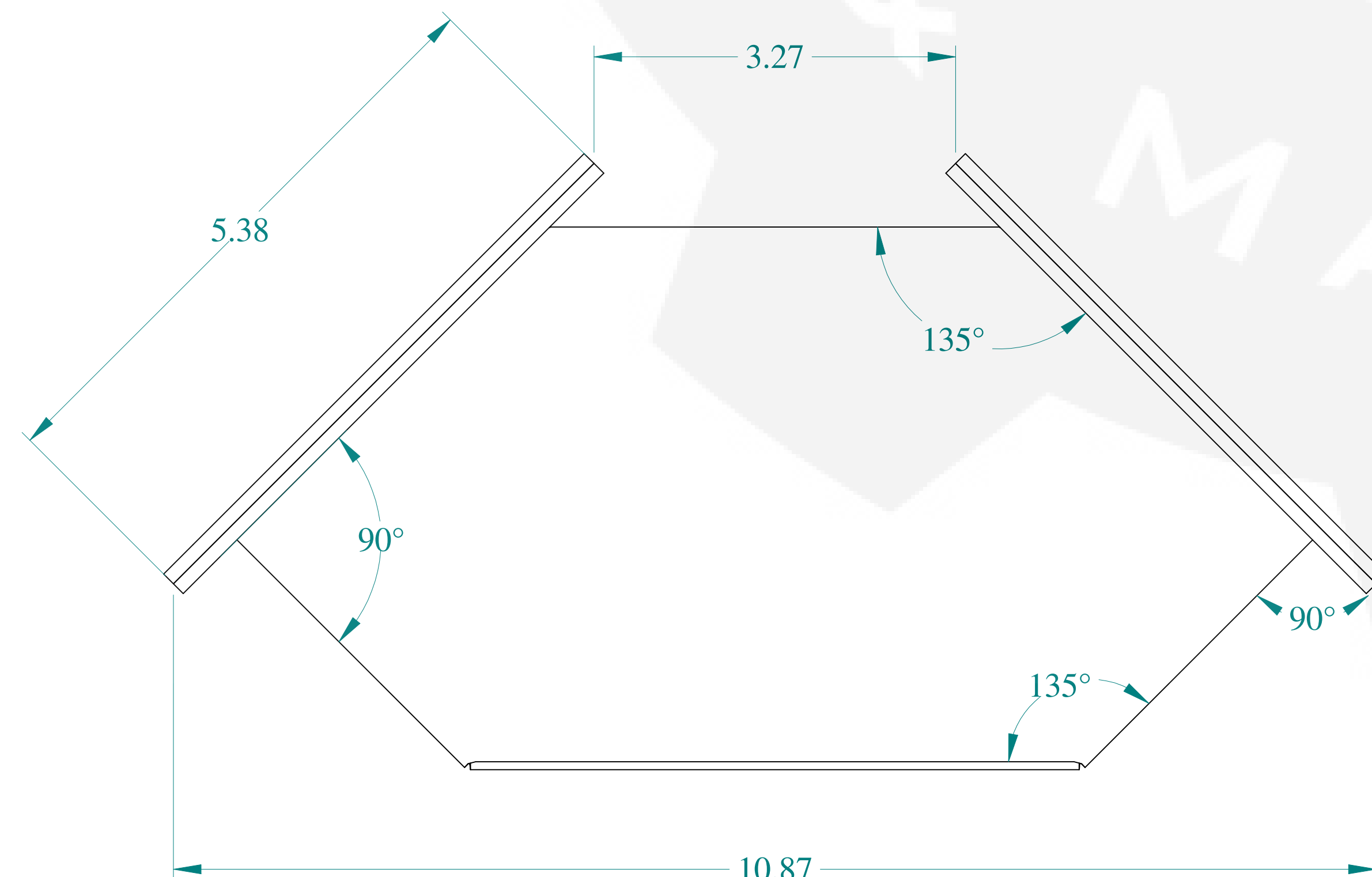
BOTTOM VIEW
