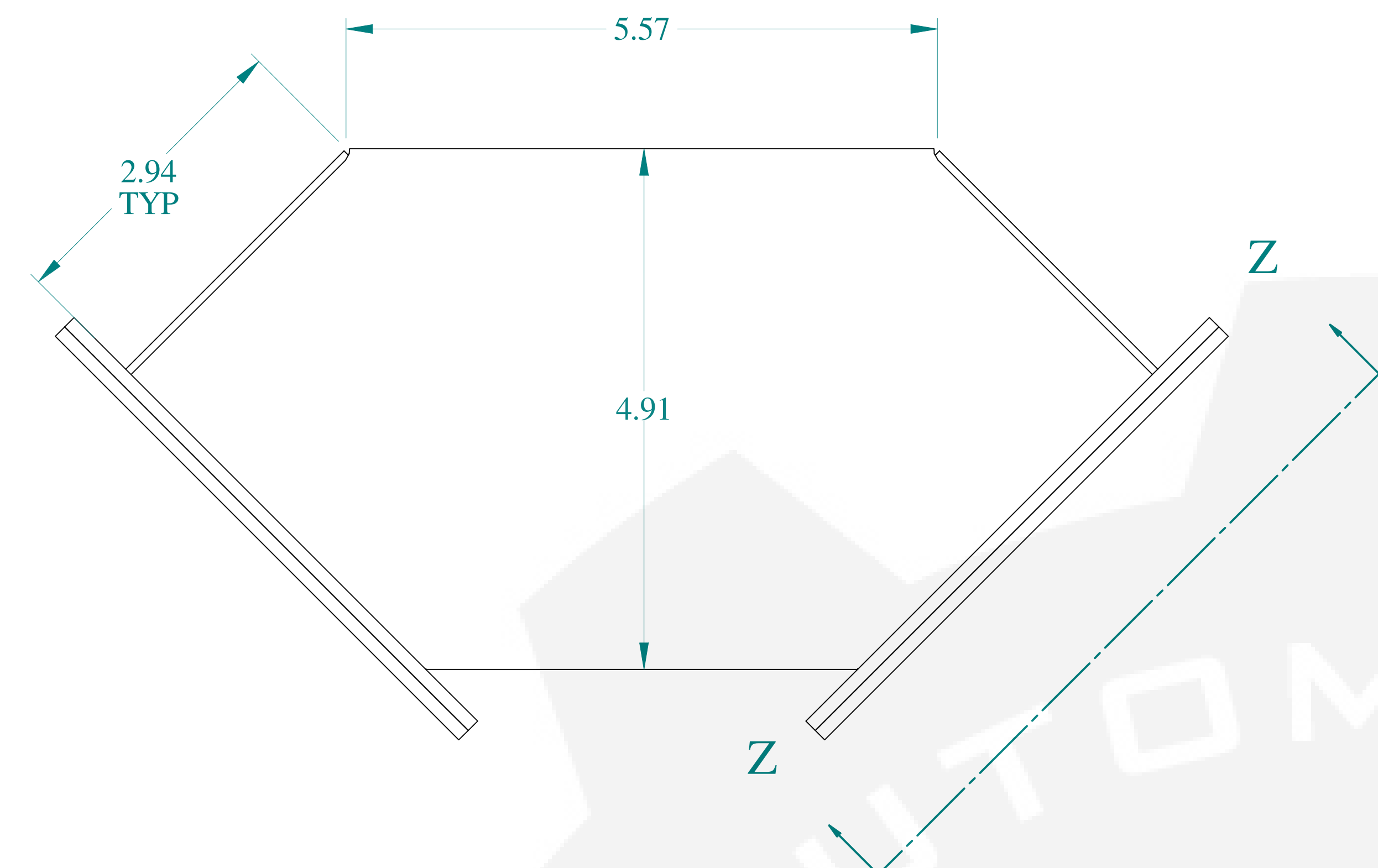
TOP VIEW
