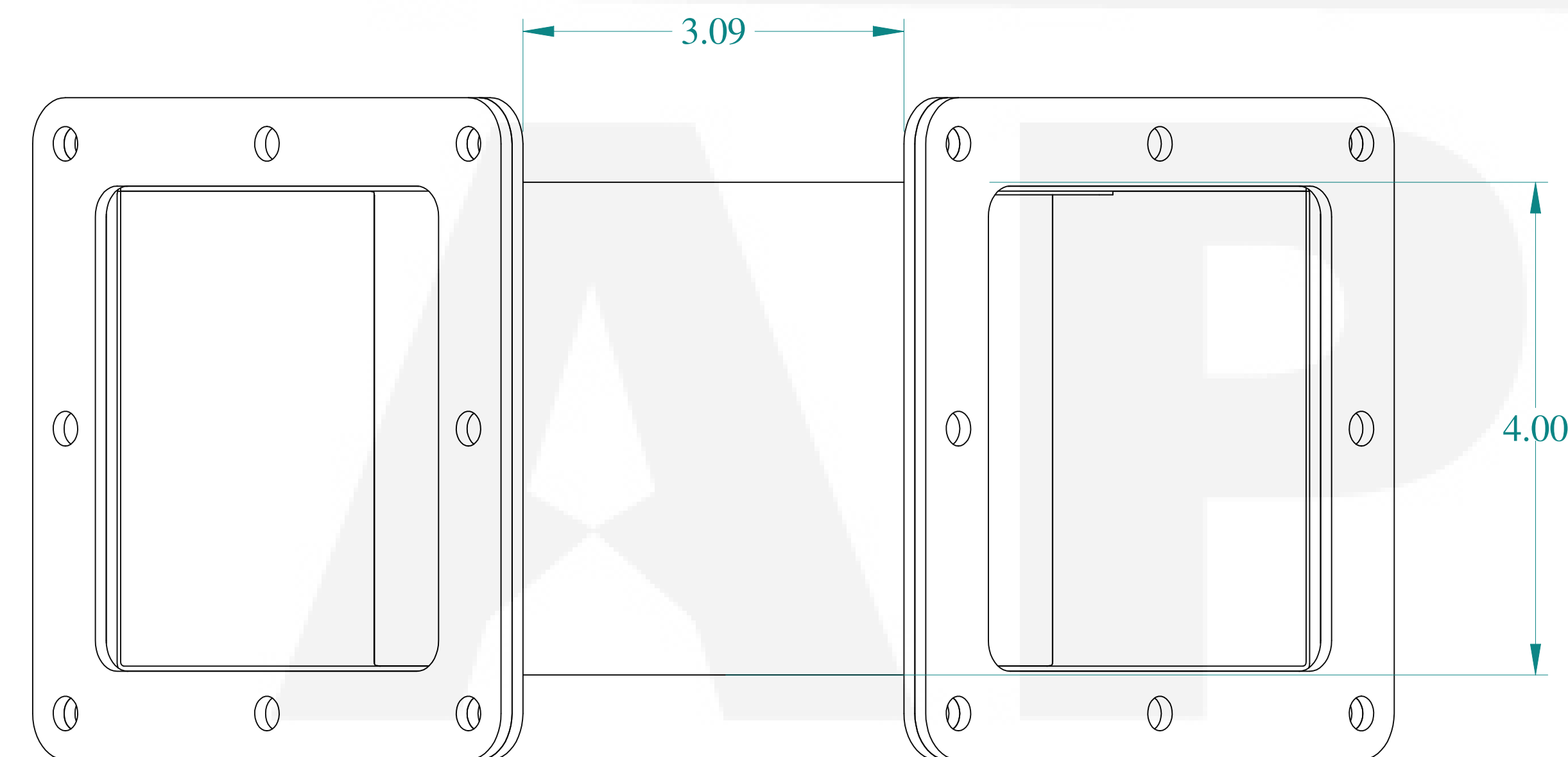
FRONT VIEW
