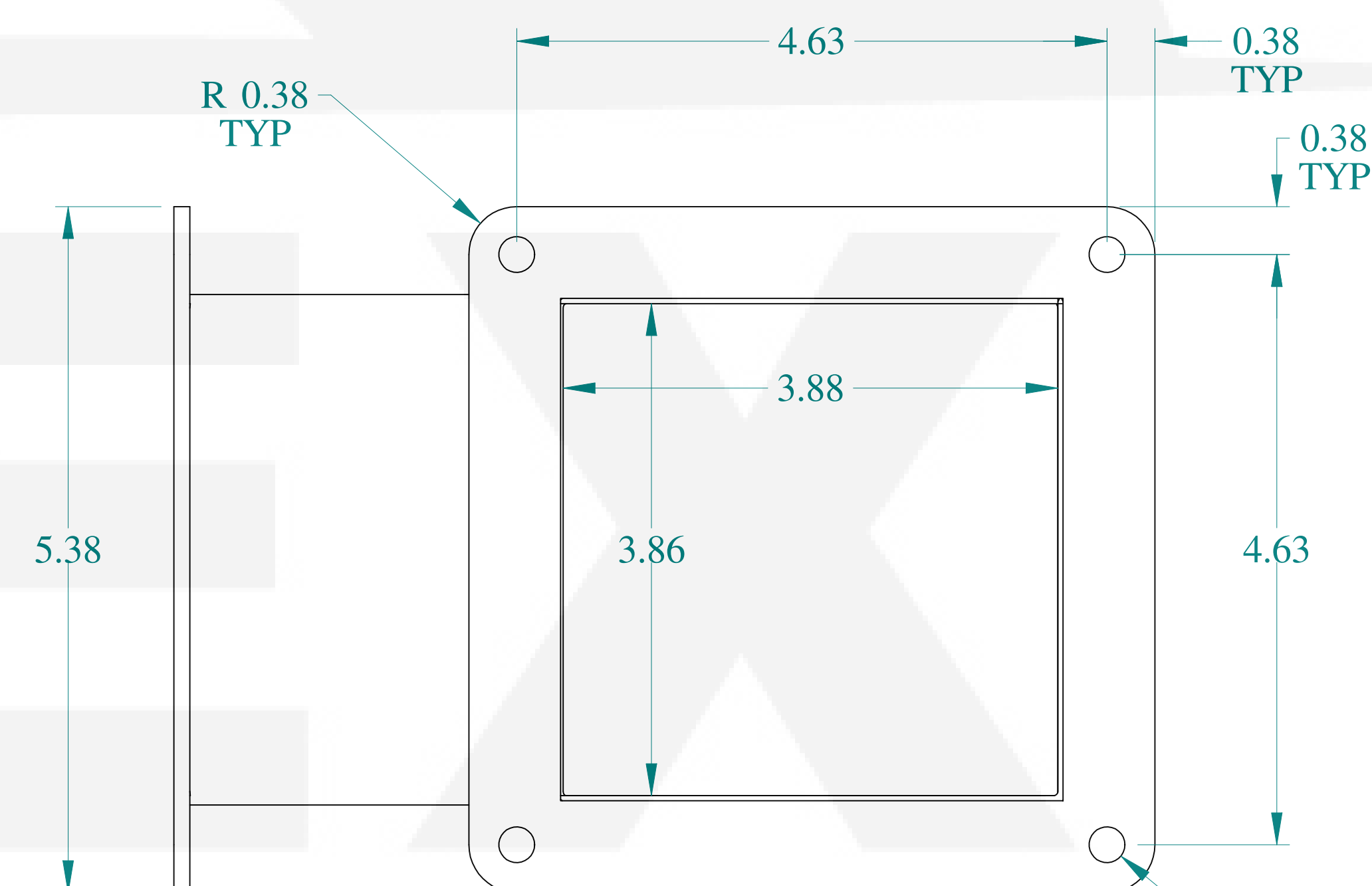
VIEW Z-Z
