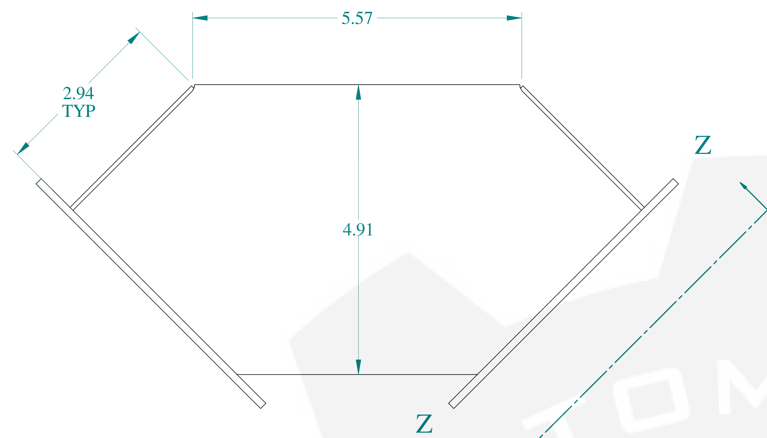
TOP VIEW
