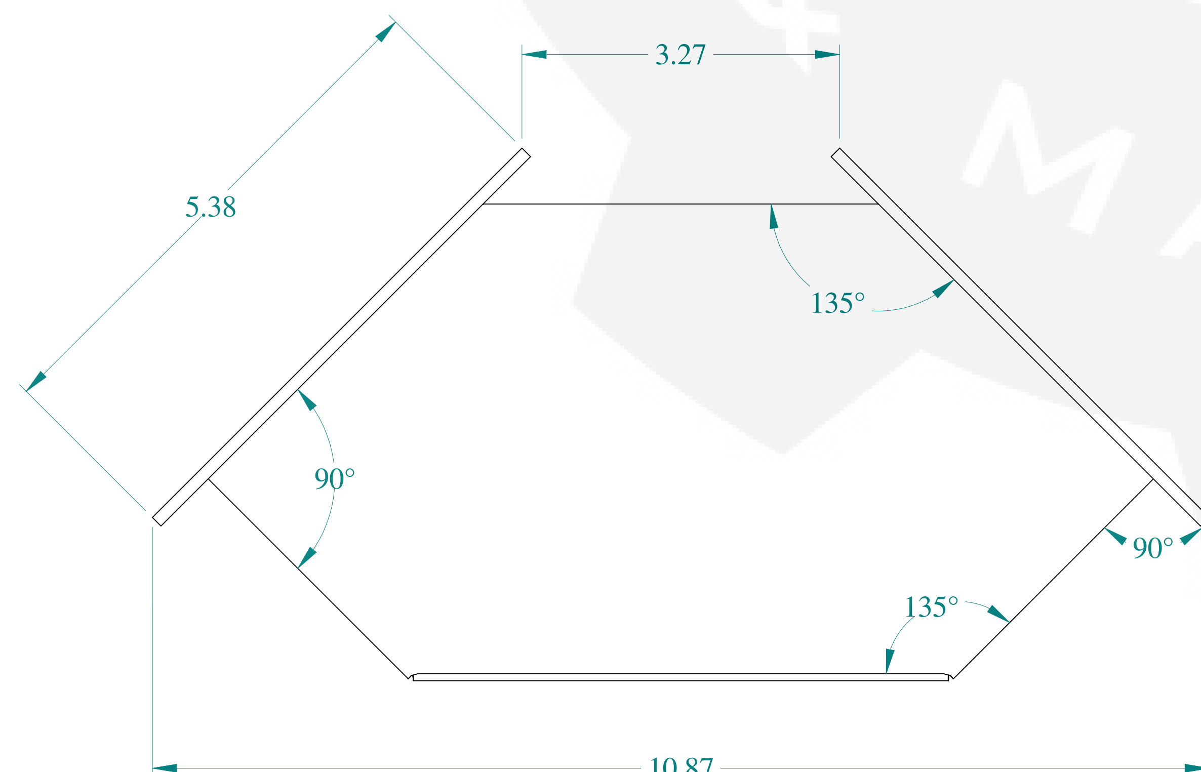
BOTTOM VIEW
