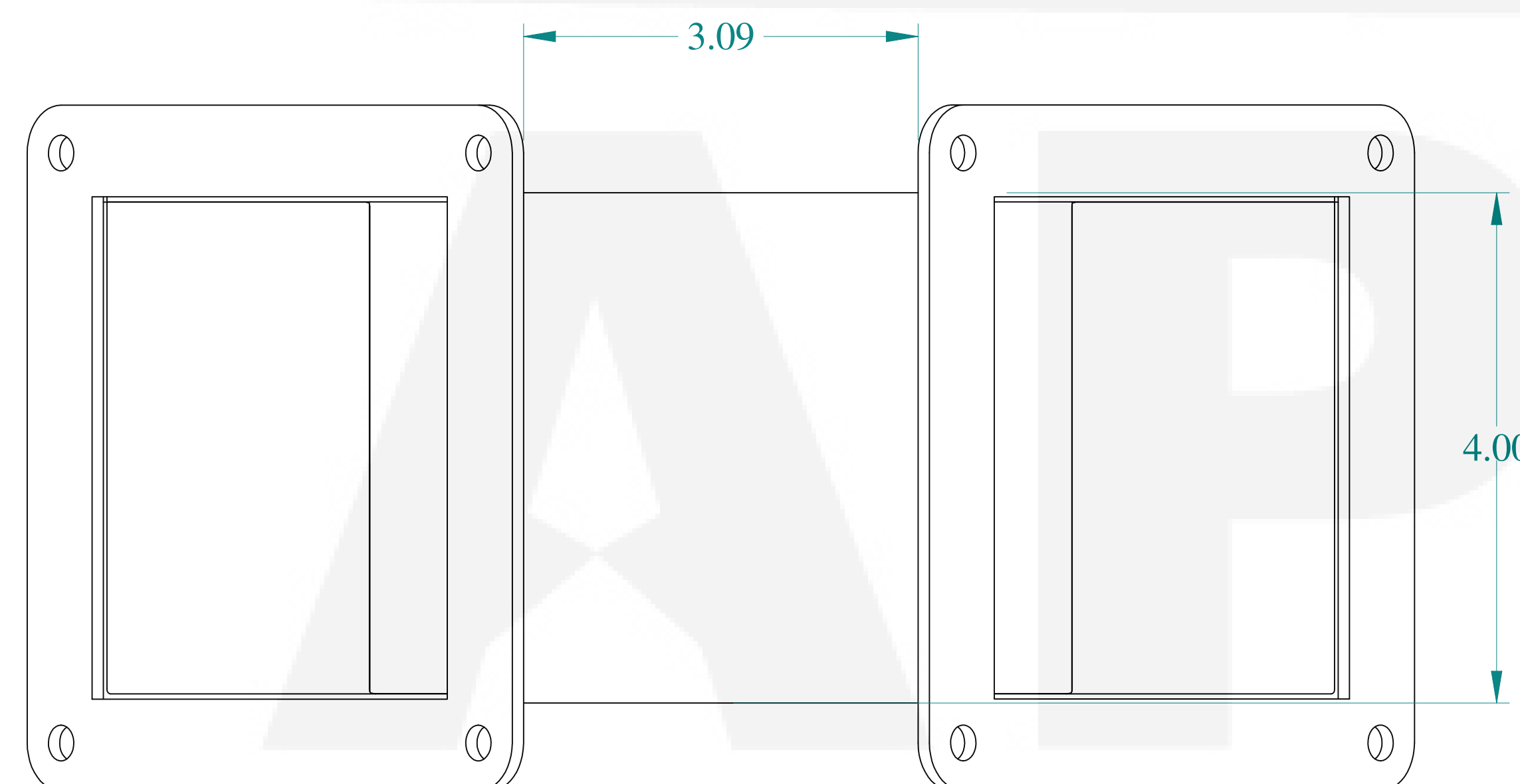
FRONT VIEW
