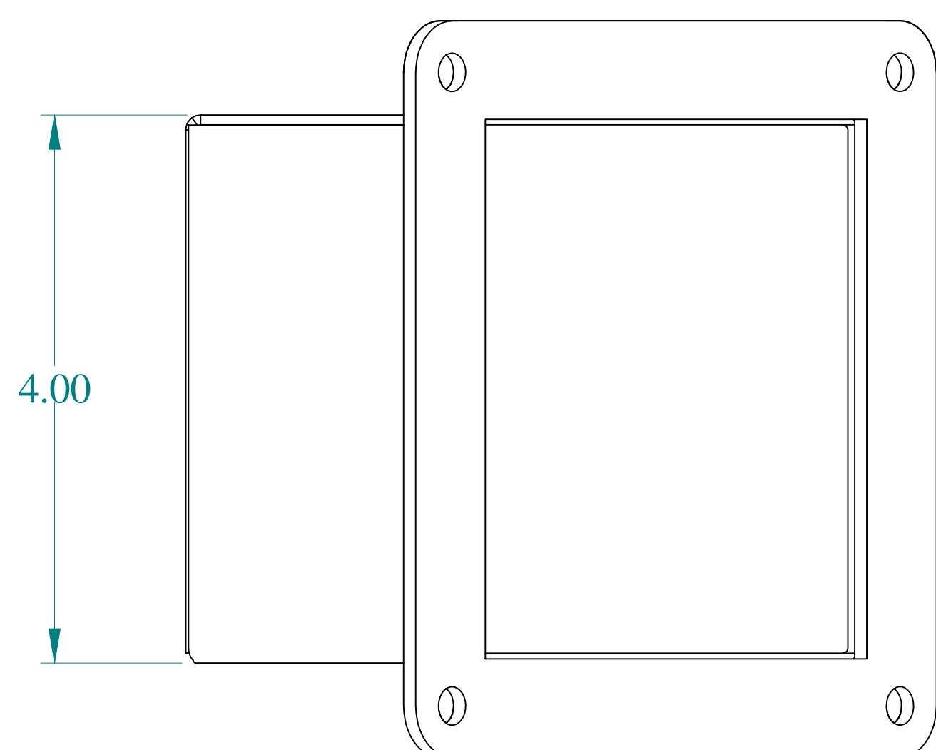
SIDE VIEW
