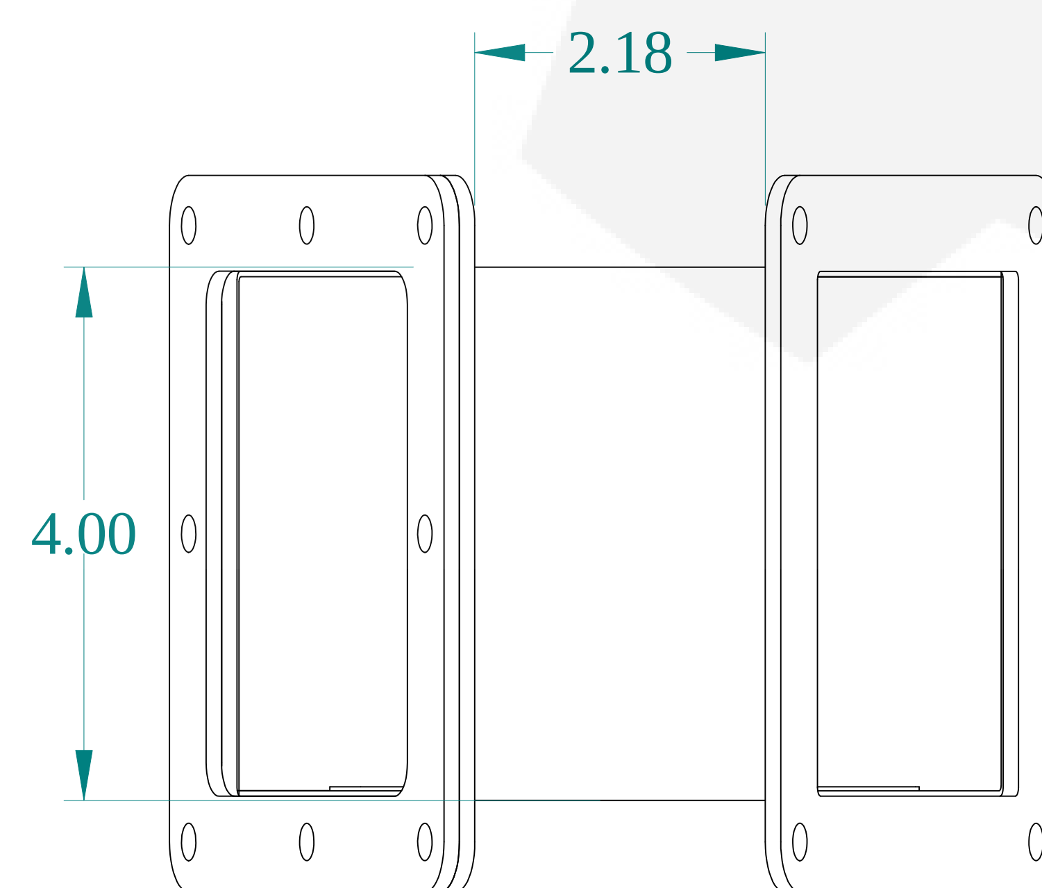
BOTTOM VIEW
