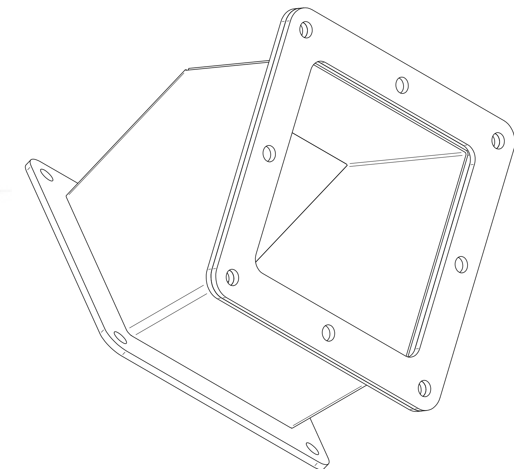
ISOMETRIC VIEWS
