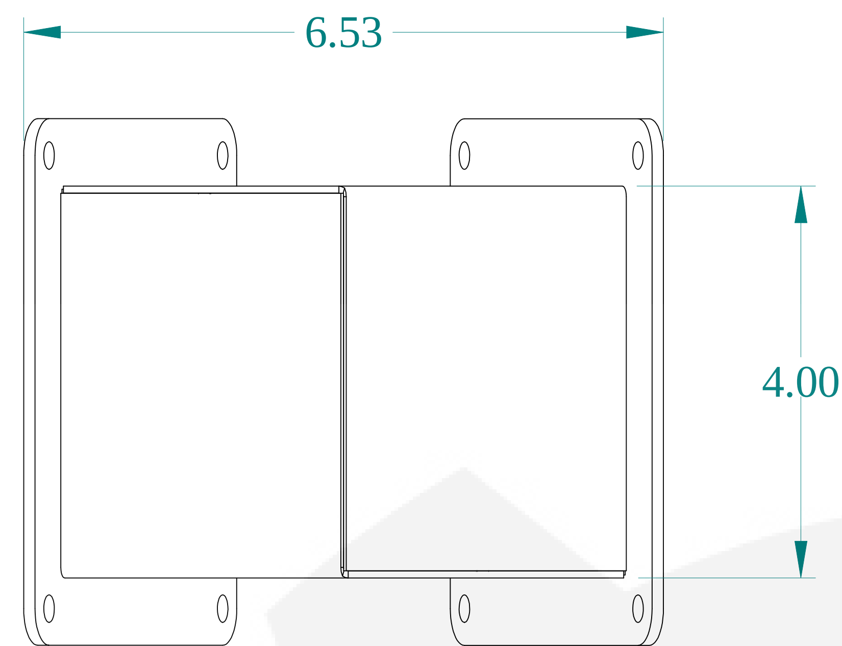
TOP VIEW
