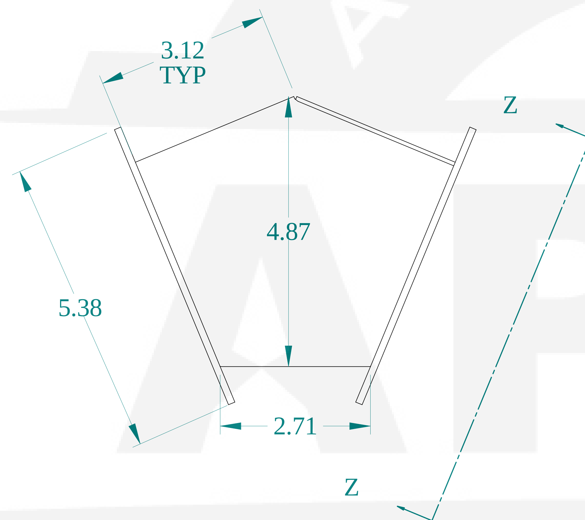
FRONT VIEW
