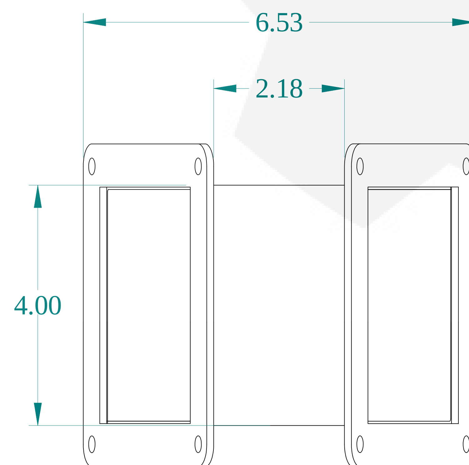
BOTTOM VIEW
