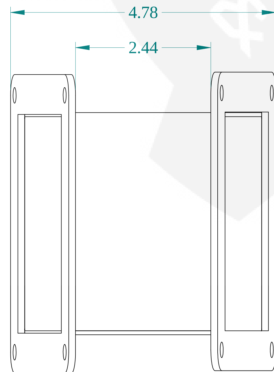
BOTTOM VIEW
