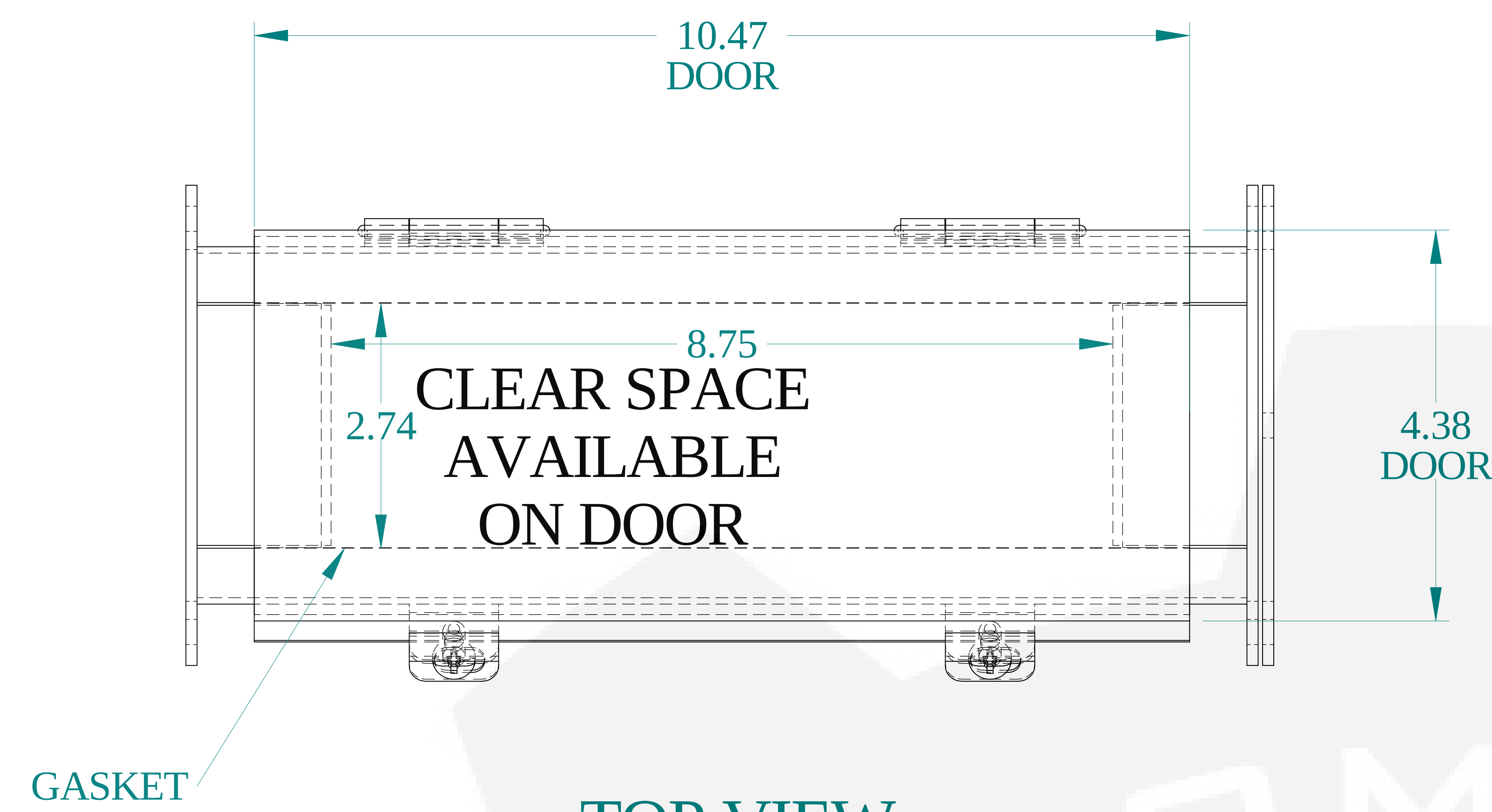
TOP VIEW
