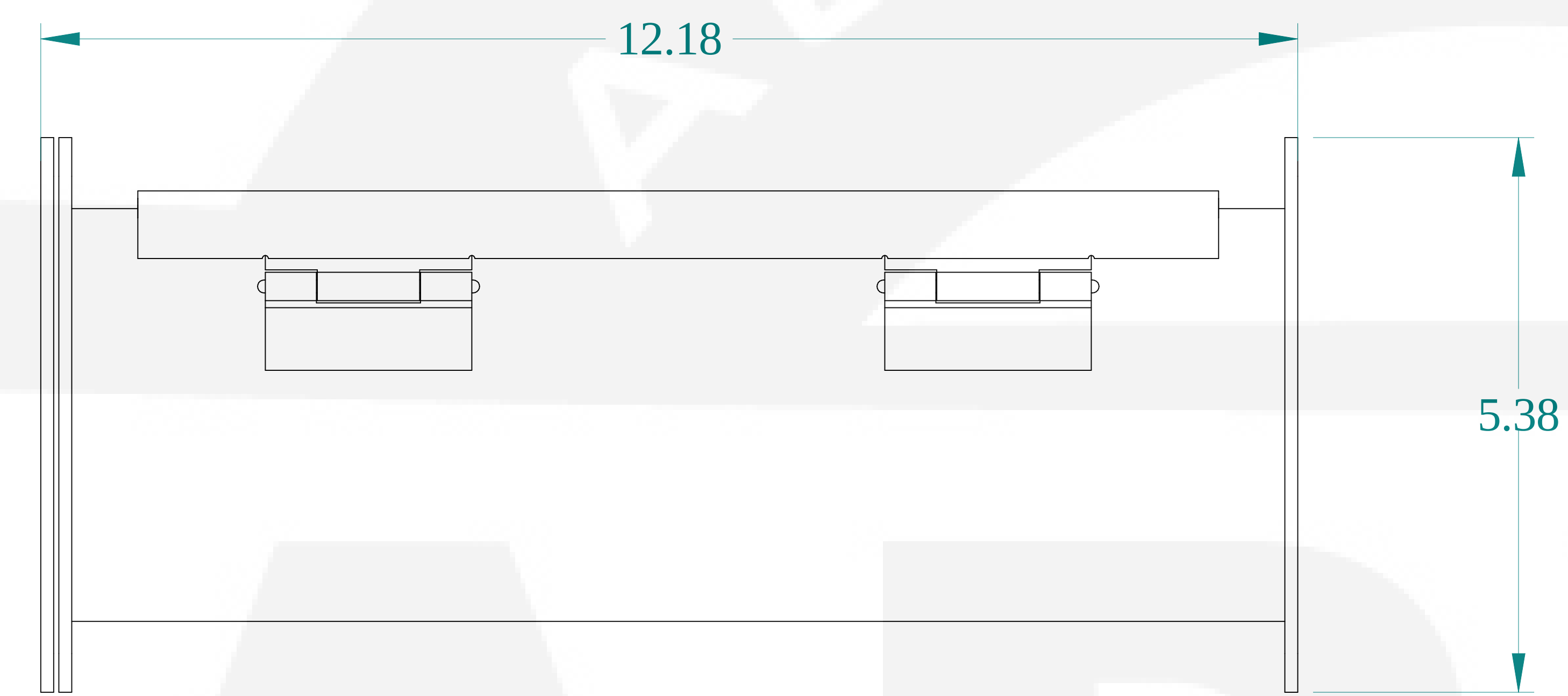
BACK VIEW
