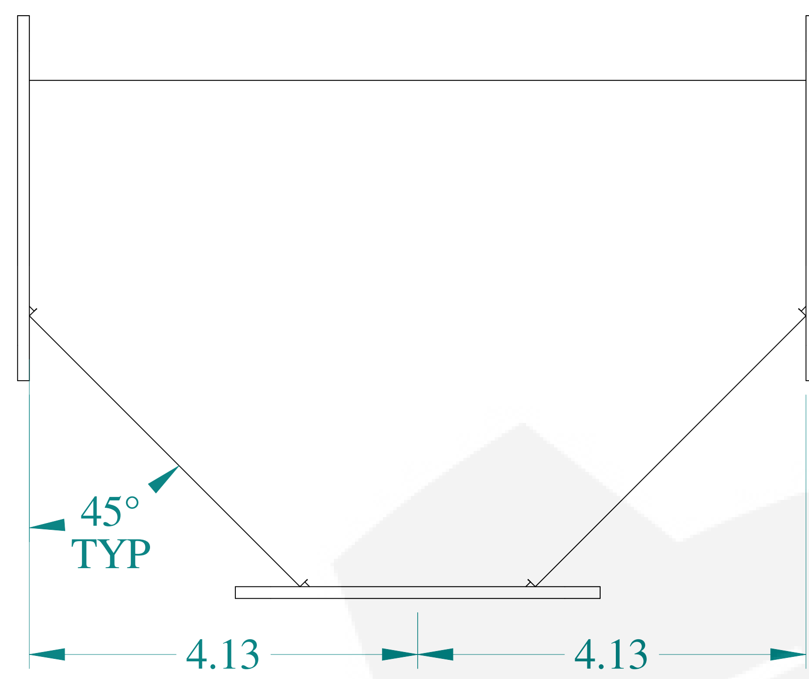
TOP VIEW
