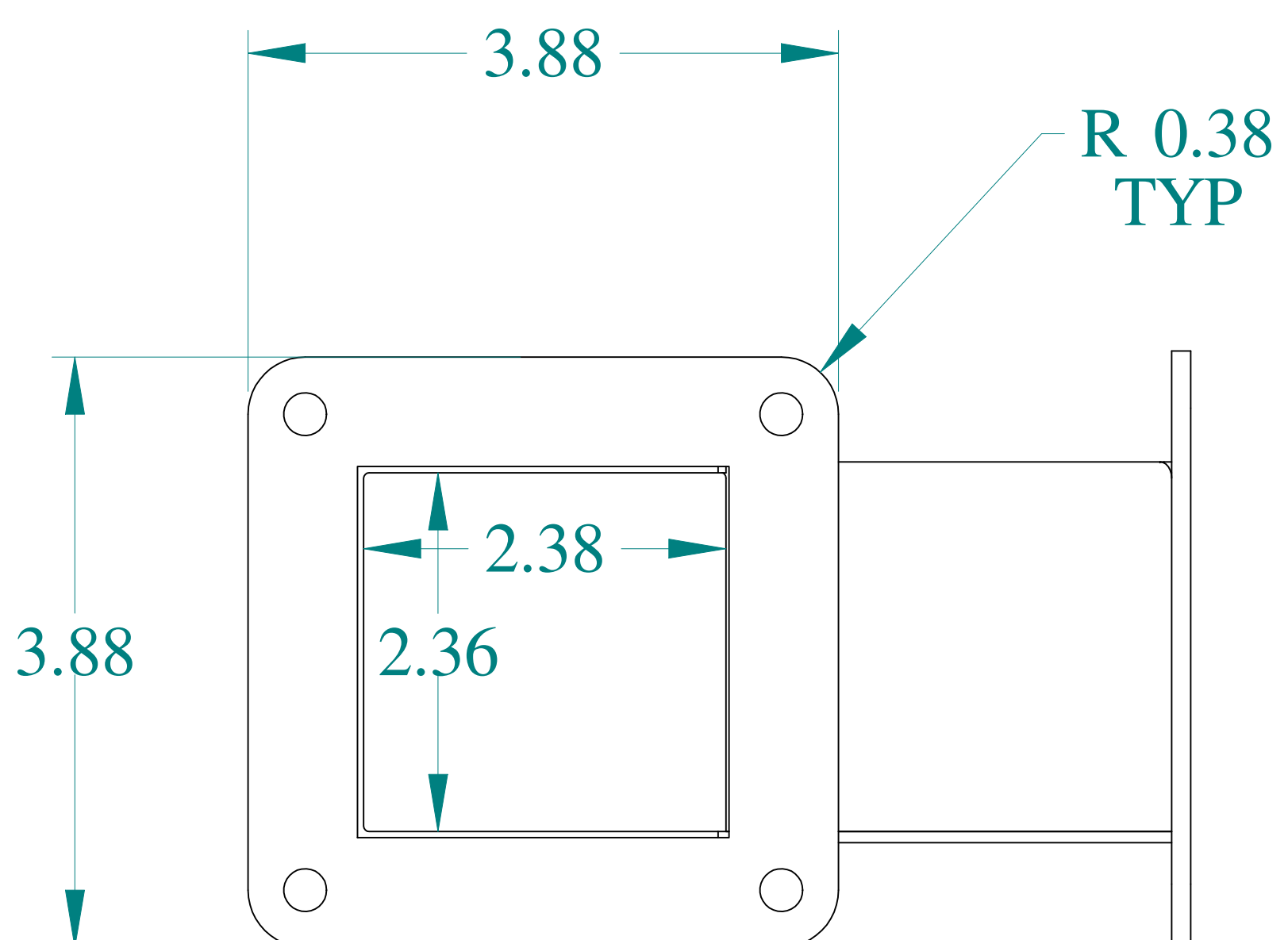
SIDE VIEW
