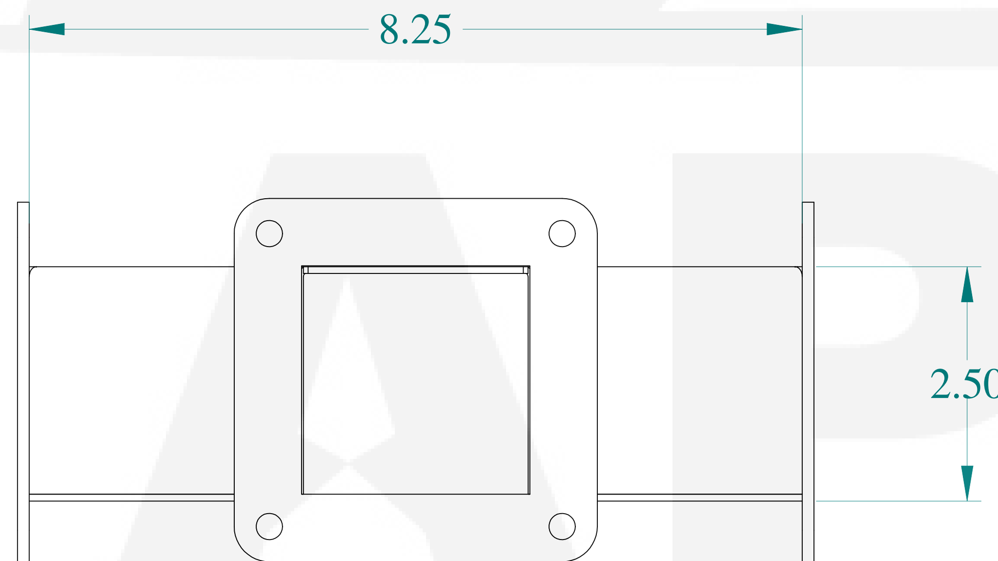
FRONT VIEW
