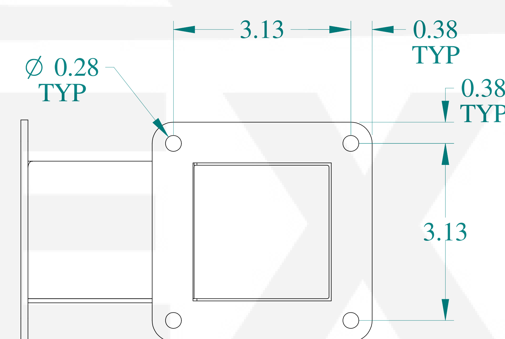
SIDE VIEW
