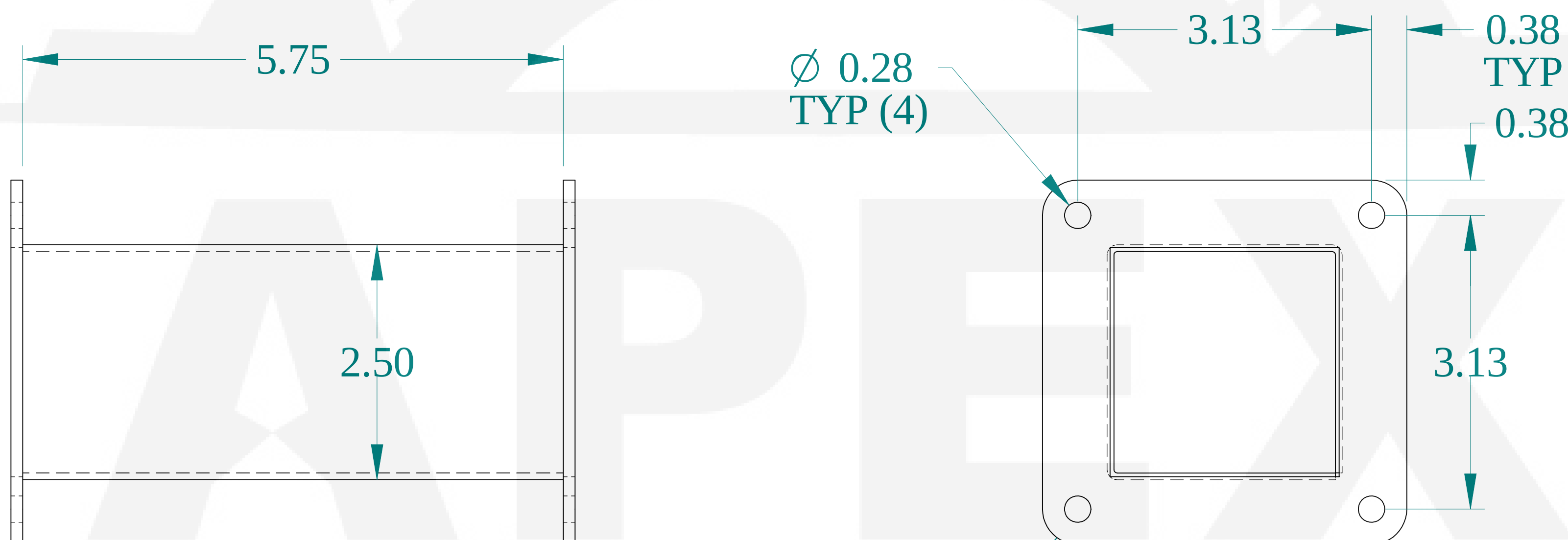
SIDE VIEW
