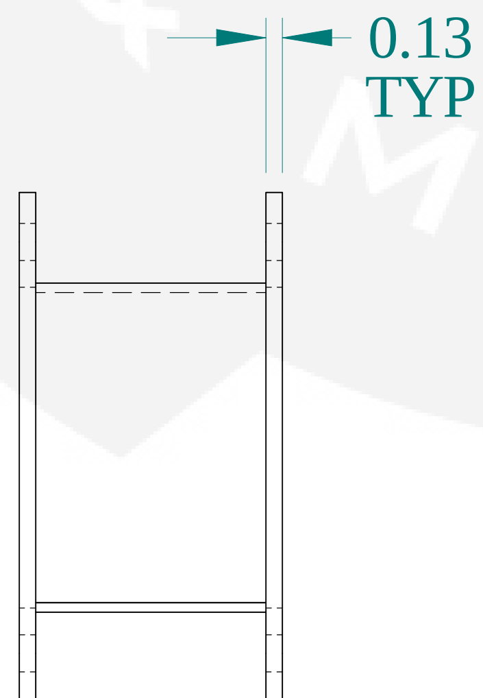
BOTTOM VIEW
