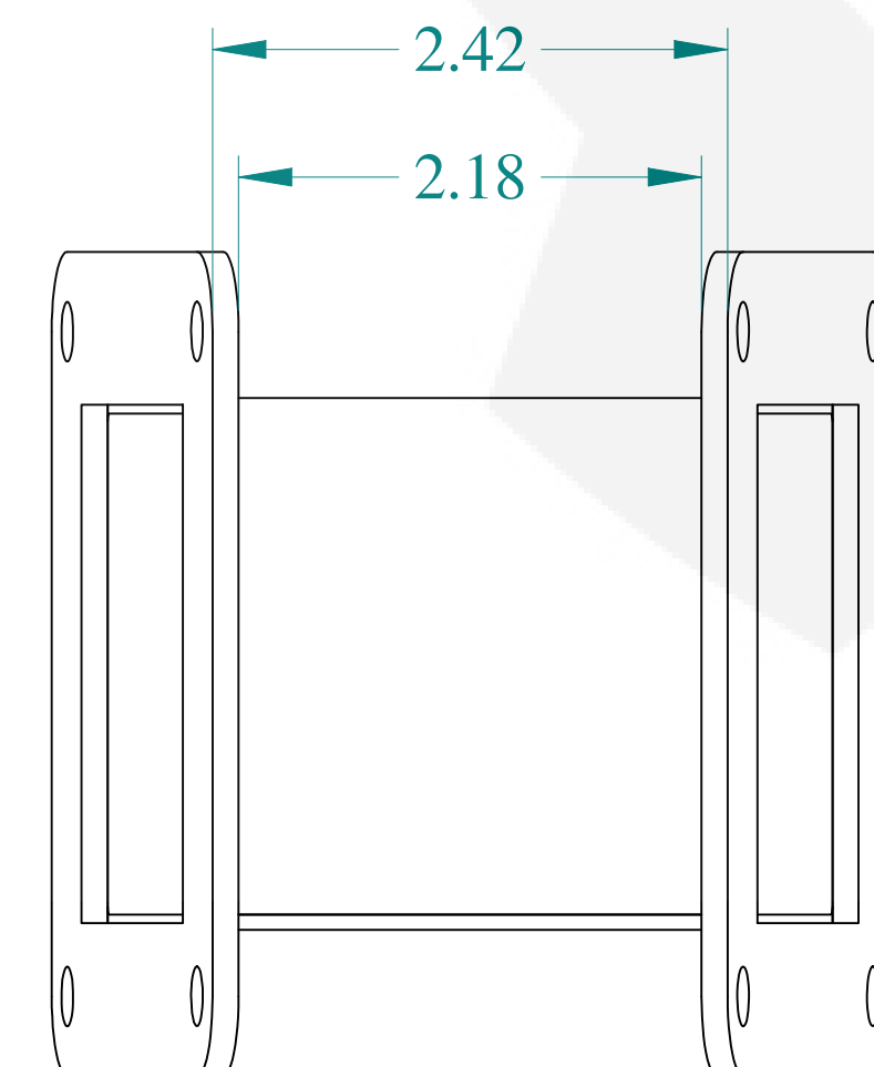
BOTTOM VIEW
