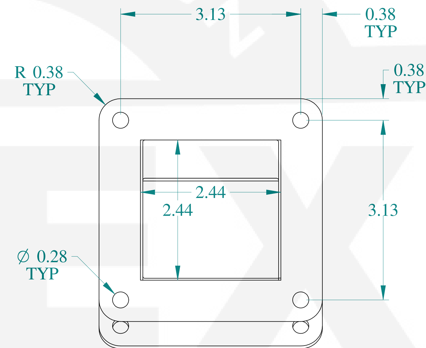
VIEW Z-Z
