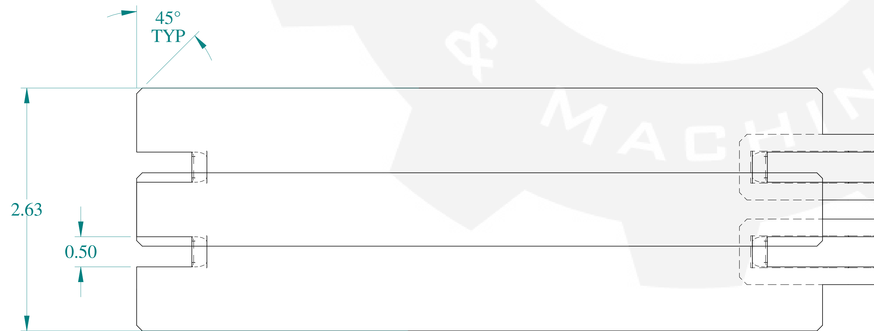
BOTTOM VIEW
