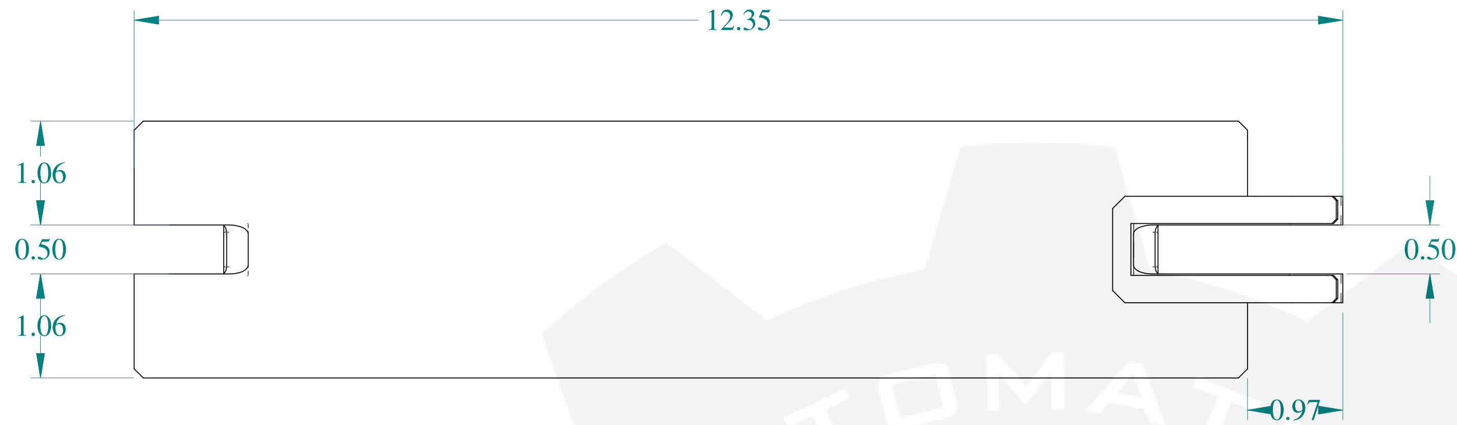
TOP VIEW
